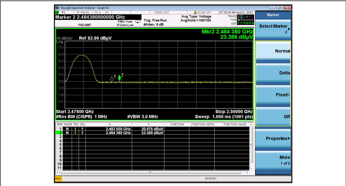
(PEAK, Channel 78, 8-DPSK)
