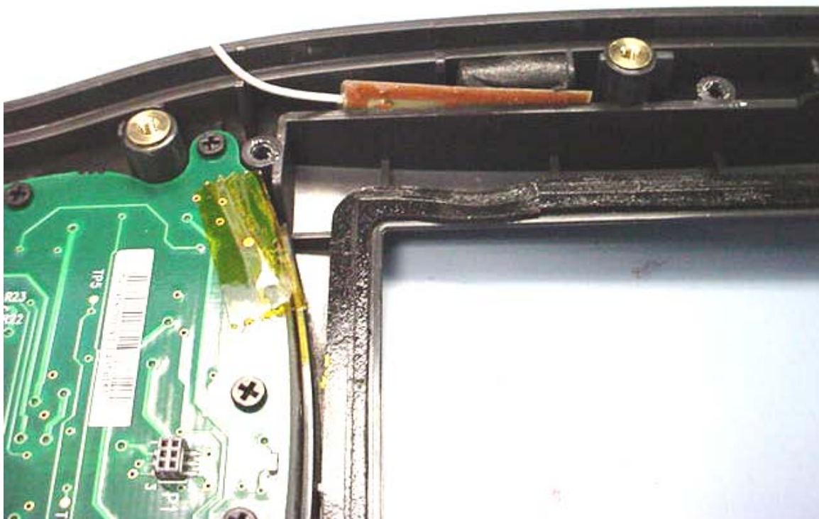
Bluetooth Antenna Location
