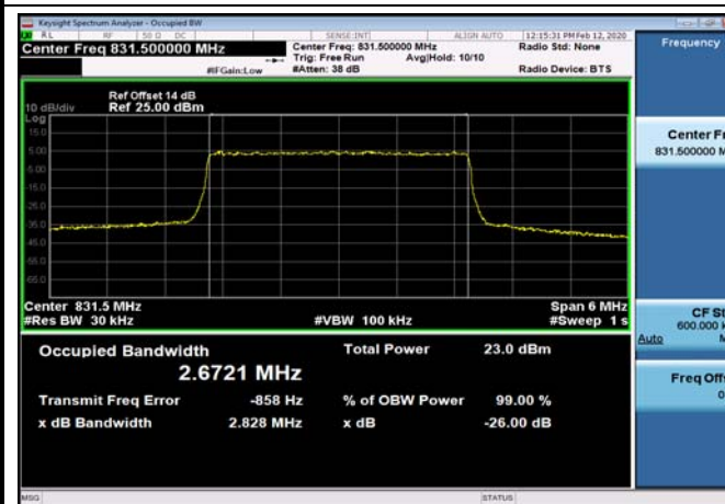
FDD26_MidRange_5_831.5_QPSK
