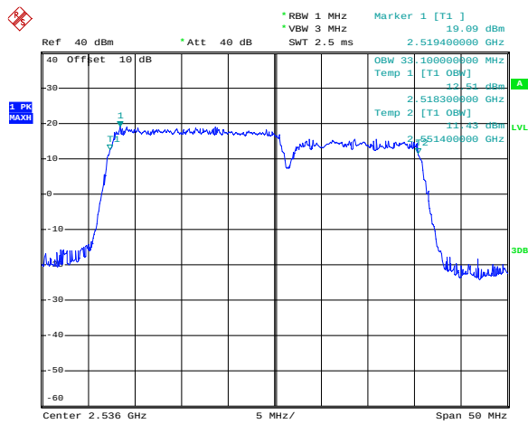
FDD7_MidRange_20+15_QPSK
