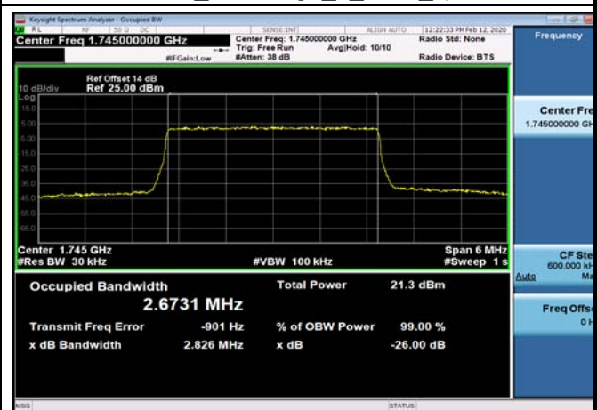
FDD66_MidRange_3_1745_Q16
