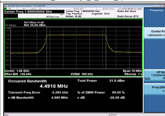
FDD02_MidRange_5_1880_QPSK
