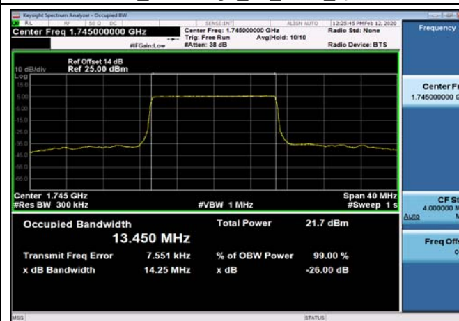
FDD66_MidRange_15_1745_QPSK
