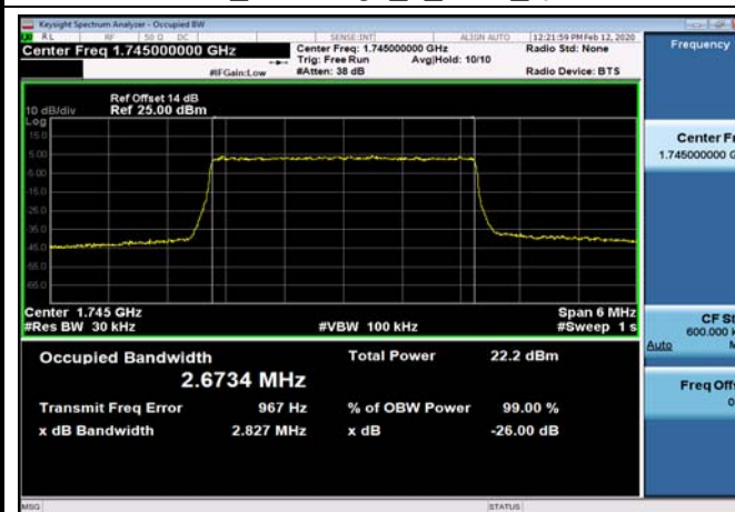
FDD66_MidRange_3_1745_QPSK
