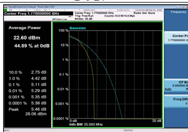
FDD66_HighRange_20MHz_1770_OneRB _high_Q16
