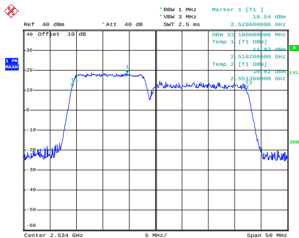
FDD7_MidRange_15+20_QPSK
