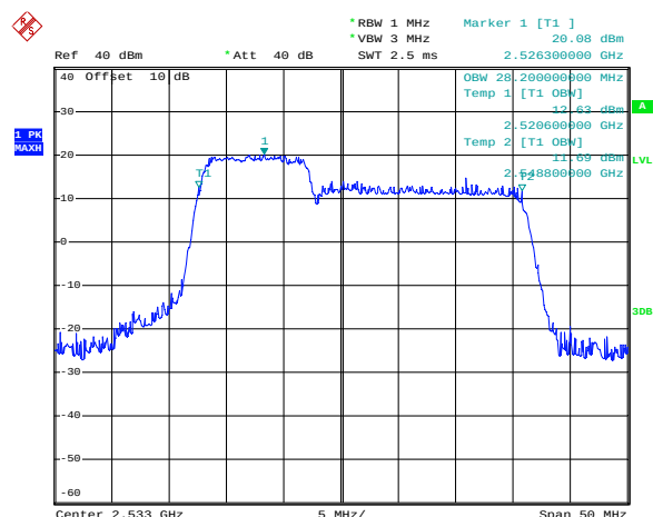
FDD7_MidRange_10+20_Q16
