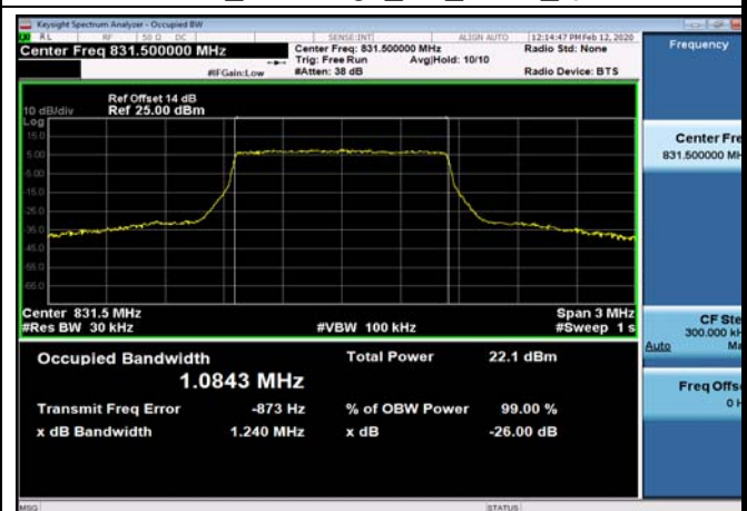
FDD26_MidRange_1.4_831.5_Q16
