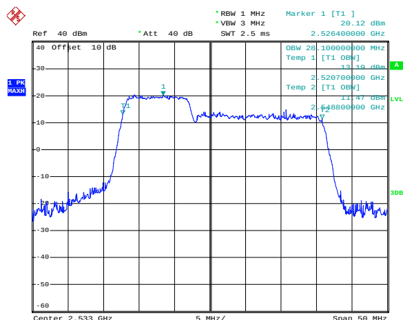
FDD7_MidRange_10+20_QPSK
