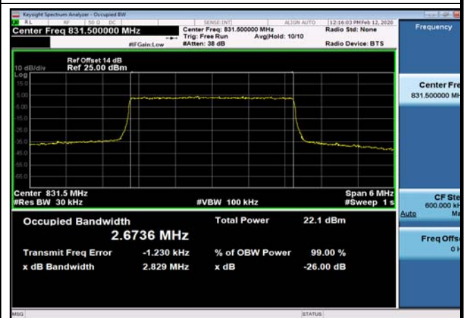
FDD26_MidRange_5_831.5_Q16
