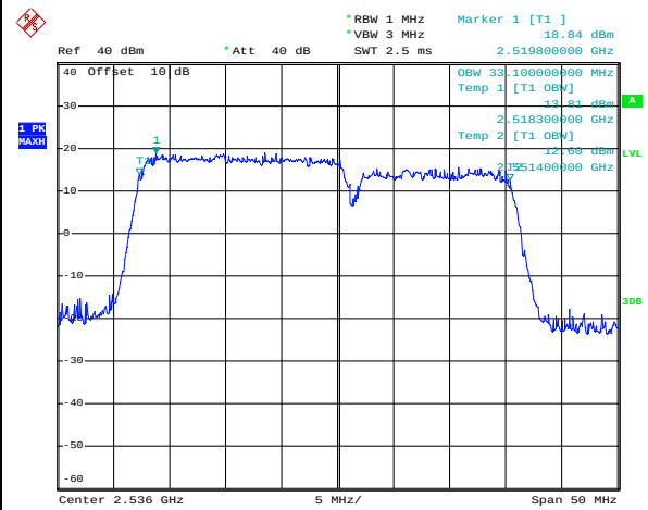
FDD7_MidRange_20+15_Q16
