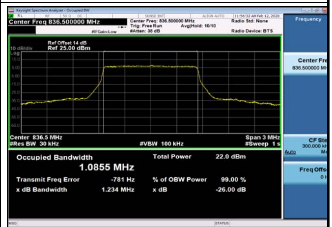
FDD05_MidRange_3_836.5_Q16
