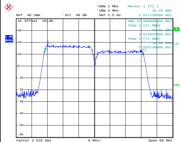
FDD7_MidRange_20+20_Q16
