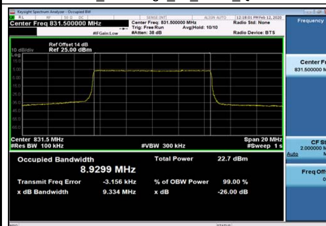
FDD26_MidRange_10_831.5_QPSK
