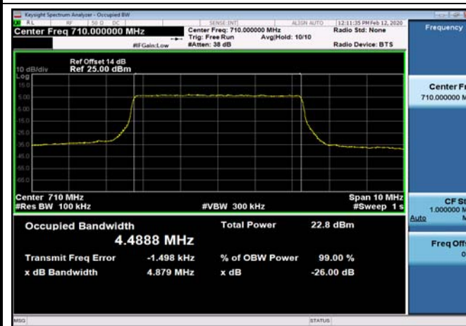
FDD17_MidRange_10_710_QPSK
