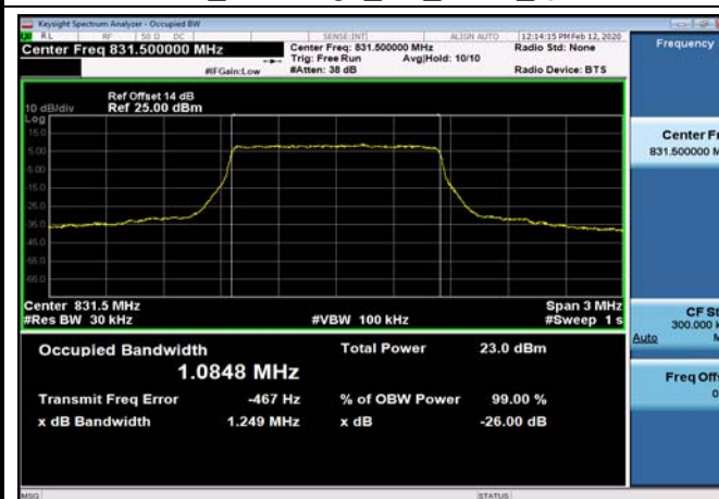
FDD26_MidRange_1.4_831.5_QPSK
