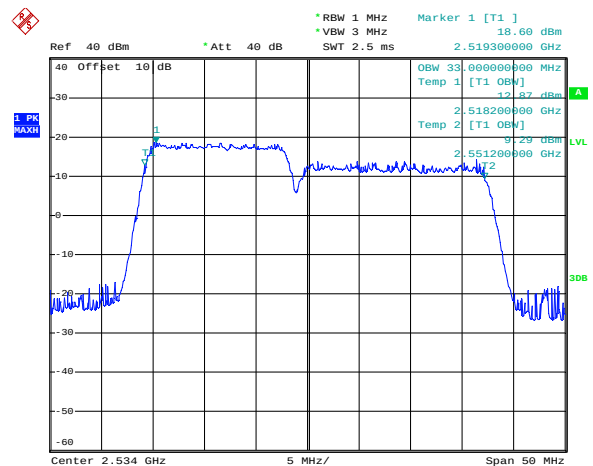
FDD7_MidRange_15+20_Q16
