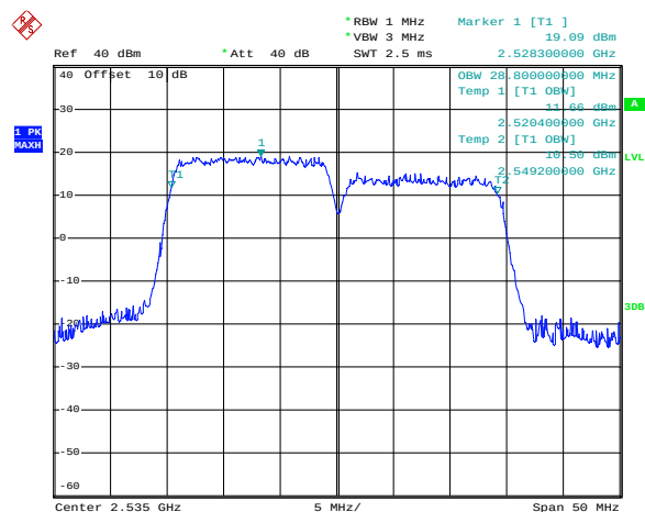
FDD7_MidRange_15+15_Q16
