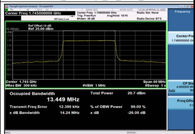
FDD66_MidRange_15_1745_Q16
