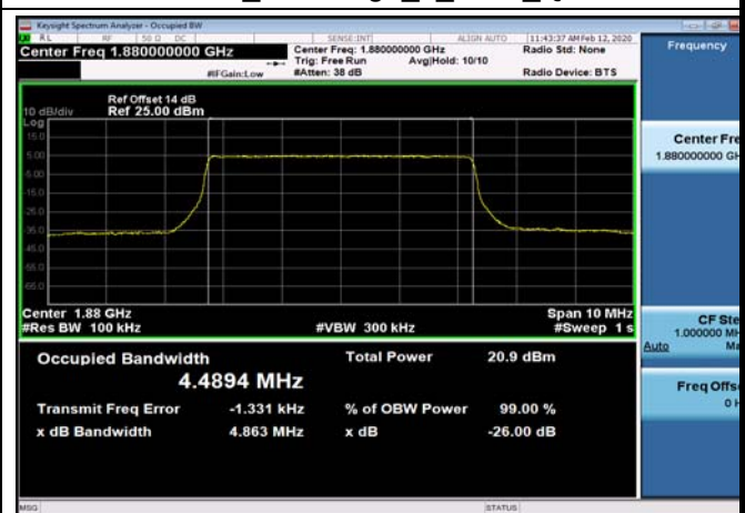
FDD02_MidRange_5_1880_Q16
