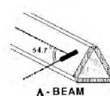
Figure E.2.1 Triangular Probe Configurations
