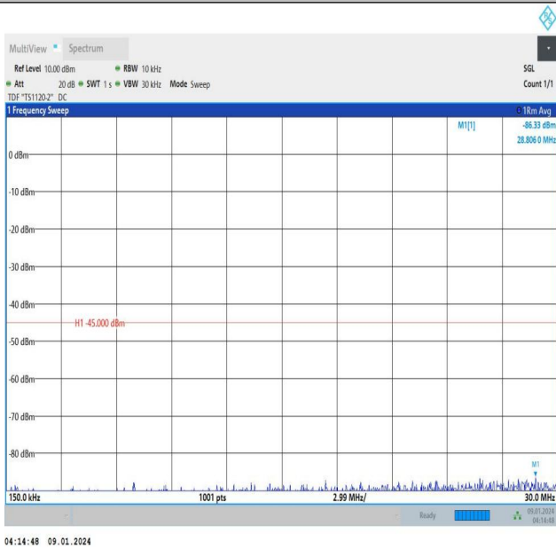
Band38_10MHz_16QAM_38200_1RB#49_0.15~30_0.15~30
