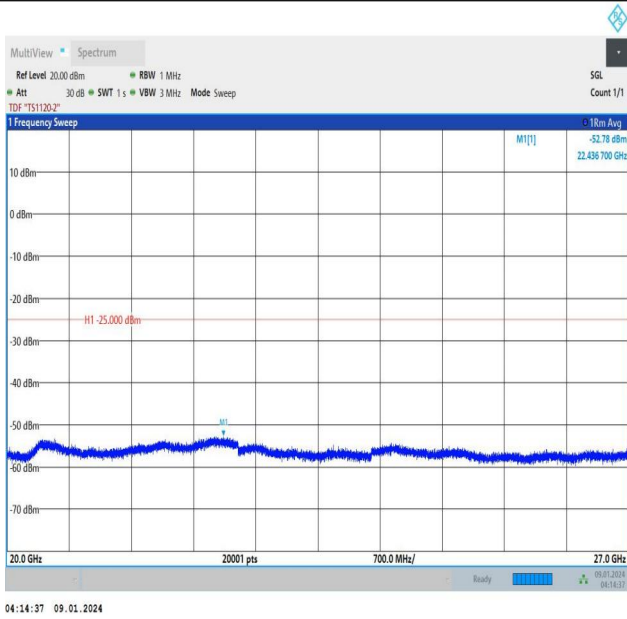
Band38_10MHz_QPSK_38200_1RB#49_20000~27000_2000 0~27000
