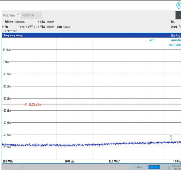
Band38_5MHz_QPSK_38225_1RB#0_30~1000_30~1000
