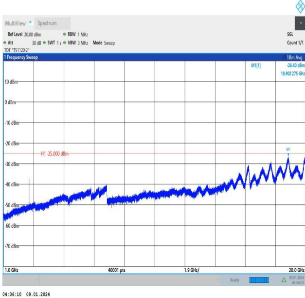
Band38_5MHz_16QAM_38225_1RB#24_1000~20000_1000~20000
