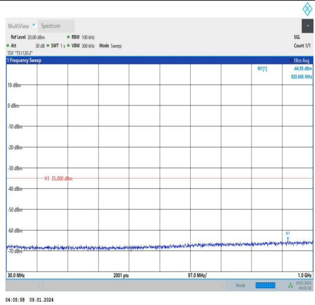
Band38_5MHz_16QAM_38225_1RB#24_30~1000_30~1000
