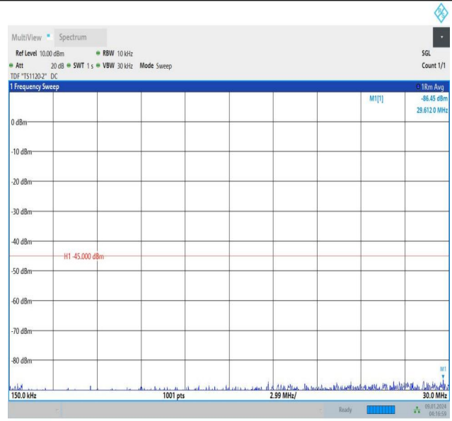
Band38_10MHz_QPSK_38200_50RB#0_0.15~30_0.15~30
