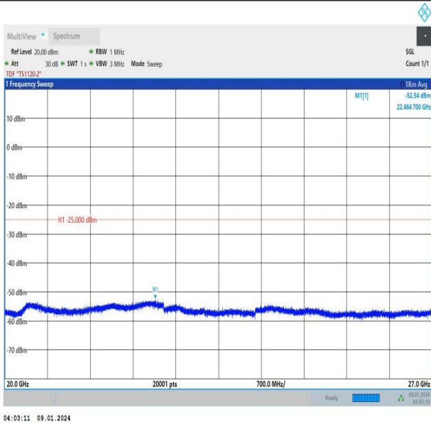
Band38_5MHz_QPSK_38000_25RB#0_20000~27000_20000~27000
