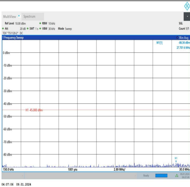
Band38_5MHz_16QAM_38225_25RB#0_0.15~30_0.15~30
