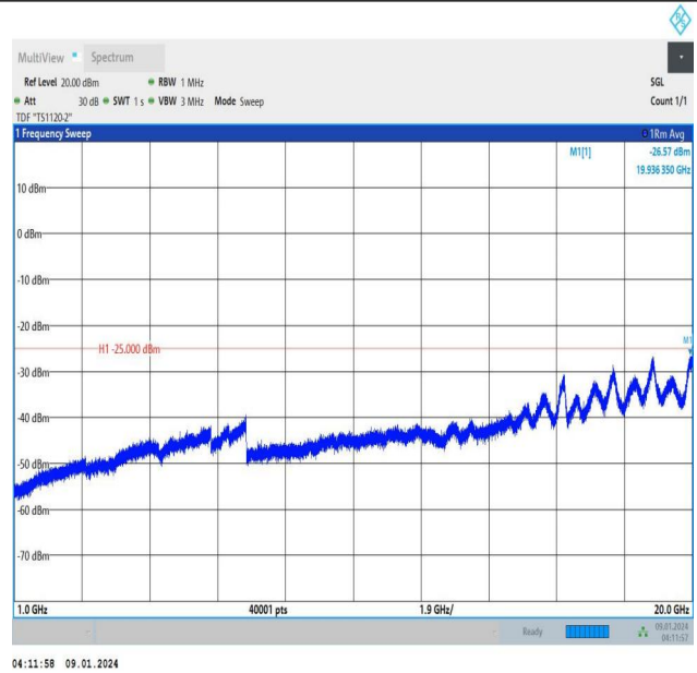
Band38_10MHz_QPSK_38000_1RB#49_1000~20000_1000~20000
