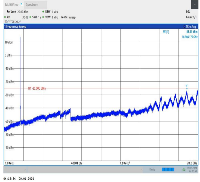
Band38_10MHz_QPSK_37800_50RB#0_1000~20000_1000~20000
