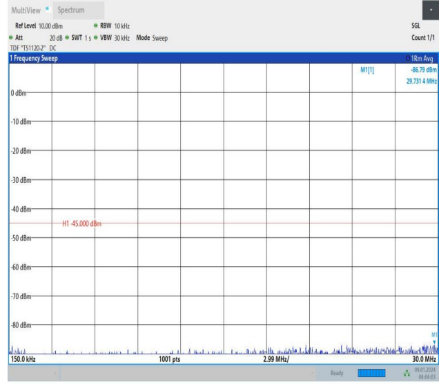
Band38_5MHz_QPSK_38225_1RB#0_0.15~30_0.15~30
