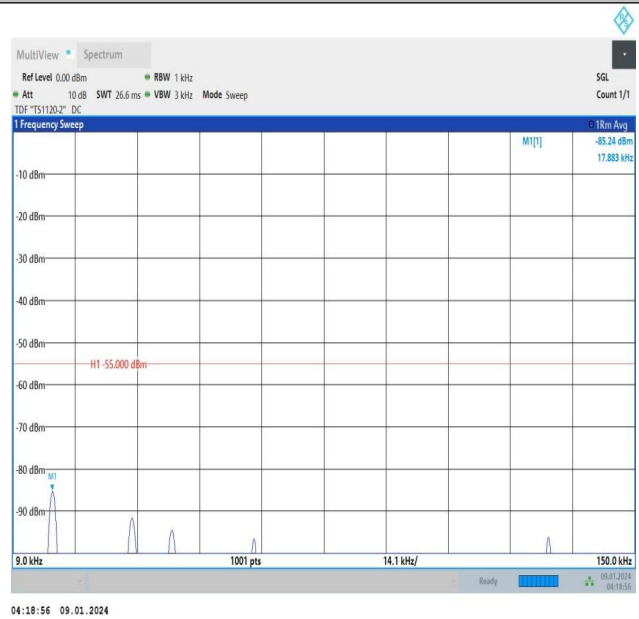
Band38_15MHz_QPSK_37825_1RB#74_0.009~0.15_0.009~0.15
