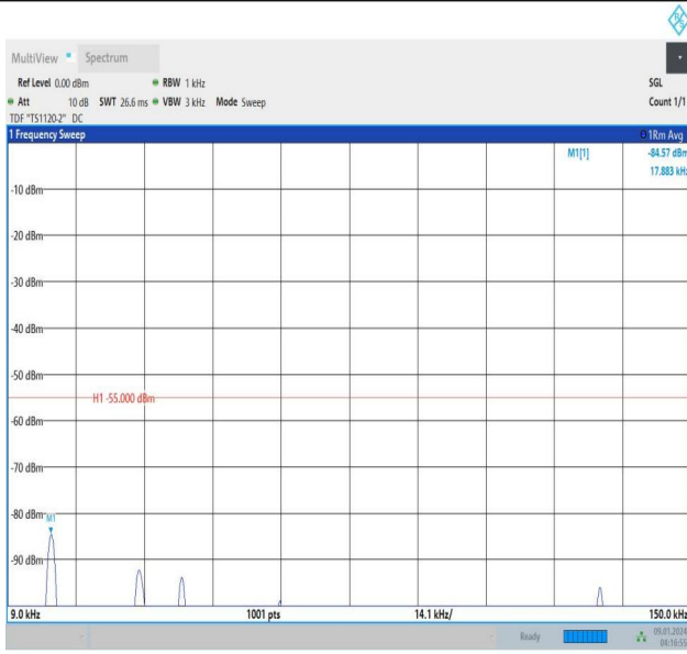
Band38_10MHz_QPSK_38200_50RB#0_0.009~0.15_0.009~0.15
