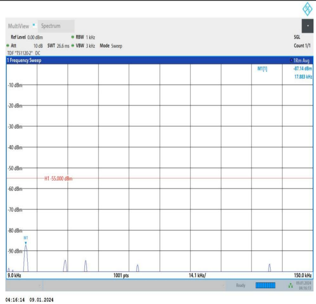
Band38_10MHz_QPSK_38000_50RB#0_0.009~0.15_0.009~0.15
