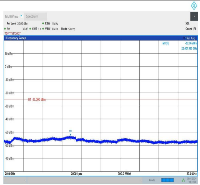
Band38_10MHz_16QAM_37800_1RB#49_20000~27000_20000~27000
