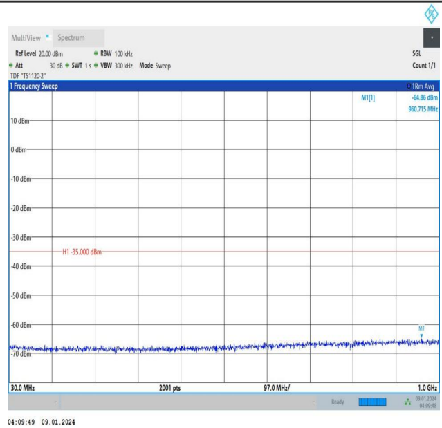
Band38_10MHz_16QAM_37800_1RB#49_30~1000_30~1000
