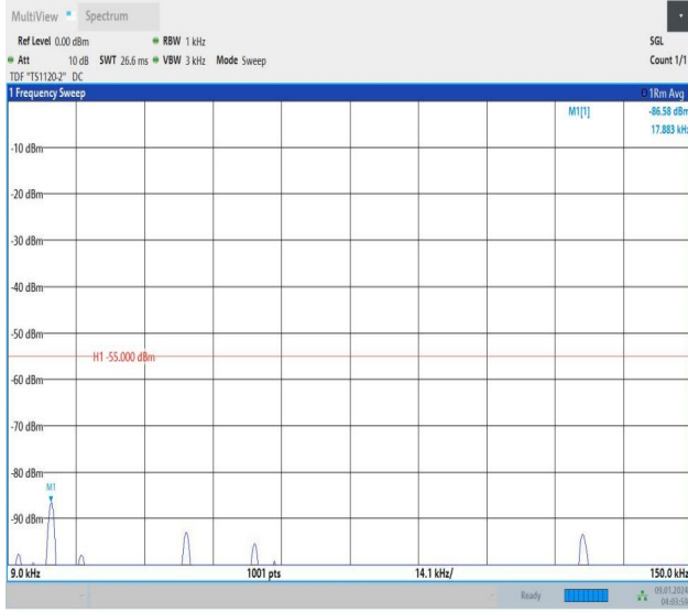
Band38_5MHz_QPSK_38225_1RB#0_0.009~0.15_0.009~0.1
