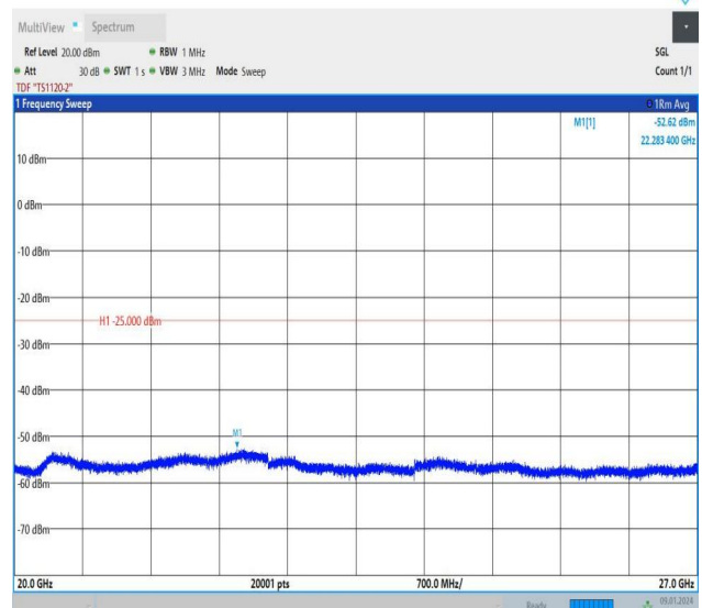
Band38_10MHz_QPSK_38000_50RB#0_20000~27000_20000~27000
