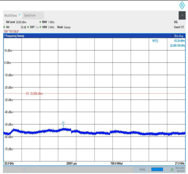
Band38_15MHz_QPSK_37825_1RB#0_20000~27000_20000
