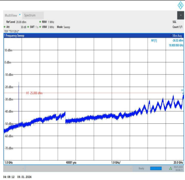
Band38_10MHz_QPSK_37800_1RB#0_1000~20000_1000~20000
