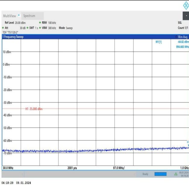
Band38_15MHz_16QAM_37825_1RB#0_30~1000_30~1000
