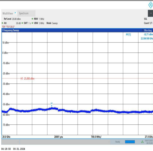
Band38_15MHz_16QAM_37825_1RB#0_20000~27000_20000~27000
