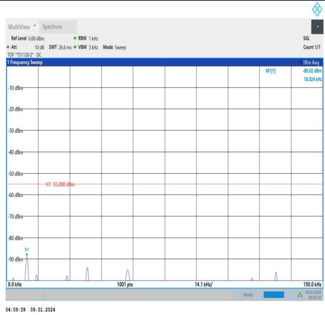
Band38_10MHz_16QAM_37800_1RB#49_0.009~0.15_0.009~ 0.15
