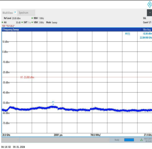
Band38_10MHz_QPSK_37800_50RB#0_20000~27000_20000~27000
