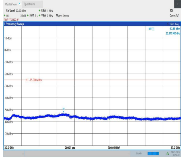
Band38_10MHz_16QAM_38000_1RB#49_20000~27000_20000~27000
