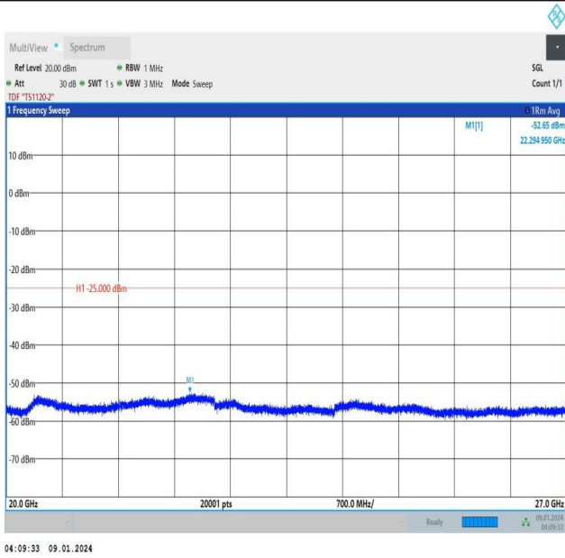
Band38_10MHz_QPSK_37800_1RB#49_20000~27000_2000 0~27000
