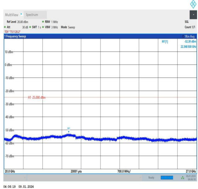
Band38_5MHz_16QAM_38225_1RB#24_20000~27000_20000~27000
