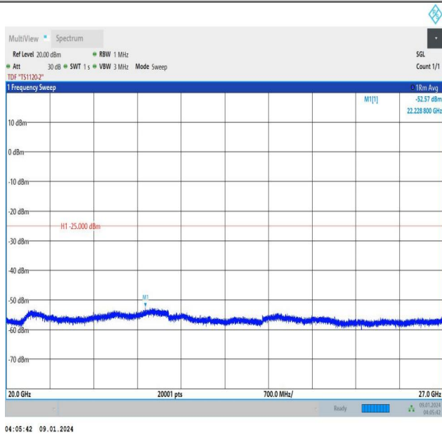
Band38_5MHz_QPSK_38225_1RB#24_20000~27000_20000~27000
