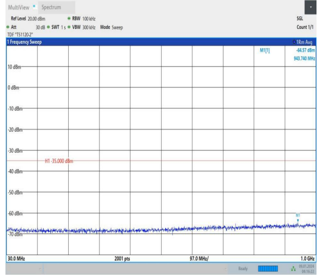
Band38_10MHz_QPSK_38000_50RB#0_30~1000_30~1000
