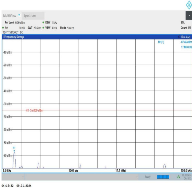
Band38_10MHz_QPSK_37800_50RB#0_0.009~0.15_0.009~0.15
