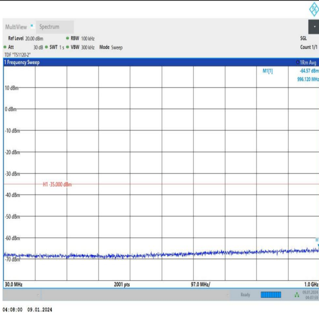
Band38_10MHz_QPSK_37800_1RB#0_30~1000_30~1000
