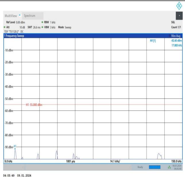
Band38_5MHz_16QAM_38225_1RB#24_0.009~0.15_0.009~0.15
