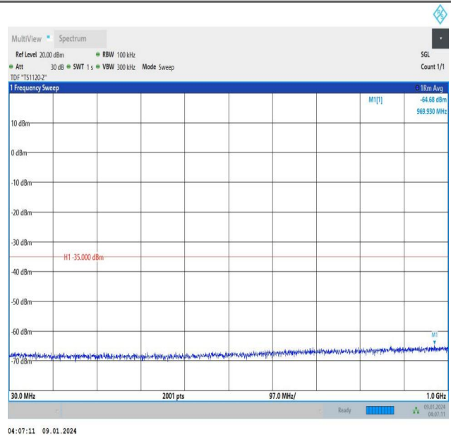
Band38_5MHz_16QAM_38225_25RB#0_30~1000_30~1000
