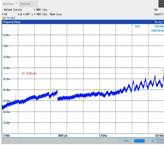
Band38_10MHz_16QAM_38000_1RB#49_1000~20000_1000~20000
