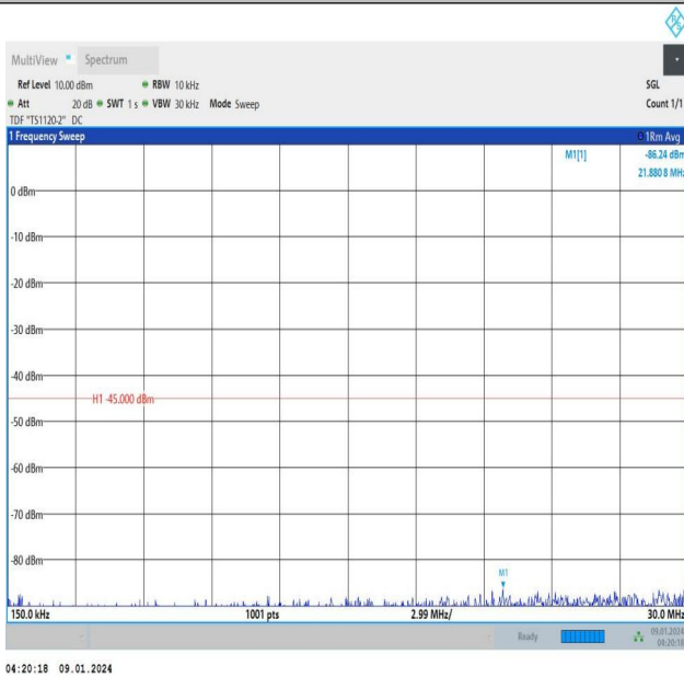
Band38_15MHz_QPSK_38000_1RB#0_0.15~30_0.15~30
