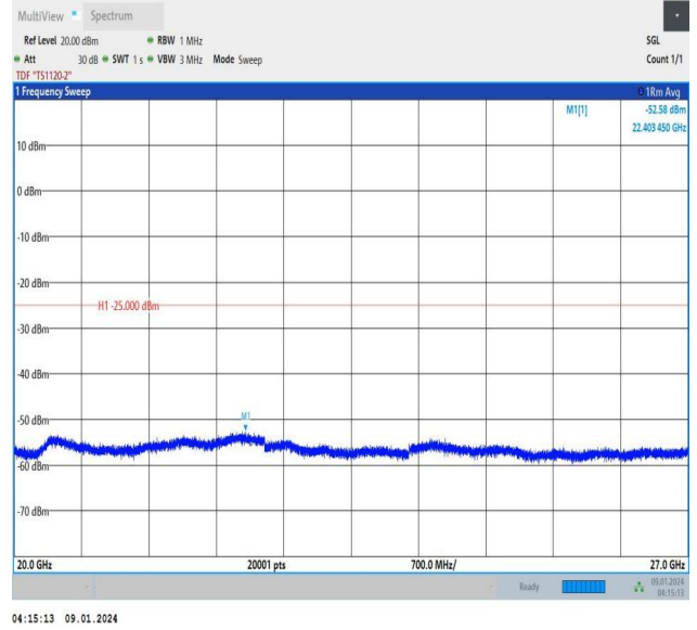
Band38_10MHz_16QAM_38200_1RB#49_20000~27000_20000~27000
