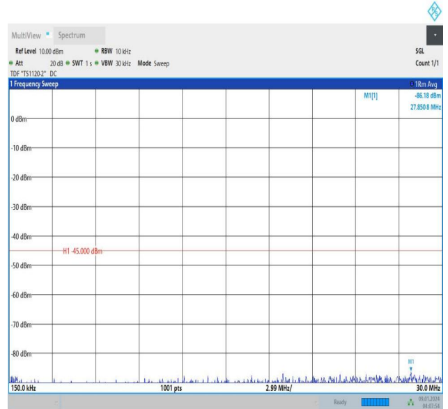
Band38_5MHz_16QAM_38225_25RB#0_20000~27000_20000~27000
