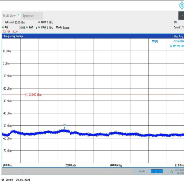
Band38_15MHz_16QAM_37825_1RB#74_20000~27000_20000~27000
