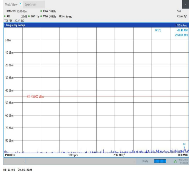
Band38_10MHz_QPSK_38000_1RB#49_0.15~30_0.15~30
