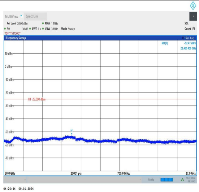
Band38_15MHz_QPSK_38000_1RB#0_20000~27000_20000
