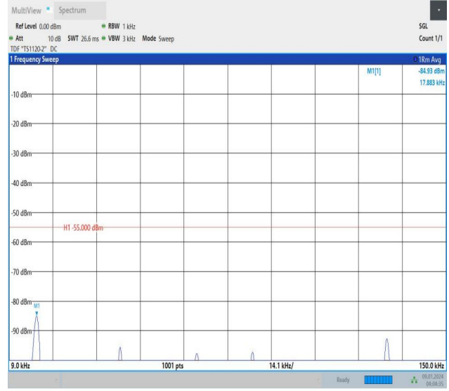
Band38_5MHz_16QAM_38225_1RB#0_0.009~0.15_0.009~0.15
