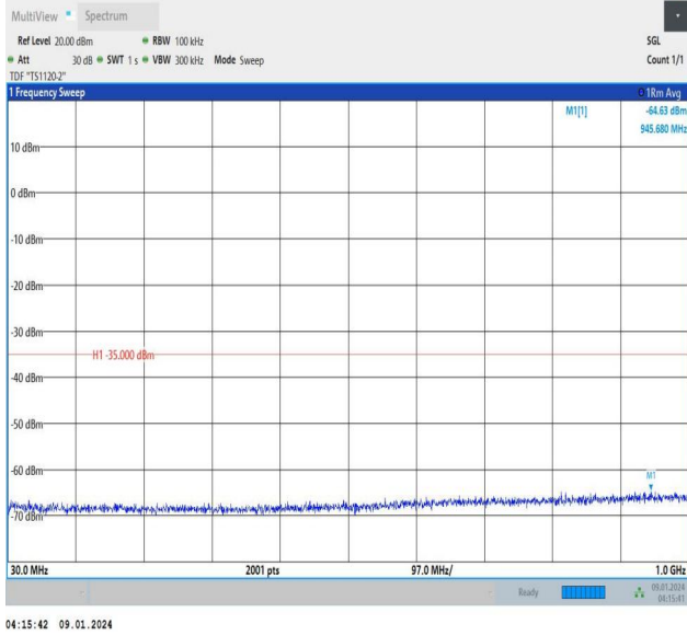
Band38_10MHz_QPSK_37800_50RB#0_30~1000_30~1000
