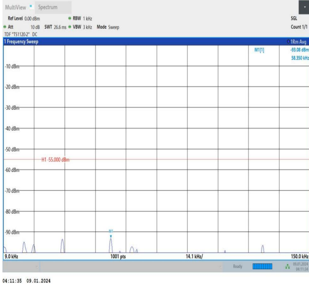
Band38_10MHz_QPSK_38000_1RB#49_0.009~0.15_0.009~0.15
