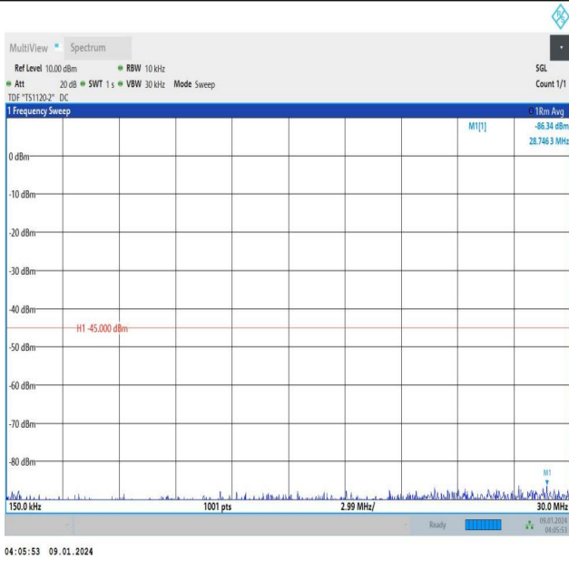
Band38_5MHz_16QAM_38225_1RB#24_0.15~30_0.15~30
