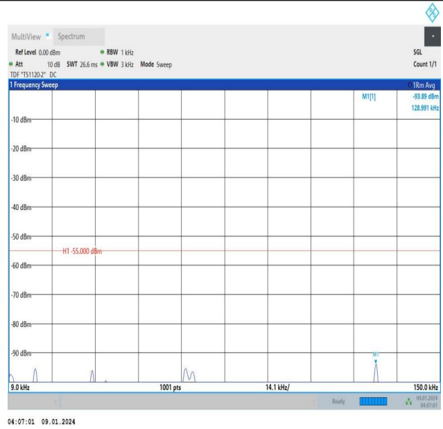
Band38_5MHz_16QAM_38225_25RB#0_0.009~0.15_0.009~0.15
