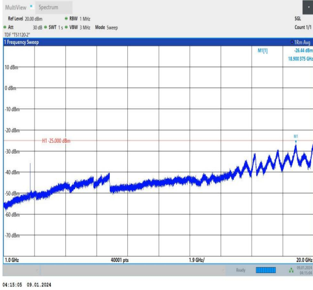
Band38_10MHz_16QAM_38200_1RB#49_1000~20000_1000~20000
