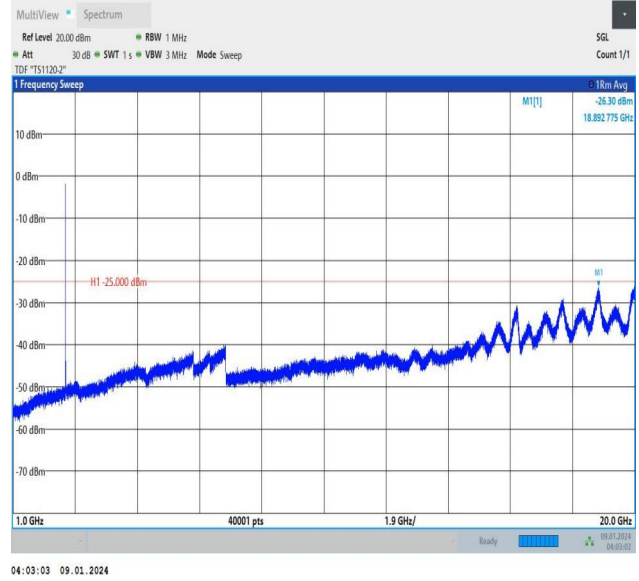
Band38_5MHz_QPSK_38000_25RB#0_1000~20000_1000~20000
