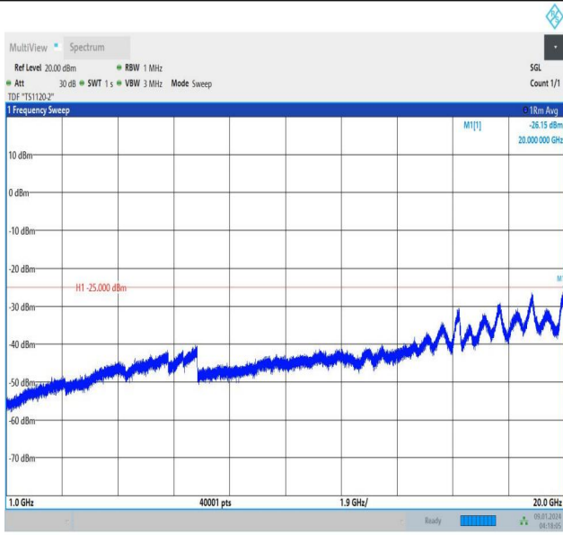
Band38_15MHz_QPSK_37825_1RB#0_1000~20000_1000~20000
