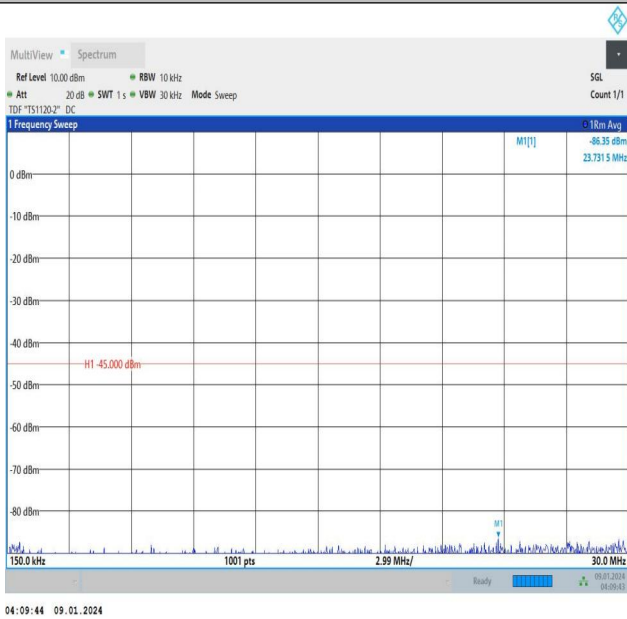
Band38_10MHz_16QAM_37800_1RB#49_0.15~30_0.15~30
