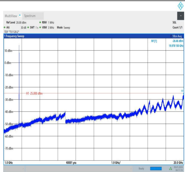
Band38_10MHz_QPSK_38200_50RB#0_1000~20000_1000~20000
