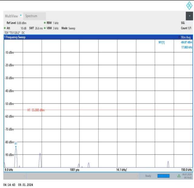
Band38_10MHz_16QAM_38200_1RB#49_0.009~0.15_0.009~ 0.15
