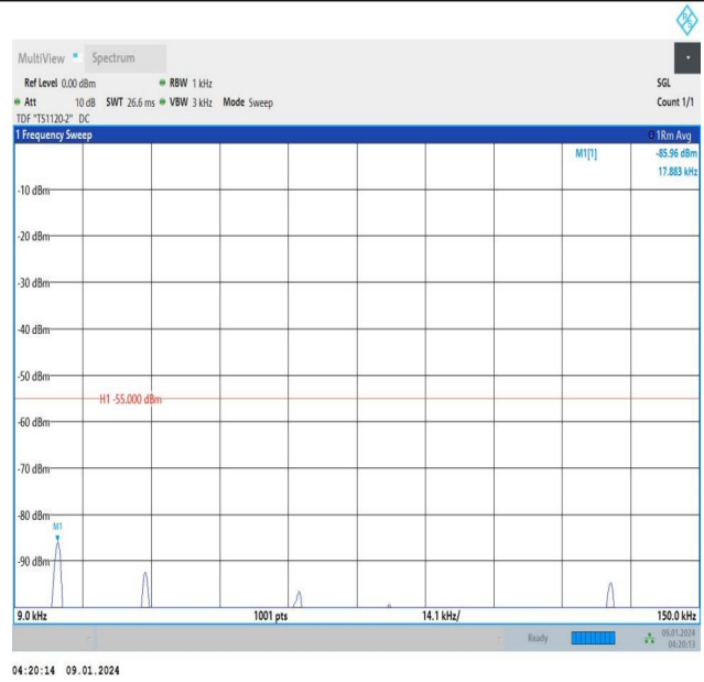
Band38_15MHz_QPSK_38000_1RB#0_0.009~0.15_0.009~0.15
