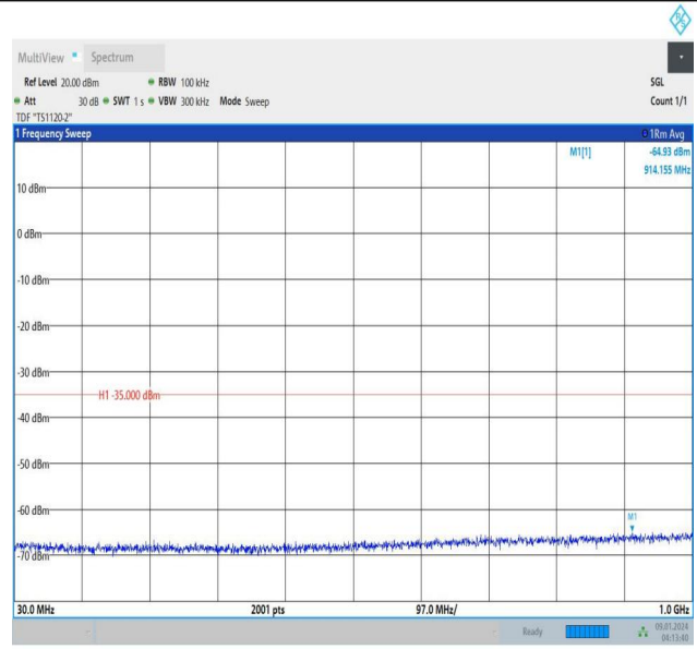
Band38_10MHz_16QAM_38200_1RB#0_30~1000_30~1000
