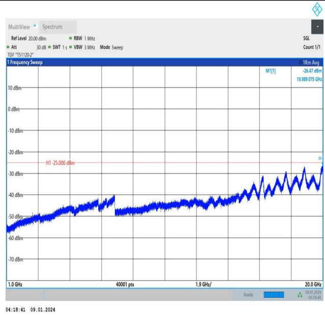
Band38_15MHz_16QAM_37825_1RB#0_1000~20000_1000~20000
