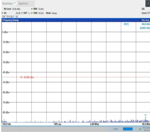
Band38_10MHz_QPSK_38000_50RB#0_0.15~30_0.15~30
