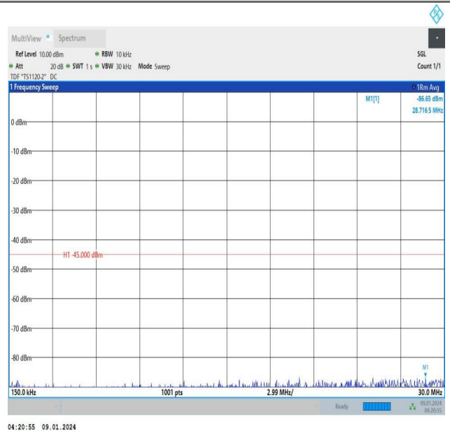
Band38_15MHz_16QAM_38000_1RB#0_0.15~30_0.15~30
