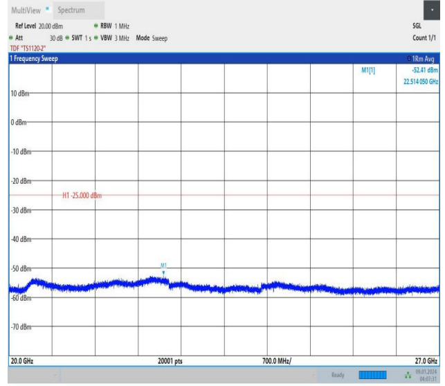
Band38_5MHz_16QAM_38225_25RB#0_20000~27000_20000~27000
