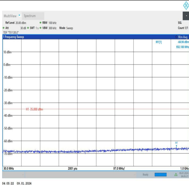
Band38_5MHz_QPSK_38225_1RB#24_30~1000_30~1000
