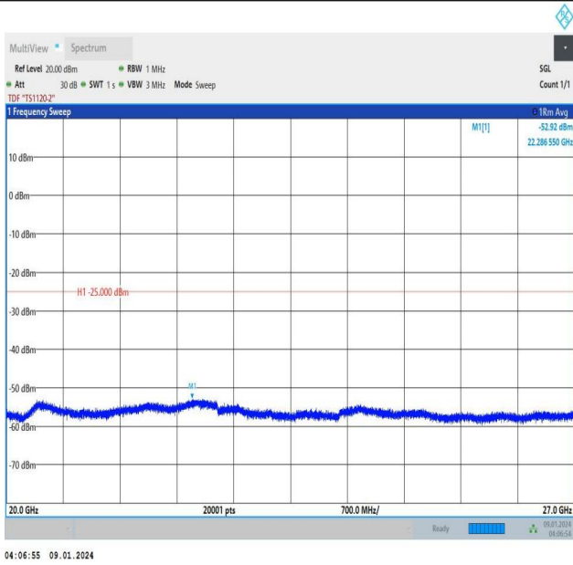
Band38_5MHz_QPSK_38225_25RB#0_20000~27000_20000~27000
