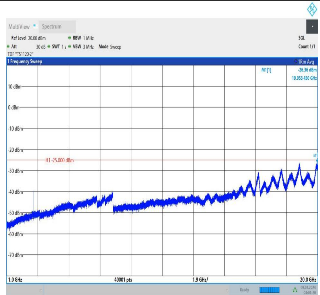
Band38_5MHz_QPSK_38225_1RB#0_1000~20000_1000~20000
