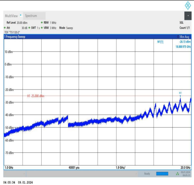
Band38_5MHz_QPSK_38225_1RB#24_1000~20000_1000~20000
