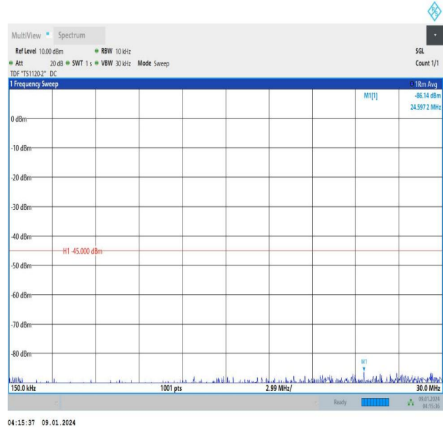
Band38_10MHz_QPSK_37800_50RB#0_0.15~30_0.15~30
