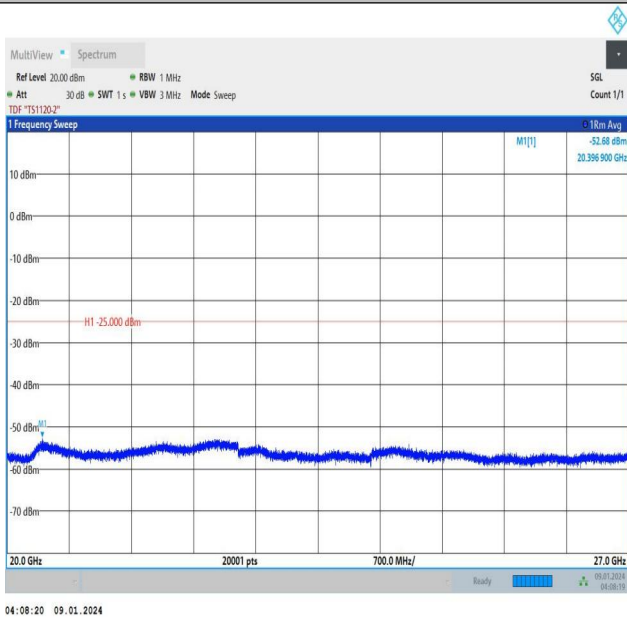
Band38_10MHz_QPSK_37800_1RB#0_20000~27000_20000~27000
