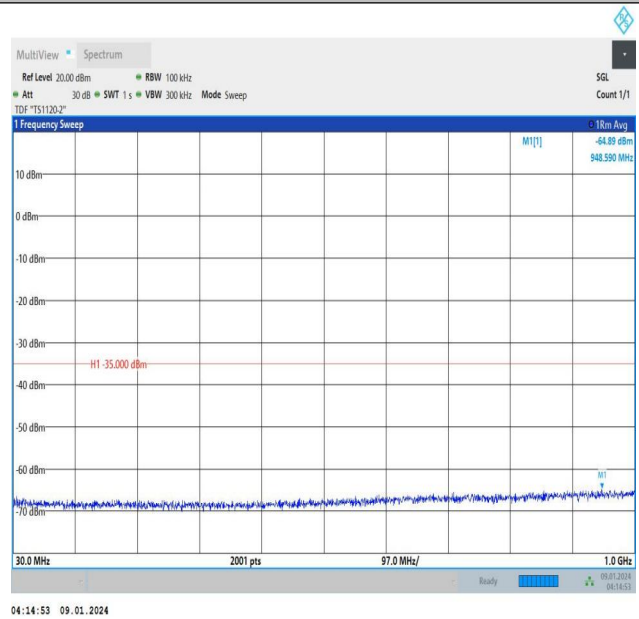
Band38_10MHz_16QAM_38200_1RB#49_30~1000_30~1000
