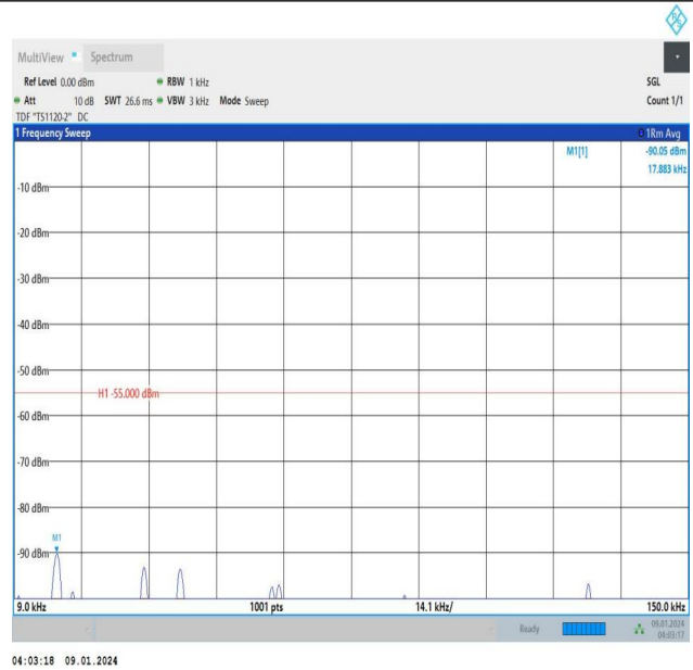
Band38_5MHz_16QAM_38000_25RB#0_0.009~0.15_0.009~0.15
