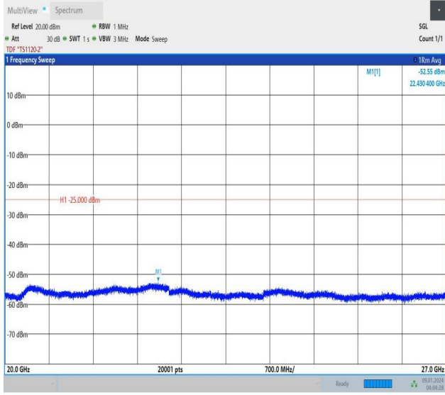
Band38_5MHz_QPSK_38225_1RB#0_20000~27000_20000~27000
