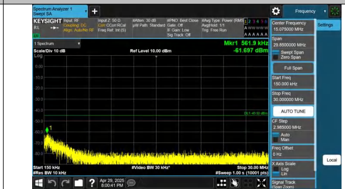
Band7-10MHz-QPSK-21400-1RB#0-0.15~30-PASS
