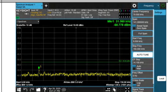
Band7-10MHz-QPSK-21400-1RB#49-0.009~0.15-PASS
