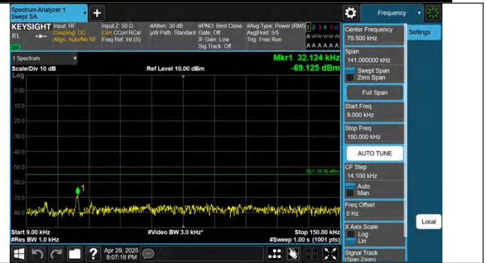
Band7-15MHz-QPSK-20825-1RB#74-0.009~0.15-PASS
