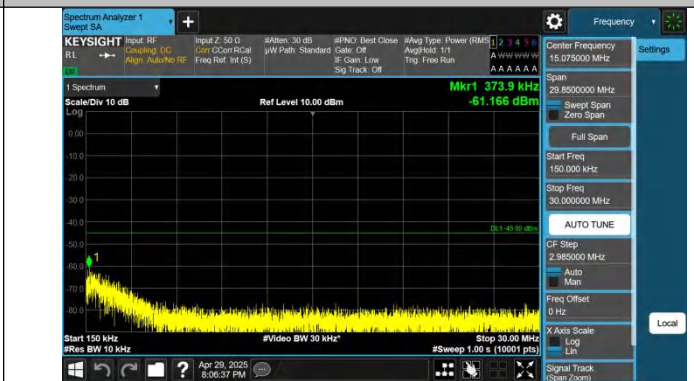
Band7-15MHz-QPSK-20825-1RB#0-0.15~30-PASS
