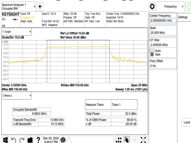
Band41_10MHz_64QAM_RB50_0_CH39740
