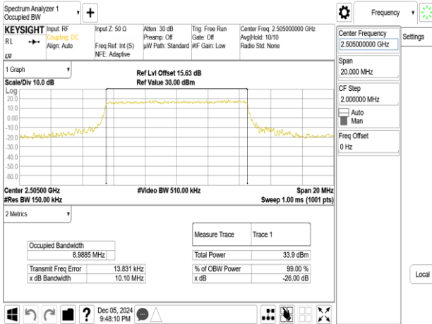
Band41_10MHz_16QAM_RB50_0_CH39740
