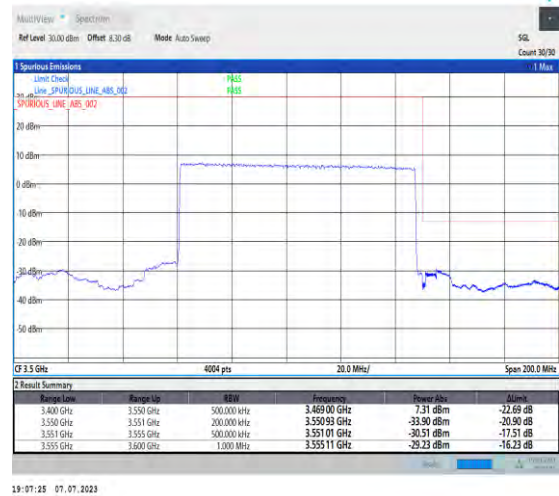
1-N77-3450-3550-PC1.5-30-90-H-3-DFT-PI2BPSK-Outer_Full-240@0-Ant3-1--PASS-see graph
