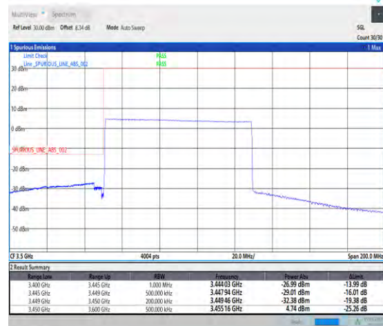
1-N77-3450-3550-PC1.5-30-80-L-6-CP-QPSK-Outer_Full-217@0-Ant3-1--PASS-see graph
