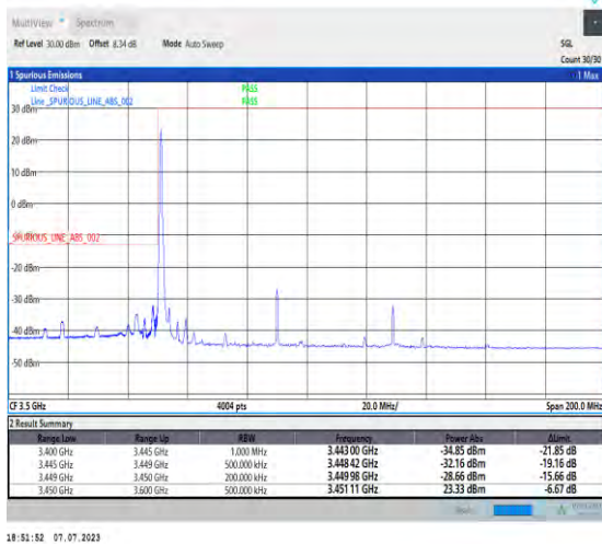
1-N77-3450-3550-PC1.5-30-80-L-4-CP-QPSK-Edge_1RB_Left-1@0-Ant3-1--PASS-see graph
