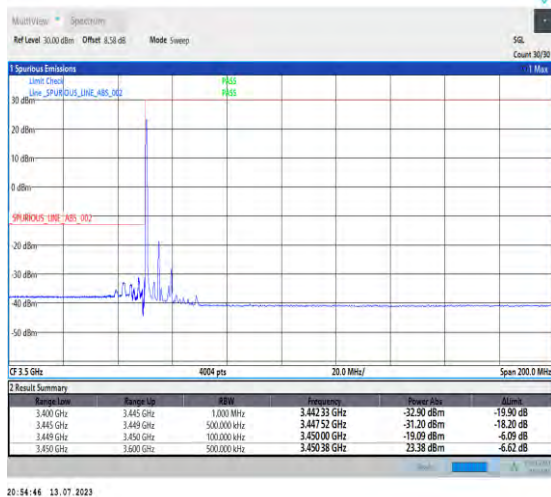
1-N77-3450-3550-PC1.5-30-10-L-4-CP-QPSK-Edge_1RB_Left-1@0-Ant3-1--PASS-see graph
