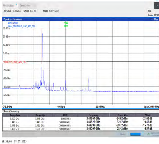
1-N77-3450-3550-PC1.5-30-60-L-1-DFT-PI2BPSK-Edge_1RB_Left-1@0-Ant3-1--PASS-see graph
