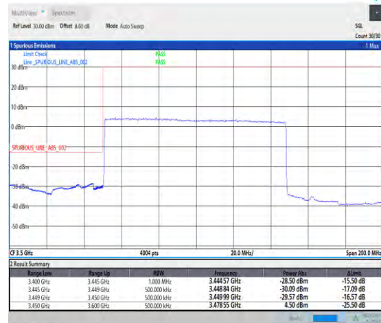
1-N77-3450-3550-PC1.5-30-100-L-3-DFT-PI2BPSK -Outer_Full-270@0-Ant3-1--PASS-see graph
