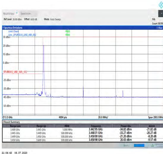
1-N77-3450-3550-PC1.5-30-100-L-4-CP-QPSK-Edge _1RB_Left-1@0-Ant3-1--PASS-see graph
