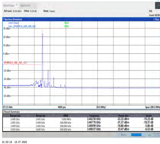
1-N77-3450-3550-PC1.5-30-15-L-1-DFT-PI2BPSK-Edge_1RB_Left-1@0-Ant3-1--PASS-see graph
