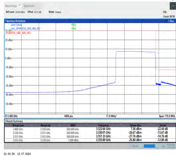
1-N77-3450-3550-PC1.5-30-40-H-3-DFT-PI2BPSK-Out_Full-100@0-Ant3-1--PASS-see graph
