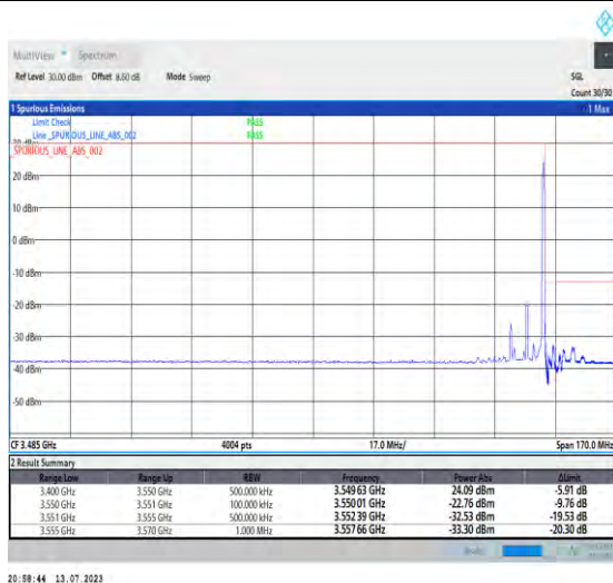
1-N77-3450-3550-PC1.5-30-10-H-5-CP-QPSK-Edge_1RB_Right-1@23-Ant3-1--PASS-see graph
