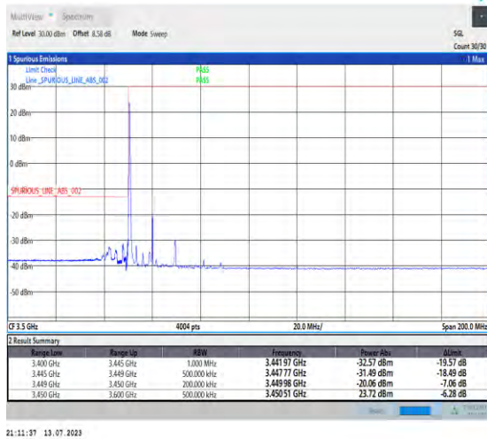
1-N77-3450-3550-PC1.5-30-20-L-1-DFT-PI2BPSK-Edge_1RB_Left-1@0-Ant3-1--PASS-see graph
