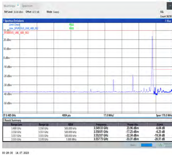
1-N77-3450-3550-PC1.5-30-40-H-2-DFT-PI2BPSK-Edge_1RB_Right-1@105-Ant3-1--PASS-see graph
