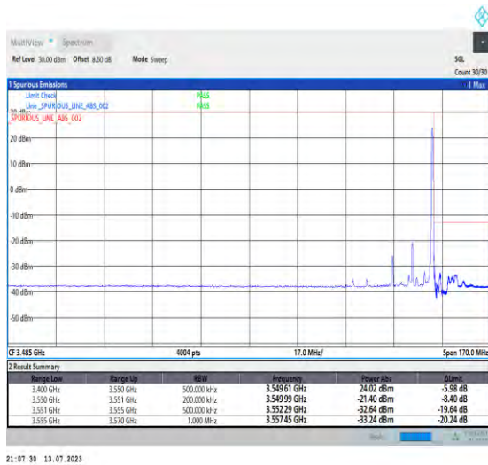
1-N77-3450-3550-PC1.5-30-15-H-2-DFT-PI2BPSK-Edge_1RB_Right-1@37-Ant3-1--PASS-see graph
