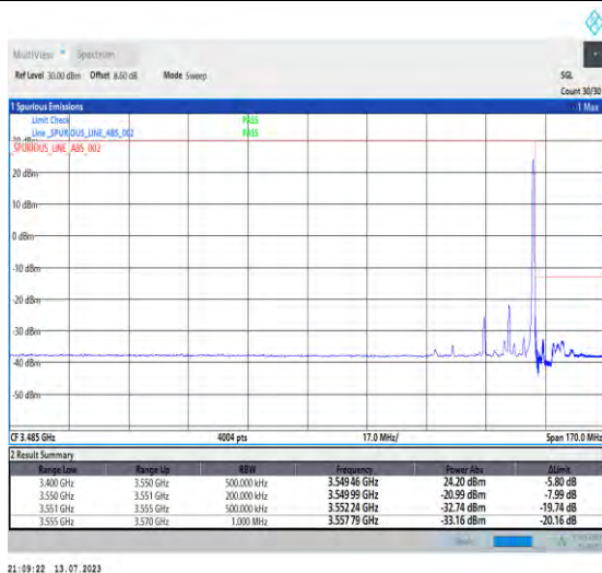
1-N77-3450-3550-PC1.5-30-15-H-5-CP-QPSK-Edge_1RB_Right-1@37-Ant3-1--PASS-see graph
