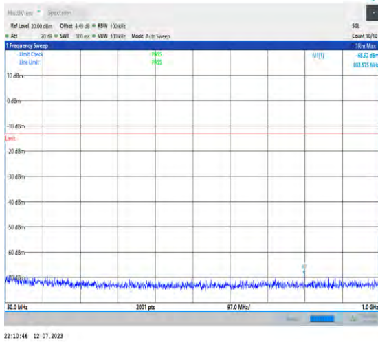
1-N77-3450-3550-PC1.5-30-100-M-1-DFT-PI2BPSK -Inner_1RB_Left-1@1-30-1000-Ant3-803.58--68.92-- 13-PASS
