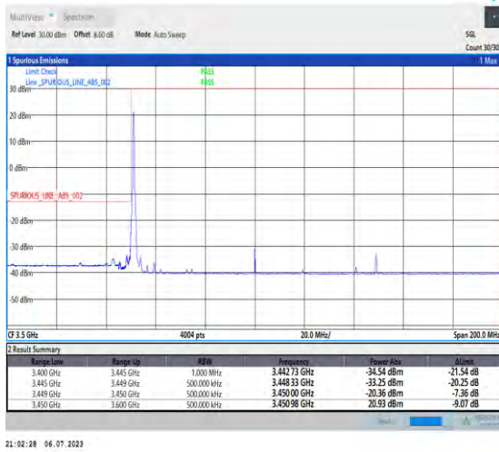
1-N77-3450-3550-PC1.5-30-100-L-1-DFT-PI2BPSK-E dge_1RB_Left-1@0-Ant3-1--PASS-see graph
