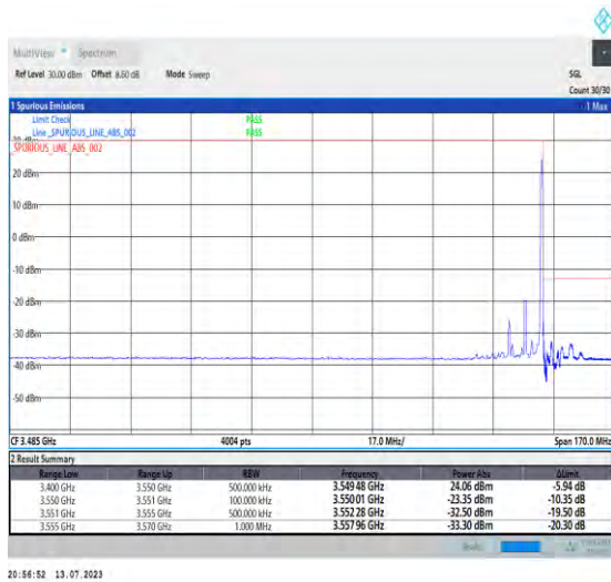
1-N77-3450-3550-PC1.5-30-10-H-2-DFT-PI2BPSK-Edge_1RB_Right-1@23-Ant3-1--PASS-see graph
