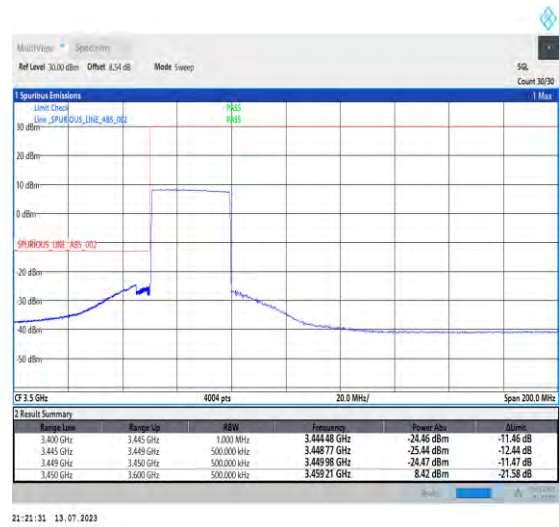
1-N77-3450-3550-PC1.5-30-30-L-3-DFT-PI2BPSK-Outer_Full-75@0-Ant3-1--PASS-see graph
