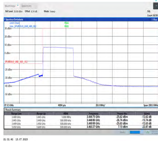
1-N77-3450-3550-PC1.5-30-40-L-6-CP-QPSK-Outer_Full-100@0-Ant3-1--PASS-see graph
