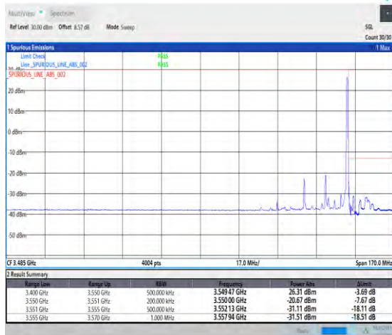
1-N77-3450-3550-PC1.5-30-20-H-2-DFT-PI2BPSK-Edge_1RB_Right-1@50-Ant3-1--PASS-see graph
