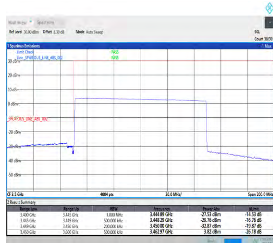
1-N77-3450-3550-PC1.5-30-100-L-3-DFT-PI2BPSK -Outer_Full-270@0-Ant3-1--PASS-see graph
