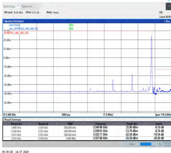
1-N77-3450-3550-PC1.5-30-40-H-5-CP-QPSK-Edge_1RB_Right-1@105-Ant3-1--PASS-see graph
