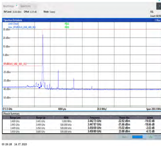
1-N77-3450-3550-PC1.5-30-40-L-4-CP-QPSK-Edge_1RB_Left-1@0-Ant3-1--PASS-see graph
