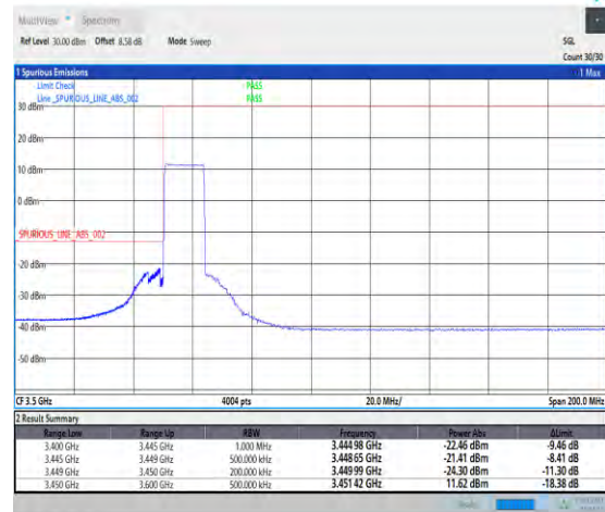
1-N77-3450-3550-PC1.5-30-15-L-3-DFT-PI2BPSK-Outer_Full-36@0-Ant3-1--PASS-see graph
