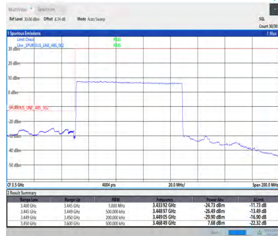
1-N77-3450-3550-PC1.5-30-80-L-3-DFT-PI2BPSK-Outer_Full-100@0-Ant3-1--PASS-see graph
