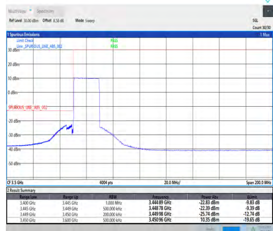
1-N77-3450-3550-PC1.5-30-20-L-6-CP-QPSK-Outer_Full-51@0-Ant3-1--PASS-see graph
