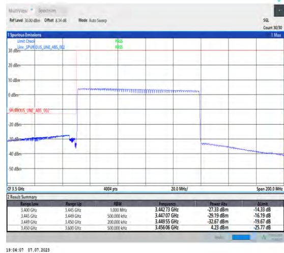
1-N77-3450-3550-PC1.5-30-90-L-6-CP-QPSK-Outer_Full-245@0-Ant3-1--PASS-see graph
