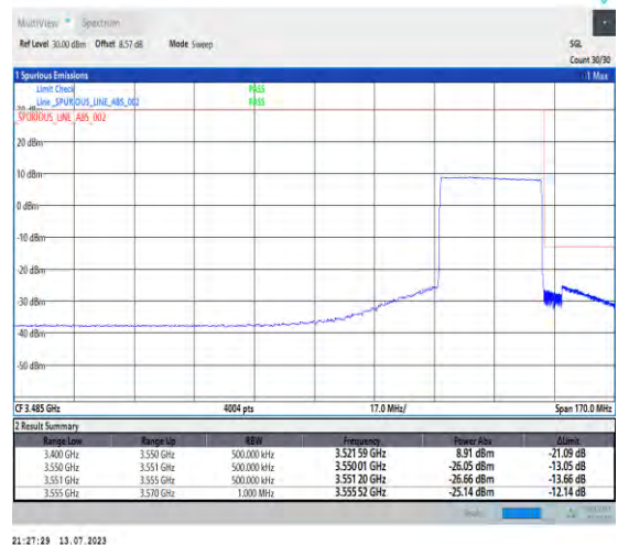
1-N77-3450-3550-PC1.5-30-30-H-6-CP-QPSK-Outer_Full-75@0-Ant3-1--PASS-see graph
