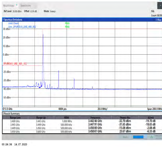
1-N77-3450-3550-PC1.5-30-40-L-1-DFT-PI2BPSK-Edge_1RB_Left-1@0-Ant3-1--PASS-see graph
