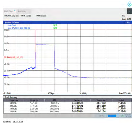
1-N77-3450-3550-PC1.5-30-30-L-6-CP-QPSK-Outer_Full-75@0-Ant3-1--PASS-see graph
