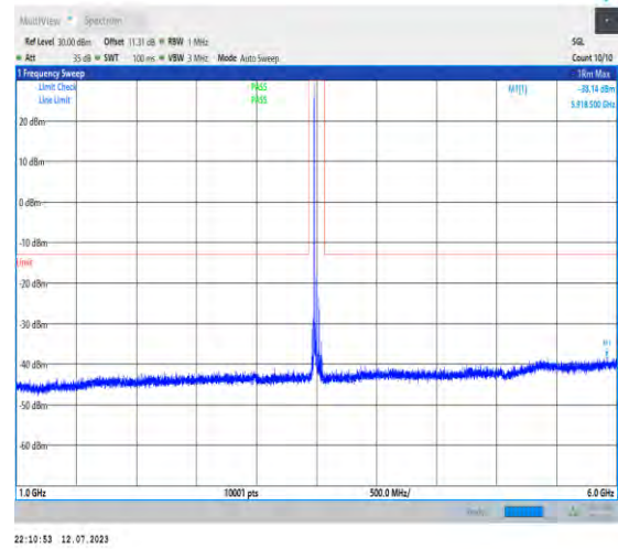
1-N77-3450-3550-PC1.5-30-100-M-1-DFT-PI2BPSK -Inner_1RB_Left-1@1-1000-6000-Ant3-5918.50--38.1 4--13-PASS
