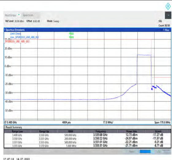
1-N77-3450-3550-PC1.5-30-15-H-6-CP-QPSK-Outer_Full-38@0-Ant3-1--PASS-see graph
