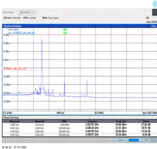
1-N77-3450-3550-PC1.5-30-60-L-4-CP-QPSK-Edge_1RB_Left-1@0-Ant3-1--PASS-see graph
