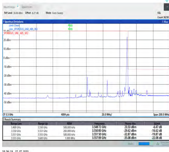
1-N77-3450-3550-PC1.5-30-50-H-5-CP-QPSK-Edge_1RB_Right-1@132-Ant3-1--PASS-see graph
