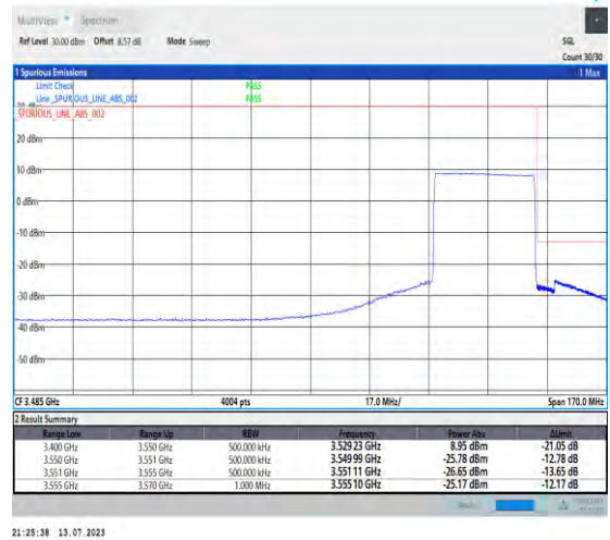
1-N77-3450-3550-PC1.5-30-30-H-3-DFT-PI2BPSK-Outer_Full-75@0-Ant3-1--PASS-see graph
