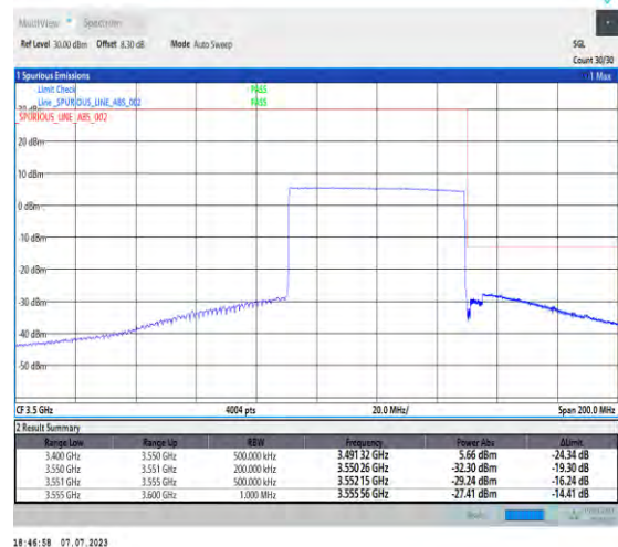
1-N77-3450-3550-PC1.5-30-60-H-6-CP-QPSK-Out_Full-162@0-Ant3-1--PASS-see graph
