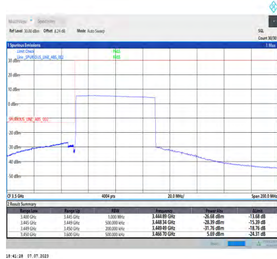
1-N77-3450-3550-PC1.5-30-60-L-6-CP-QPSK-Outer_Full-162@0-Ant3-1--PASS-see graph
