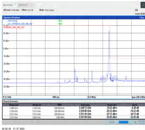
1-N77-3450-3550-PC1.5-30-50-H-2-DFT-PI2BPSK-Edge_1RB_Right-1@132-Ant3-1--PASS-see graph
