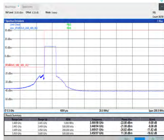
1-N77-3450-3550-PC1.5-30-15-L-6-CP-QPSK-Outer_Full-38@0-Ant3-1--PASS-see graph
