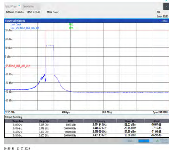
1-N77-3450-3550-PC1.5-30-10-L-6-CP-QPSK-Outer_Full-24@0-Ant3-1--PASS-see graph
