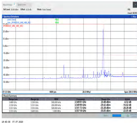
1-N77-3450-3550-PC1.5-30-60-H-2-DFT-PI2BPSK-Edge_1RB_Right-1@161-Ant3-1--PASS-see graph
