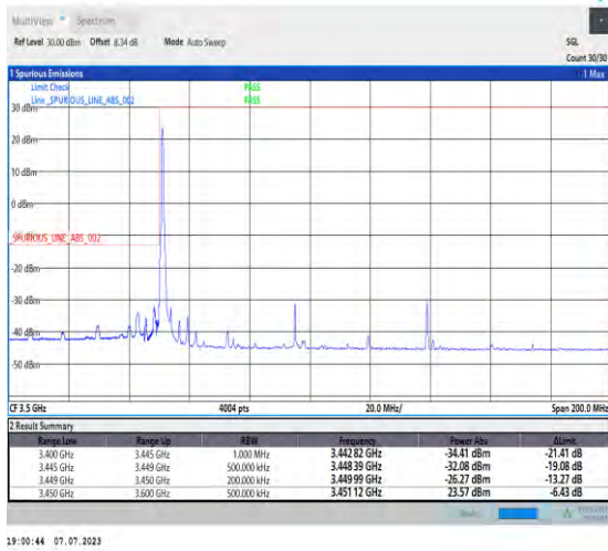
1-N77-3450-3550-PC1.5-30-90-L-1-DFT-PI2BPSK-Edge_1RB_Left-1@0-Ant3-1--PASS-see graph
