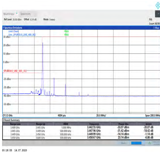
1-N77-3450-3550-PC1.5-30-30-L-4-CP-QPSK-Edge_1RB_Left-1@0-Ant3-1--PASS-see graph
