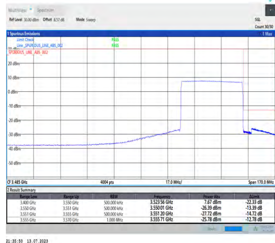
1-N77-3450-3550-PC1.5-30-40-H-6-CP-QPSK-Out_Full-100@0-Ant3-1--PASS-see graph
