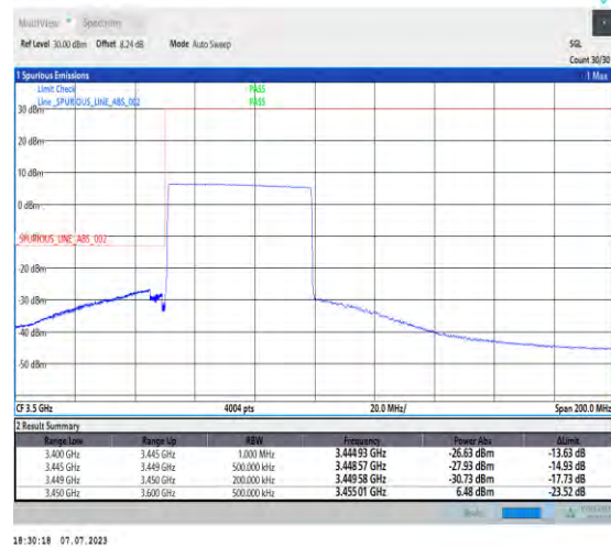
1-N77-3450-3550-PC1.5-30-50-L-6-CP-QPSK-Outer_Full-133@0-Ant3-1--PASS-see graph
