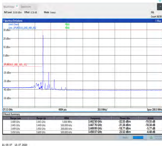
1-N77-3450-3550-PC1.5-30-15-L-4-CP-QPSK-Edge_1RB_Left-1@0-Ant3-1--PASS-see graph
