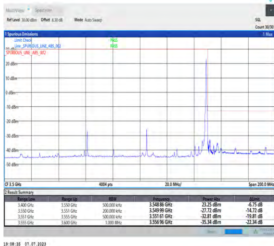
1-N77-3450-3550-PC1.5-30-90-H-5-CP-QPSK-Edge_1RB_Right-1@244-Ant3-1--PASS-see graph
