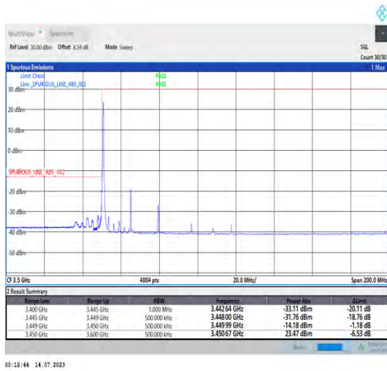
1-N77-3450-3550-PC1.5-30-30-L-1-DFT-PI2BPSK-Edge_1RB_Left-1@0-Ant3-1--PASS-see graph
