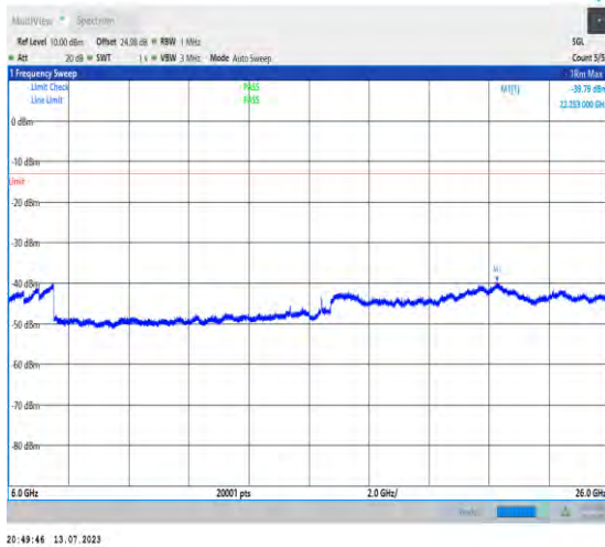
1-N77-3450-3550-PC1.5-30-100-M-1-DFT-QPSK-Edge_1RB_Left-1@0-6000-26000-Ant3-22253.00--39.7 9--13-PASS
