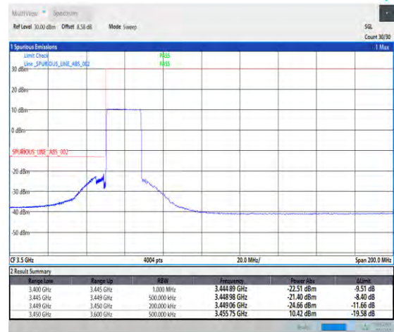
1-N77-3450-3550-PC1.5-30-20-L-3-DFT-PI2BPSK-Outer_Full-50@0-Ant3-1--PASS-see graph
