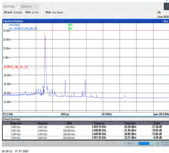
1-N77-3450-3550-PC1.5-30-50-L-4-CP-QPSK-Edge_1RB_Left-1@0-Ant3-1--PASS-see graph
