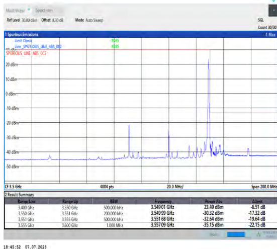
1-N77-3450-3550-PC1.5-30-60-H-5-CP-QPSK-Edge_1RB_Right-1@161-Ant3-1--PASS-see graph
