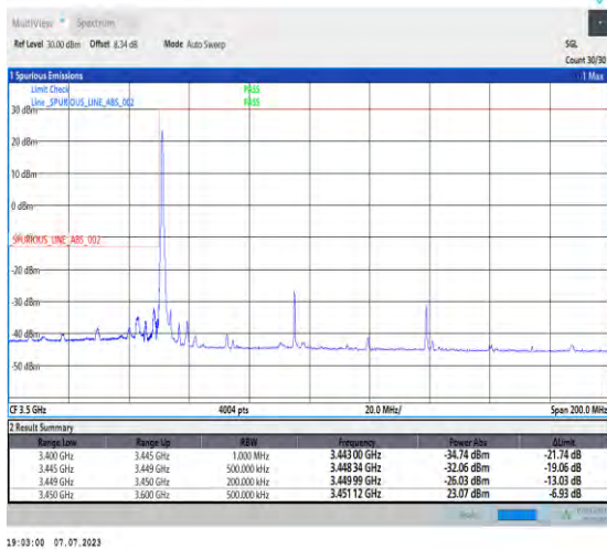
1-N77-3450-3550-PC1.5-30-90-L-4-CP-QPSK-Edge_1RB_Left-1@0-Ant3-1--PASS-see graph
