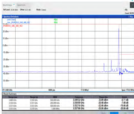
1-N77-3450-3550-PC1.5-30-20-H-5-CP-QPSK-Edge_1RB_Right-1@50-Ant3-1--PASS-see graph
