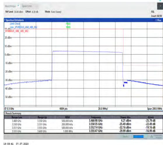
1-N77-3450-3550-PC1.5-30-90-H-6-CP-QPSK-Outer_Full-245@0-Ant3-1--PASS-see graph
