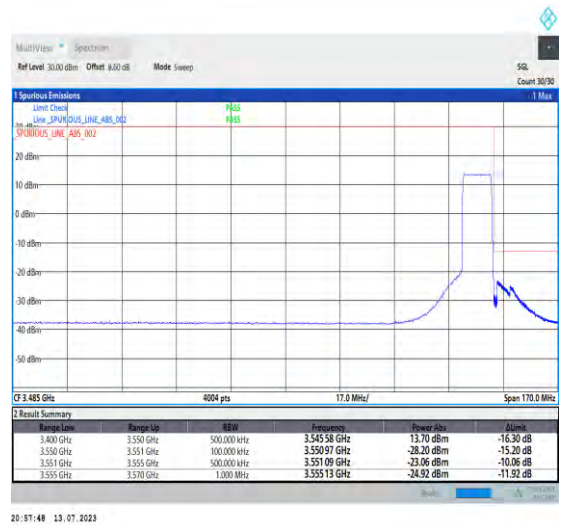
1-N77-3450-3550-PC1.5-30-10-H-3-DFT-PI2BPSK-Outer_Full-24@0-Ant3-1--PASS-see graph
