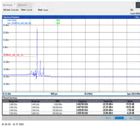
1-N77-3450-3550-PC1.5-30-10-L-1-DFT-PI2BPSK-Edge_1RB_Left-1@0-Ant3-1--PASS-see graph
