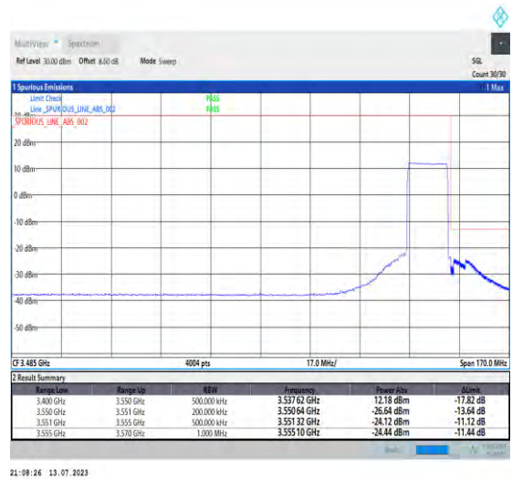
1-N77-3450-3550-PC1.5-30-15-H-3-DFT-PI2BPSK-Outer_Full-36@0-Ant3-1--PASS-see graph
