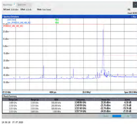
1-N77-3450-3550-PC1.5-30-90-H-2-DFT-PI2BPSK-Edge_1RB_Right-1@244-Ant3-1--PASS-see graph
