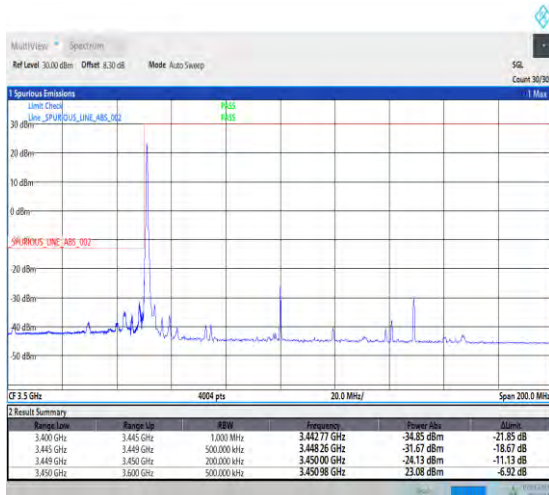
1-N77-3450-3550-PC1.5-30-100-L-1-DFT-PI2BPSK-E dge_1RB_Left-1@0-Ant3-1--PASS-see graph
