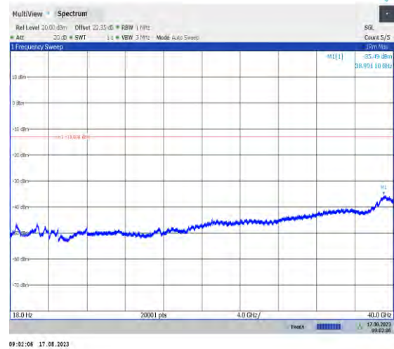
1-N77-3450-3550-PC1.5-30-100-M-1-DFT-PI2BPSK -Inner_1RB_Left-1@1-18000-40000-Ant3-18000.00-- 57.00--13-PASS
