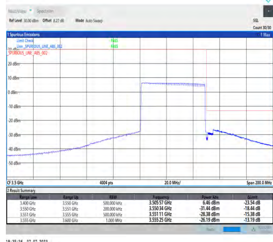
1-N77-3450-3550-PC1.5-30-50-H-6-CP-QPSK-Outer_Full-133@0-Ant3-1--PASS-see graph
