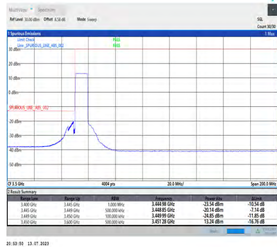
1-N77-3450-3550-PC1.5-30-10-L-3-DFT-PI2BPSK-Outer_Full-24@0-Ant3-1--PASS-see graph
