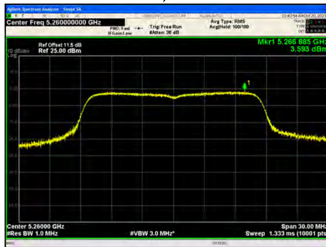
802.11a, 5260MHz
