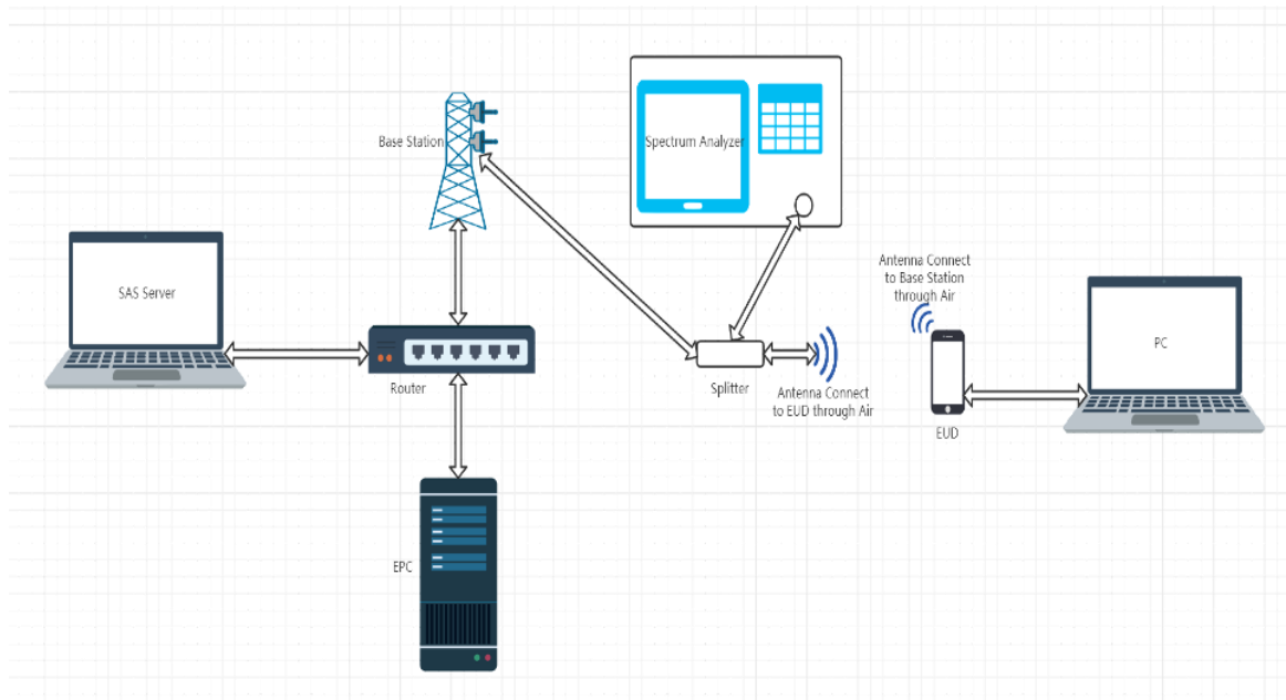
Test setup diagram for WINNF.PT.C.HBT Test case
