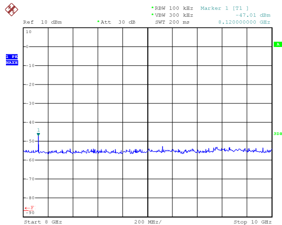
Plot 6 (8÷10GHz)
