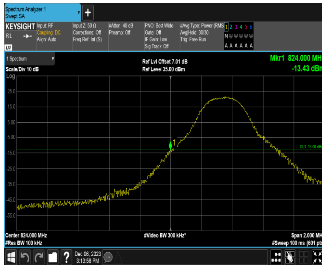
Band26-5MHz-16QAM-26815-1RB#24
