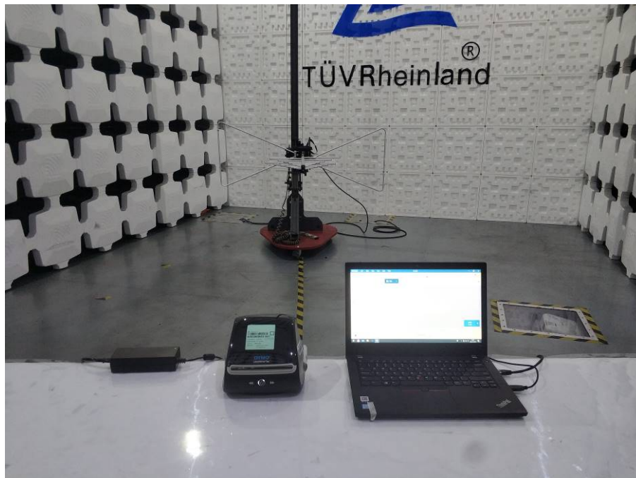
Photograph 1: Set-up photo for Radiated Emission, Below 1GHz
