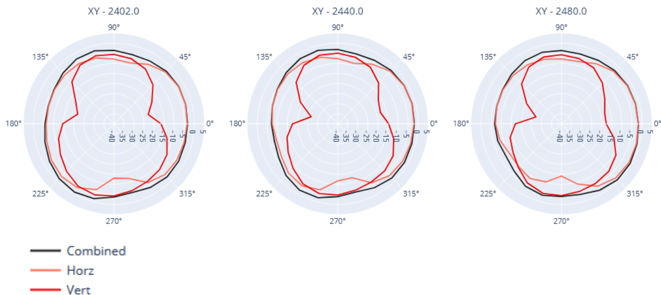
Figure 1 – Gain X-Y
