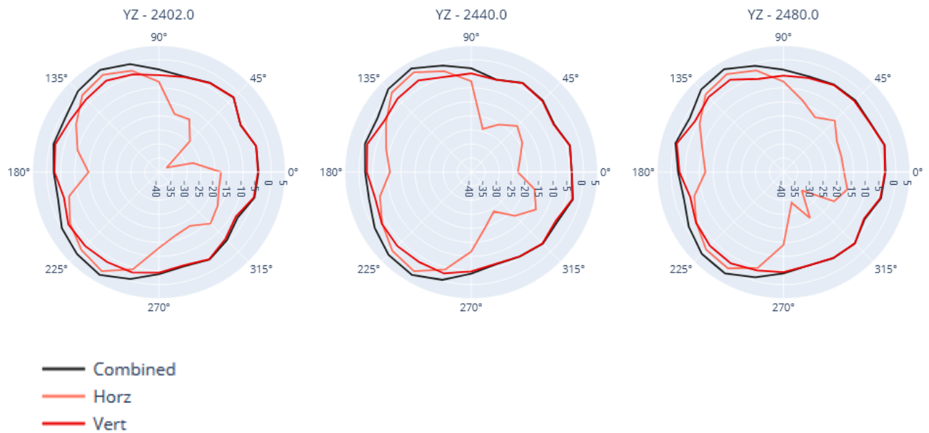
Figure 3 - Gain Y-Z
