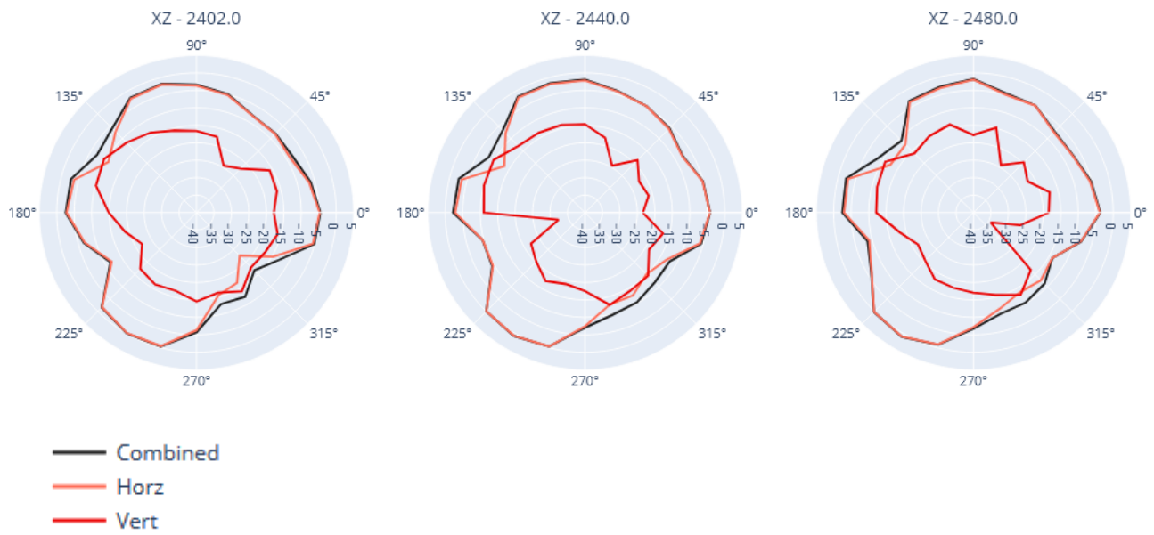
Figure 2 - Gain X-Z
