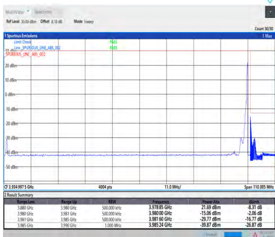
1-N77-3700-3980--30-100-H-2-DFT-PI2BPSK-Edge_1 RB_Right-1@272-Ant1-1--PASS-see graph
