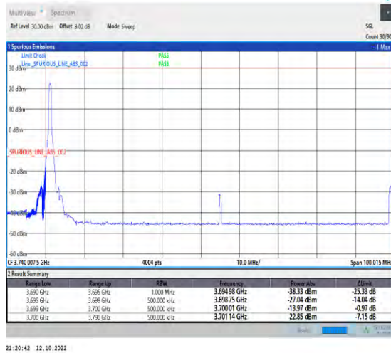
1-N77-3700-3980--30-90-L-1-DFT-PI2BPSK-Edge_1R B_Left-1@0-Ant1-1--PASS-see graph
