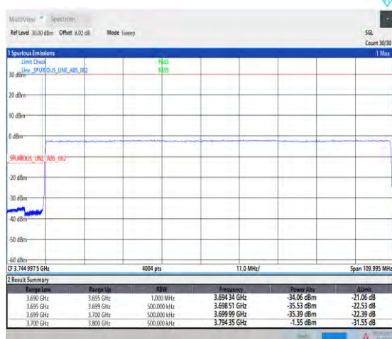
1-N77-3700-3980--30-100-L-6-CP-QPSK-Outer_F ull-273@0-Ant1-1--PASS-see graph
