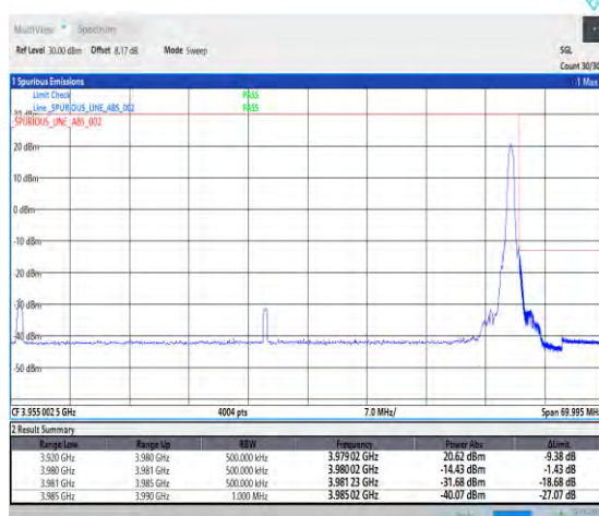
1-N77-3700-3980--30-60-H-5-CP-QPSK-Edge_1RB_R ight-1@161-Ant1-1--PASS-see graph
