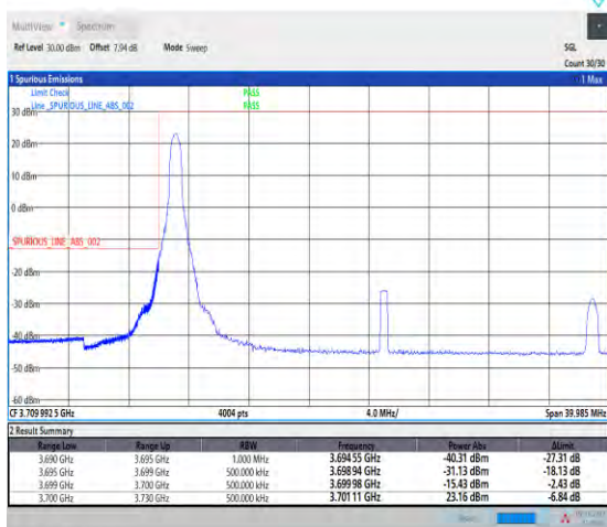
1-N77-3700-3980--30-30-L-1-DFT-PI2BPSK-Edge_1R B_Left-1@0-Ant1-1--PASS-see graph
