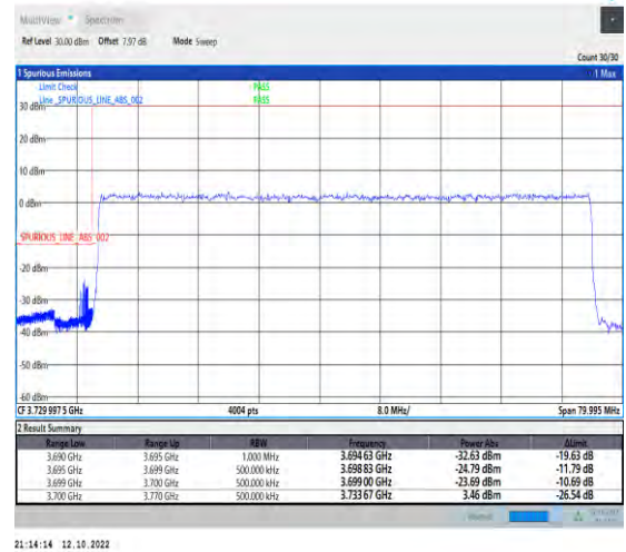
1-N77-3700-3980--30-70-L-3-DFT-PI2BPSK-Outer _Full-180@0-Ant1-1--PASS-see graph
