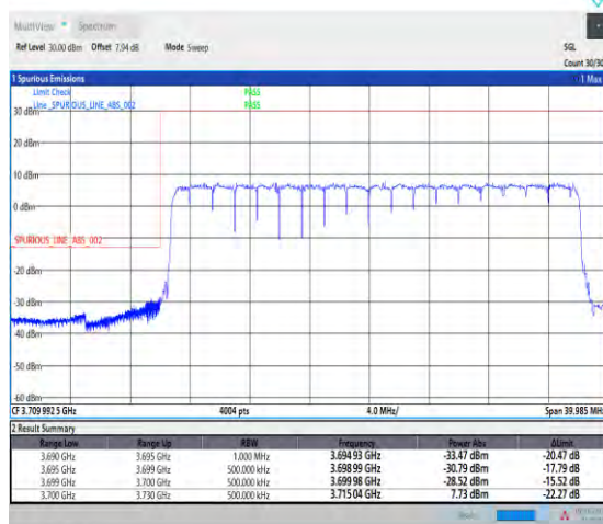
1-N77-3700-3980--30-30-L-3-DFT-PI2BPSK-Outer _Full-75@0-Ant1-1--PASS-see graph
