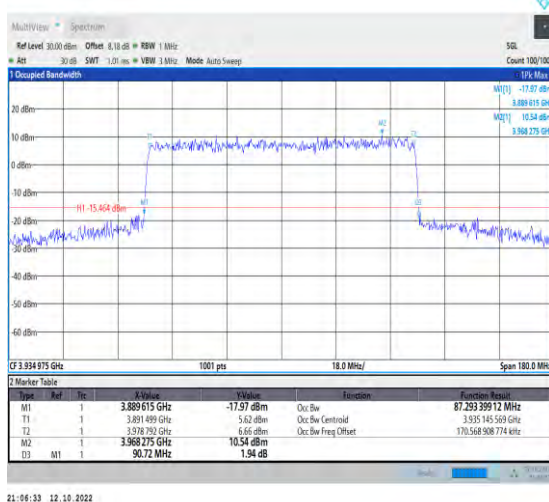
1-N77-3700-3980--30-90-H-8-CP-64QAM-Outer_Full-245@0-Ant1-87.293-90.720≤90-PASS
