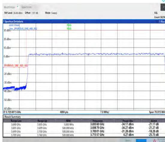
1-N77-3700-3980--30-60-L-3-DFT-PI2BPSK-Outer_Full-162@0-Ant1-1--PASS-see graph
