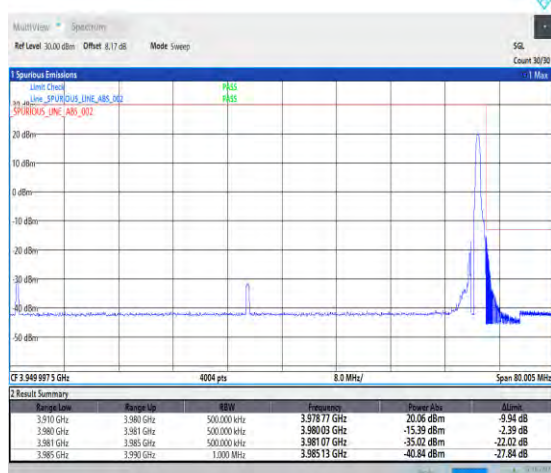
1-N77-3700-3980--30-70-H-5-CP-QPSK-Edge_1RB_R ight-1@188-Ant1-1--PASS-see graph
