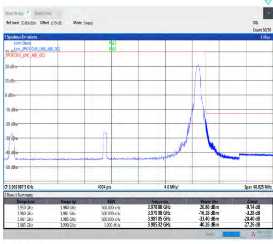
1-N77-3700-3980--30-30-H-5-CP-QPSK-Edge_1RB_R ight-1@77-Ant1-1--PASS-see graph
