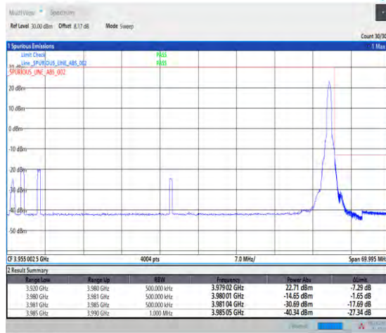
1-N77-3700-3980--30-60-H-2-DFT-PI2BPSK-Edge_1R B_Right-1@161-Ant1-1--PASS-see graph
