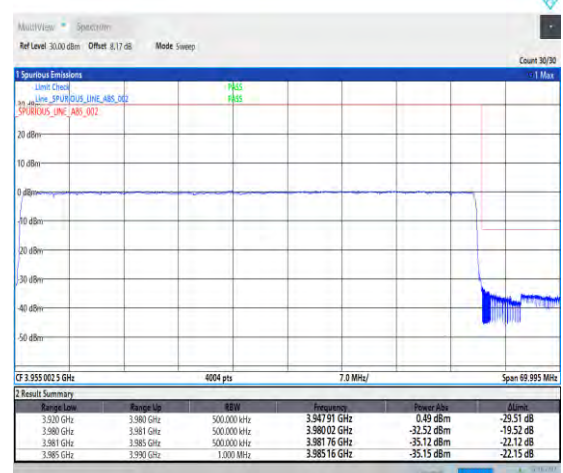
1-N77-3700-3980--30-60-H-6-CP-QPSK-Outer_Ful I-162@0-Ant1-1--PASS-see graph
