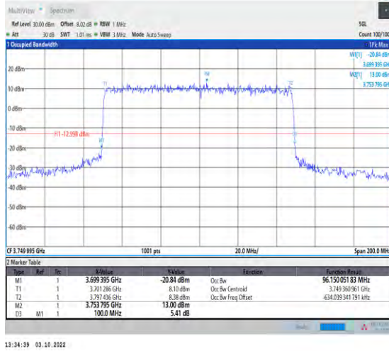
1-N77-3700-3980--30-100-L-1-DFT-QPSK-Outer_Full-I-270@0-Ant1-96.15-100.000-≤100-PASS
