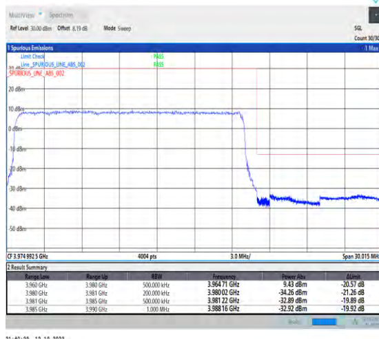
1-N77-3700-3980--30-20-H-3-DFT-PI2BPSK-Outer_Full-50@0-Ant1-1--PASS-see graph
