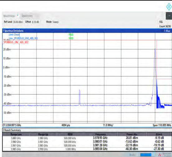
1-N77-3700-3980--30-100-H-2-DFT-PI2BPSK-Edge_1 RB_Right-1@272-Ant1-1--PASS-see graph
