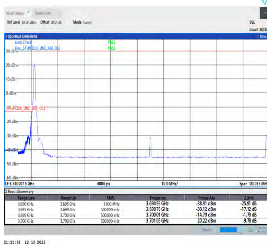
1-N77-3700-3980--30-90-L-4-CP-QPSK-Edge_1RB_L eft-1@0-Ant1-1--PASS-see graph
