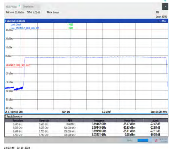
1-N77-3700-3980--30-80-L-6-CP-QPSK-Outer_Ful I-217@0-Ant1-1--PASS-see graph
