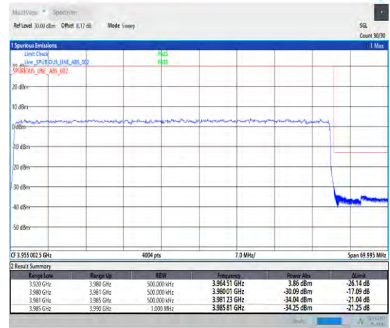
1-N77-3700-3980--30-60-H-3-DFT-PI2BPSK-Outer _Full-162@0-Ant1-1--PASS-see graph
