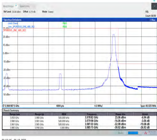
1-N77-3700-3980--30-30-H-2-DFT-PI2BPSK-Edge_1R_B_Right-1@77-Ant1-1--PASS-see graph
