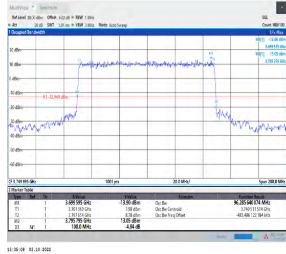
1-N77-3700-3980--30-100-L-2-DFT-PI2BPSK-Outer_Full-270@0-Ant1-96.286-100.000-≤100-PASS
