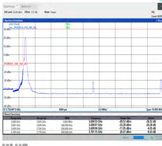
1-N77-3700-3980--30-70-L-4-CP-QPSK-Edge_1RB_L eft-1@0-Ant1-1--PASS-see graph
