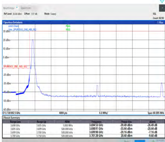
1-N77-3700-3980--30-50-L-4-CP-QPSK-Edge_1RB_L eft-1@0-Ant1-1--PASS-see graph
