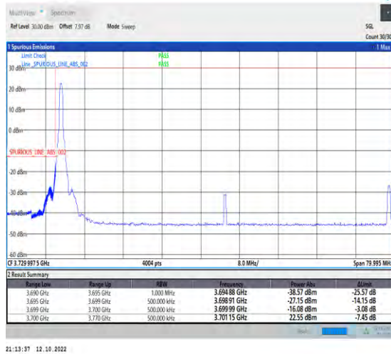
1-N77-3700-3980--30-70-L-1-DFT-PI2BPSK-Edge_1R B_Left-1@0-Ant1-1--PASS-see graph
