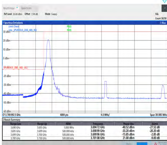
1-N77-3700-3980--30-30-L-4-CP-QPSK-Edge_1RB_L eft-1@0-Ant1-1--PASS-see graph
