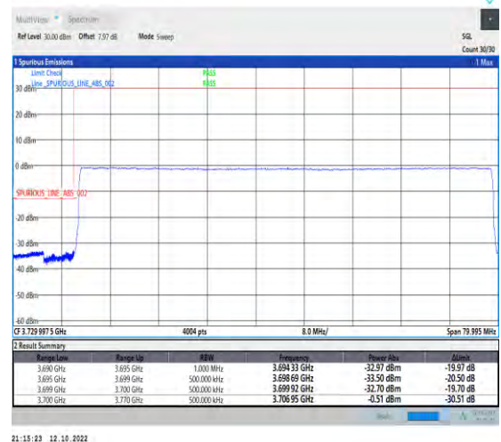
1-N77-3700-3980--30-70-L-6-CP-QPSK-Outer_Ful l-189@0-Ant1-1--PASS-see graph
