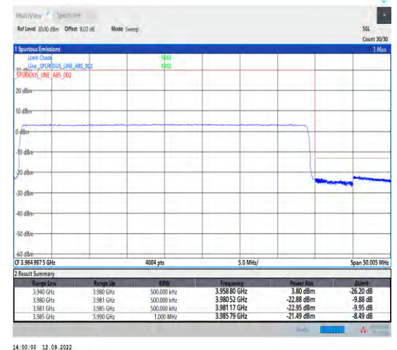
1-N77-3700-3980--30-40-H-6-CP-QPSK-Outer_Ful I-106@0-Ant1-1--PASS-see graph
