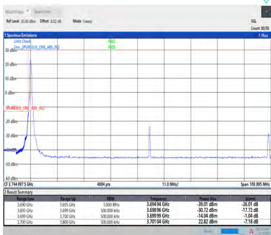
1-N77-3700-3980--30-100-L-1-DFT-PI2BPSK-Edge_1 RB_Left-1@0-Ant1-1--PASS-see graph
