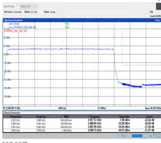
1-N77-3700-3980--30-30-H-3-DFT-PI2BPSK-Outer_Full-75@0-Ant1-1--PASS-see graph
