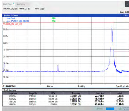
1-N77-3700-3980--30-70-H-2-DFT-PI2BPSK-Edge_1R B_Right-1@188-Ant1-1--PASS-see graph
