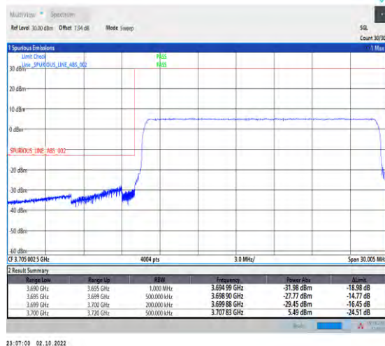
1-N77-3700-3980--30-20-L-6-CP-QPSK-Outer_Ful I-51@0-Ant1-1--PASS-see graph
