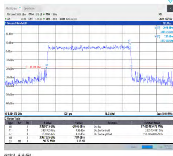
1-N77-3700-3980--30-90-H-9-CP-256QAM-Outer_Full-245@0-Ant1-87.42-90.720≤90-PASS
