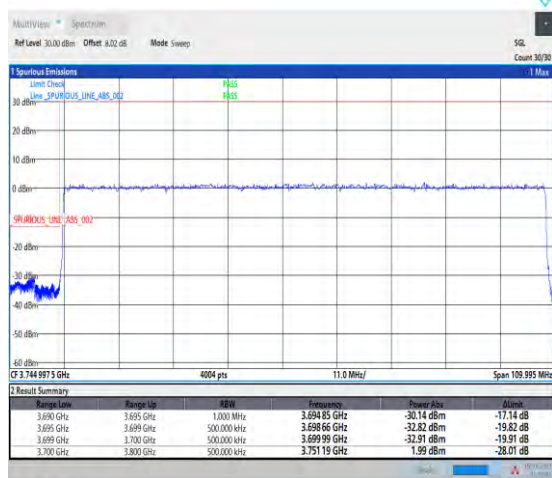
1-N77-3700-3980--30-100-L-3-DFT-PI2BPSK-Outer_F Full-270@0-Ant1-1--PASS-see graph
