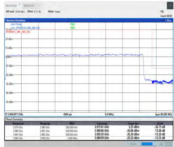
1-N77-3700-3980--30-70-H-3-DFT-PI2BPSK-Outer _Full-180@0-Ant1-1--PASS-see graph
