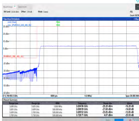
1-N77-3700-3980--30-30-L-6-CP-QPSK-Outer_Ful l-78@0-Ant1-1--PASS-see graph
