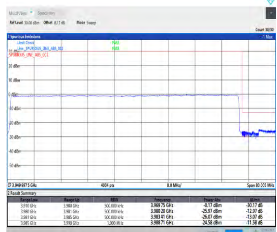
1-N77-3700-3980--30-70-H-6-CP-QPSK-Outer_Ful I-189@0-Ant1-1--PASS-see graph
