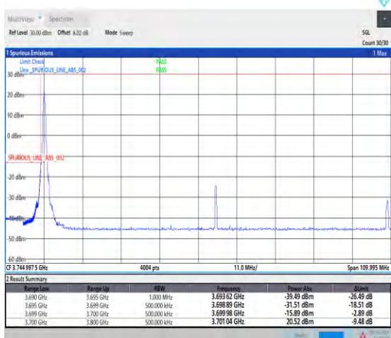
1-N77-3700-3980--30-100-L-4-CP-QPSK-Edge_1RB_ Left-1@0-Ant1-1--PASS-see graph
