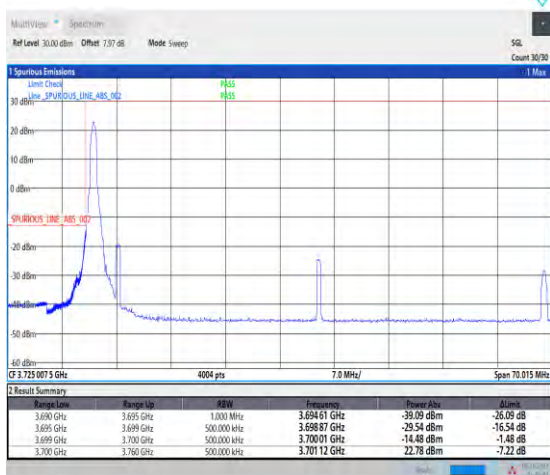
1-N77-3700-3980--30-60-L-1-DFT-PI2BPSK-Edge_1R_B_Left-1@0-Ant1-1--PASS-see graph
