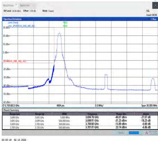
1-N77-3700-3980--30-20-L-1-DFT-PI2BPSK-Edge_1R_B_Left-1@0-Ant1-1--PASS-see graph
