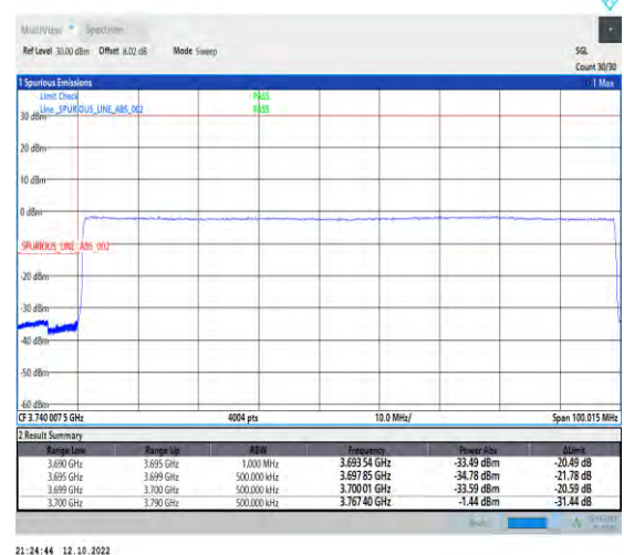
1-N77-3700-3980--30-90-L-6-CP-QPSK-Outer_Ful I-245@0-Ant1-1--PASS-see graph
