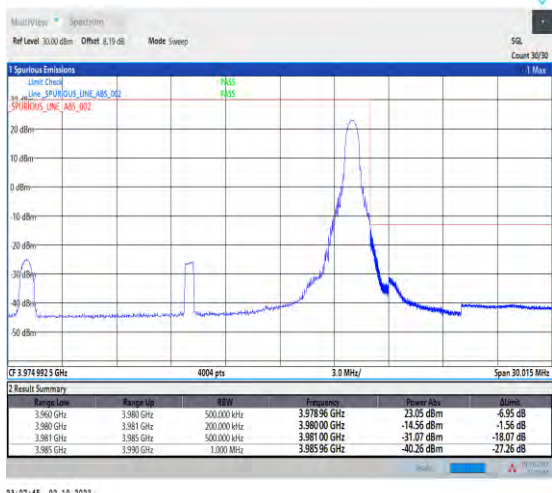
1-N77-3700-3980--30-20-H-2-DFT-PI2BPSK-Edge_1R_B_Right-1@50-Ant1-1--PASS-see graph
