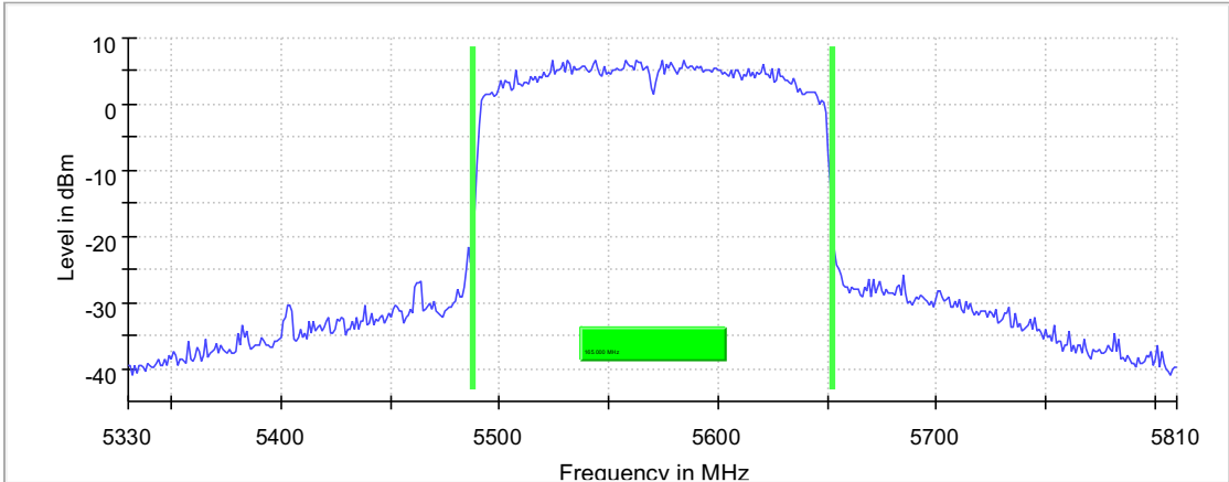
26 dB Bandwidth
