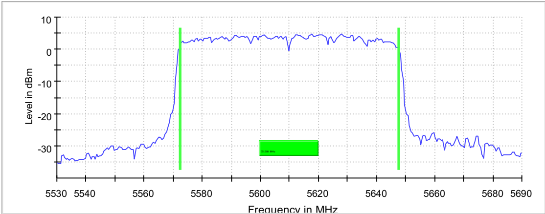
99 % Bandwidth
