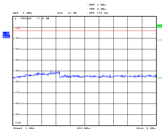
LTE Band 14 10MHz CH- Middle 1GHz~9GHz
