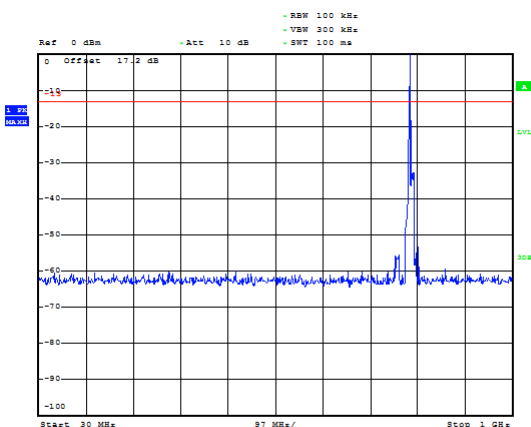
LTE Band 14 10MHz CH- Middle 30MHz~1GHz
