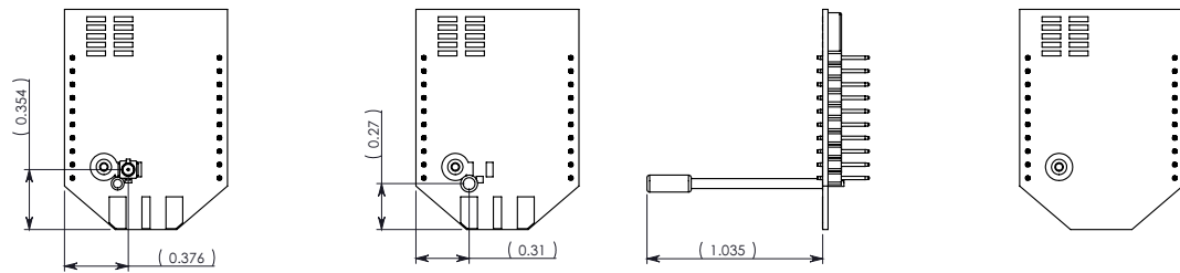
WIRE WHIP
