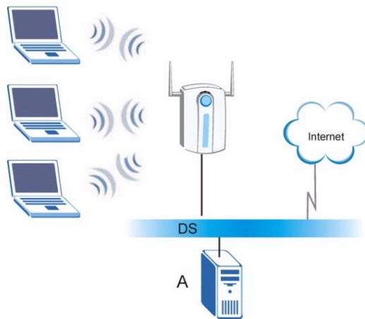
Figure 52 WPA(2) with RADIUS Application Example
