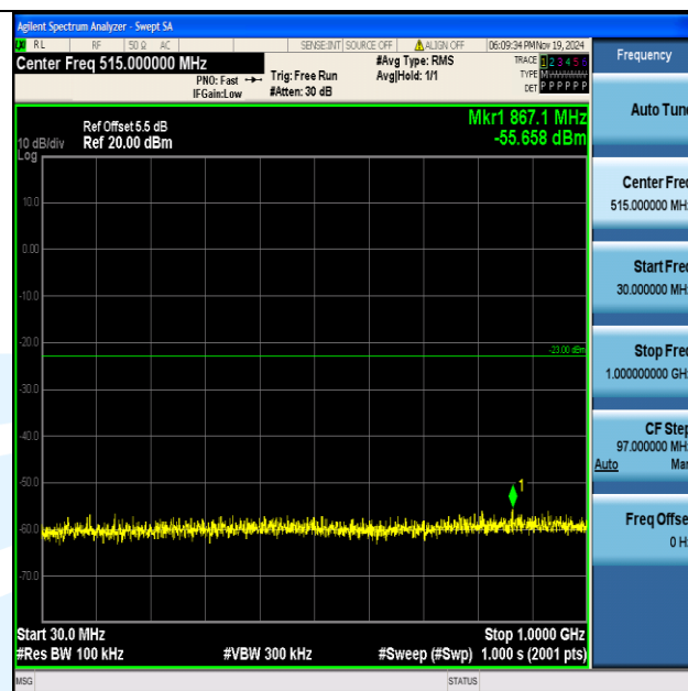
Band2_3MHz_16QAM_19185_1RB#0_30~1000_30~1000
