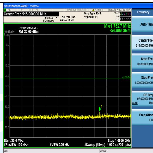
Band2_10MHz_16QAM_19150_1RB#0_30~1000_30~1000
