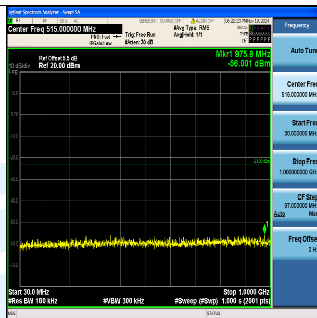
Band2_5MHz_16QAM_18625_1RB#0_30~1000_30~1000
