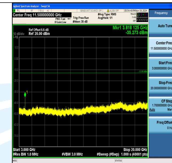
Band2_1.4MHz_16QAM_19193_1RB#0_3000~20000_3000~20000
