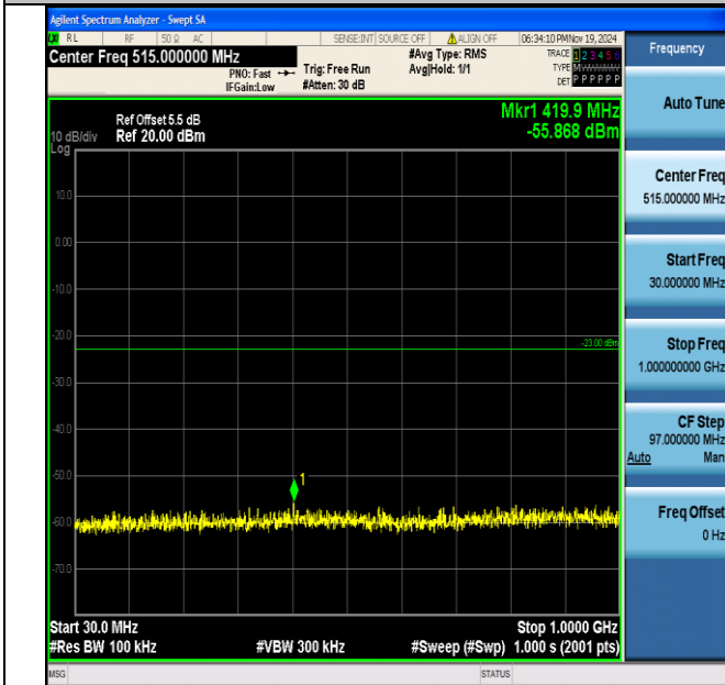
Band2_10MHz_QPSK_18650_1RB#0_30~1000_30~1000
