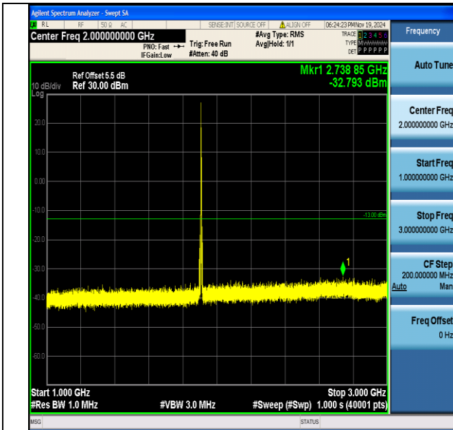
Band2_5MHz_16QAM_19175_1RB#0_1000~3000_1000~3000
