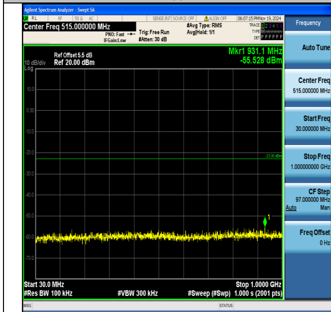
Band2_3MHz_QPSK_18615_1RB#0_30~1000_30~1000
