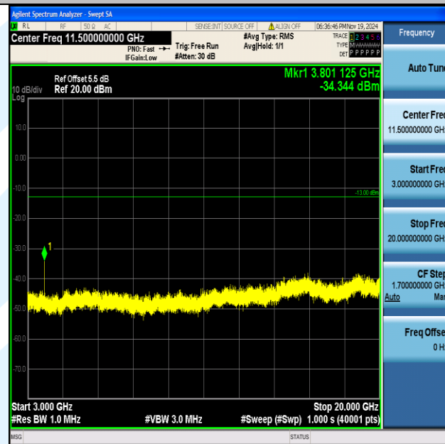
Band2_10MHz_16QAM_19150_1RB#0_3000~20000_3000~20000
