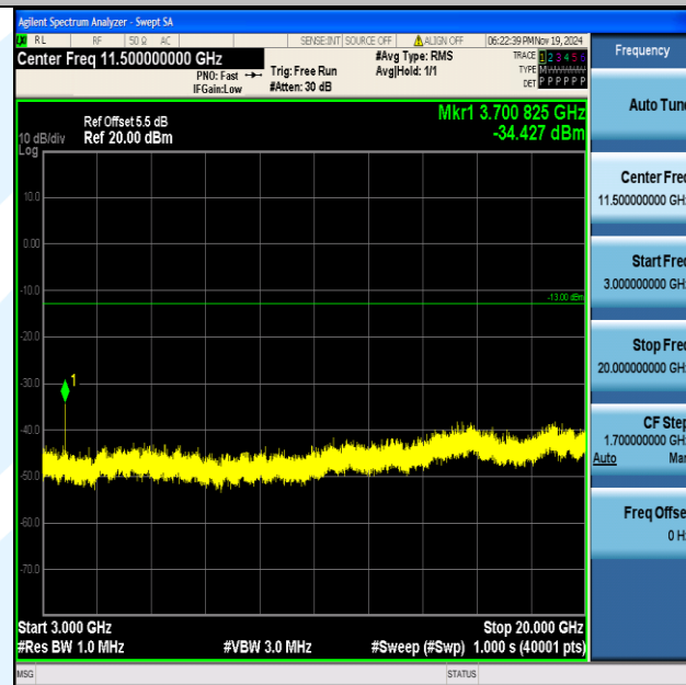
Band2_5MHz_16QAM_18625_1RB#0_3000~20000_3000~20000
