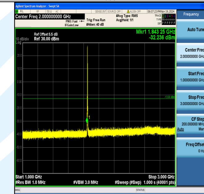
Band2_3MHz_QPSK_18615_1RB#0_1000~3000_1000~3000
