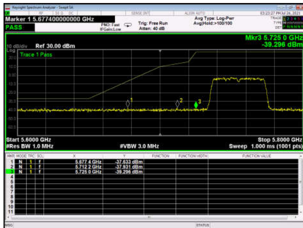
U-NII-3 ,Plot 1,Band Edge-802.11ax(80 MHz),5775MHz,Ant1 Left side bandedge
