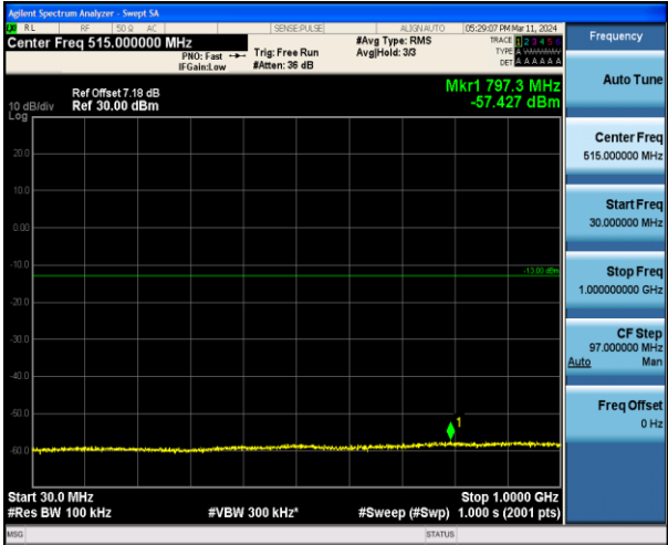
Band4_10MHz_QPSK_20350_1RB#0_30~1000_30~1000
