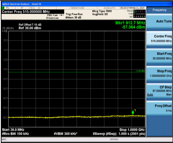
Band4_10MHz_16QAM_20350_1RB#0_30~1000_30~1000
