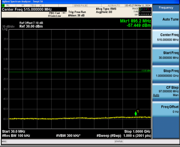
Band4_15MHz_16QAM_20025_1RB#0_30~1000_30~1000
