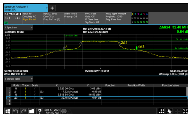
Figure 42 - 802.11a SP Maximum 99% OBW
