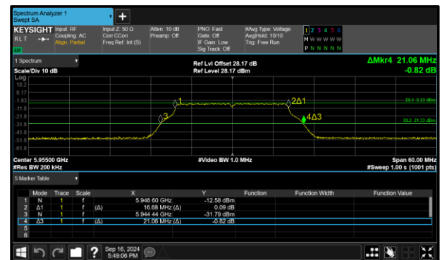
Figure 32 - 802.11a LPI Maximum 99% OBW
