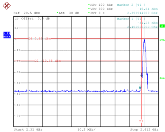
BLE(2M): Band edge-left side
