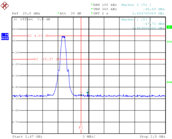
BLE(1M): Band edge-right side
