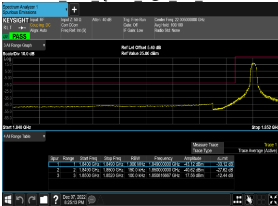
B2 15M 16QAM 1@0 CH 18675
