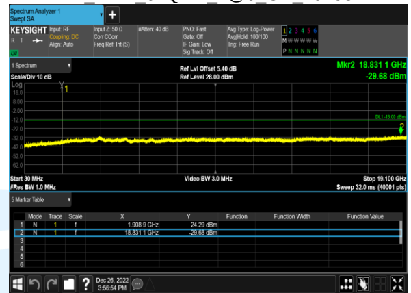
B2 1.4M 64QAM 1@0 CH 19193
