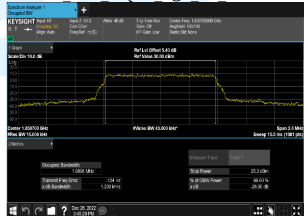
B2_1.4M_64QAM_6@0_CH_18607
