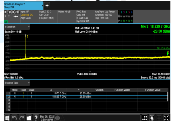
B2 10M 64QAM 1@0 CH 18900
