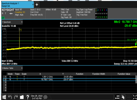
B2 15M 64QAM 1@0 CH 18900
