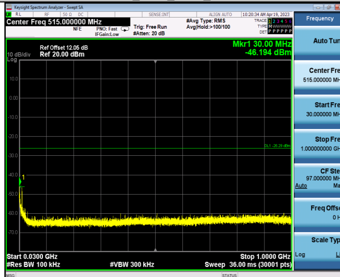
11N40SISO_Ant1_2437_30~1000
