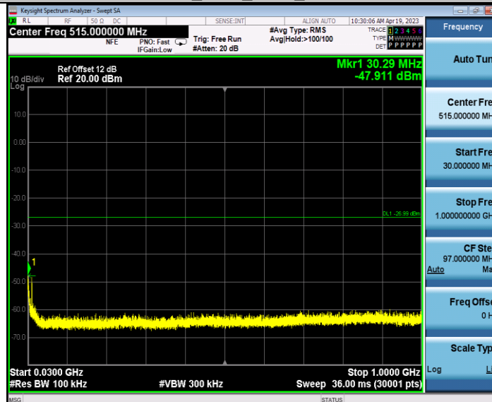
11N40SISO_Ant1_2452_30~1000
