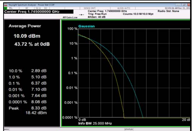
FDD66_20MHz_1745_fullRB_Q16
