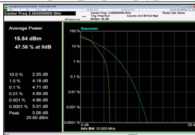
FDD07_10MHz_2565_OneRB_high_Q16
