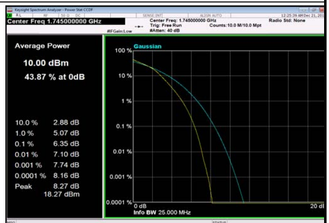
FDD04_20MHz_1745_fullRB_Q16
