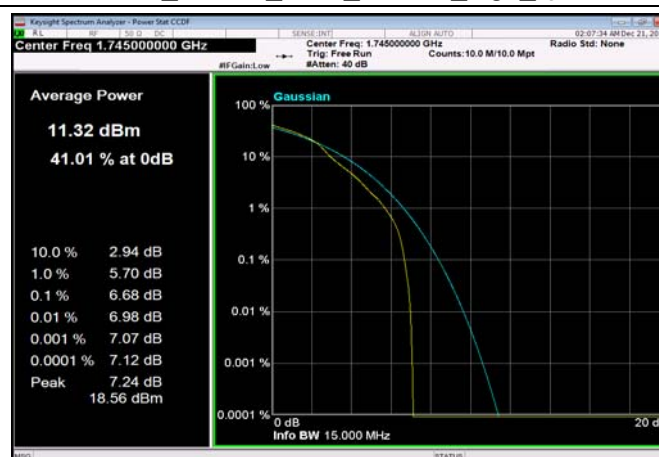
FDD66_15MHz_1745_OneRB_high_Q16
