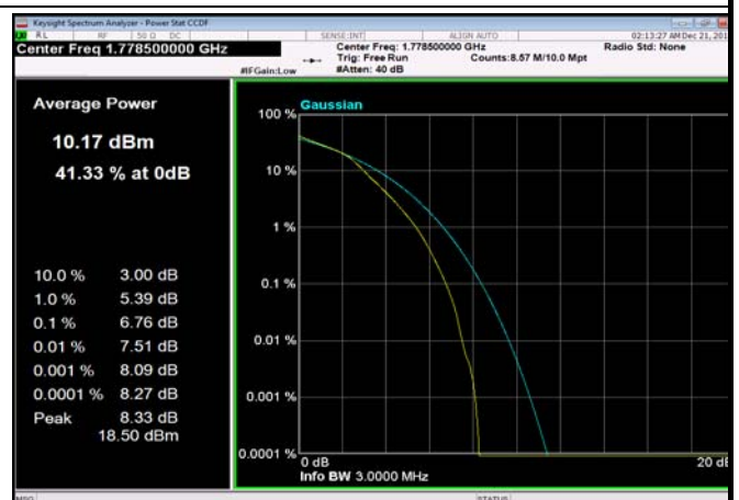
FDD66_3MHz_1778.5_fullRB_Q16
