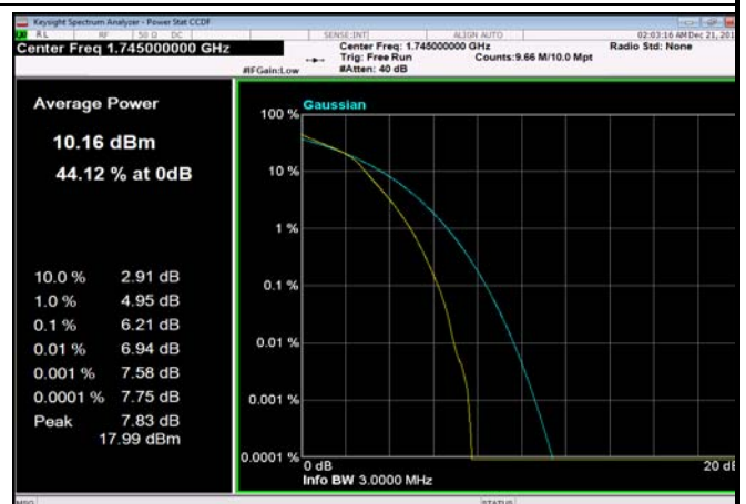
FDD66_3MHz_1745_fullRB_Q16
