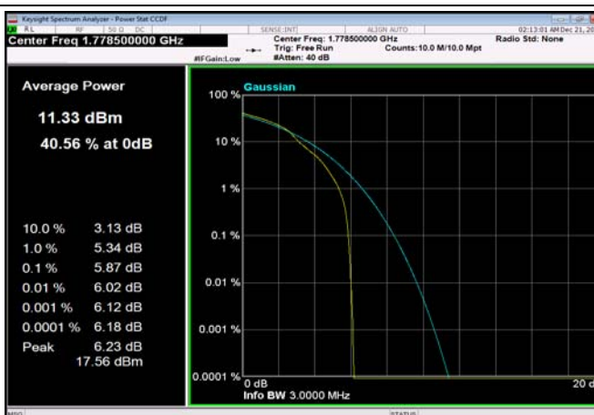
FDD66_3MHz_1778.5_OneRB_high_Q16
