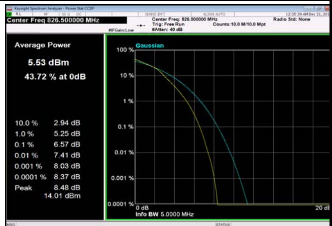
FDD05_5MHz_826.5_fullRB_Q16
