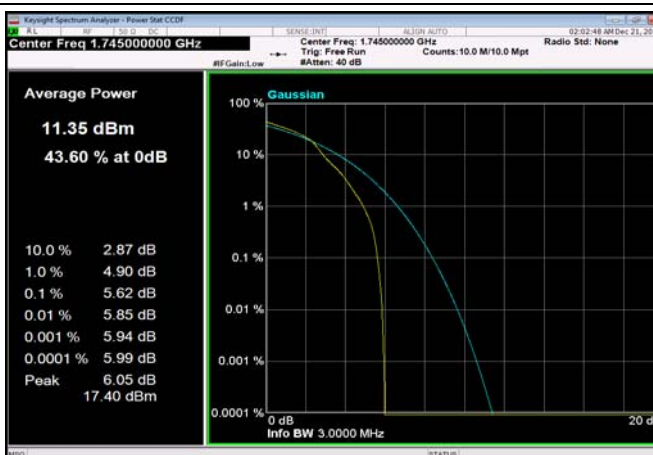
FDD66_3MHz_1745_OneRB_high_Q16
