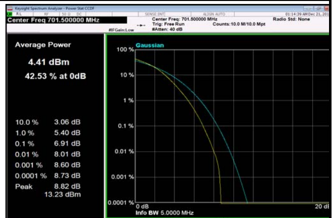
FDD12_5MHz_701.5_fullRB_Q16
