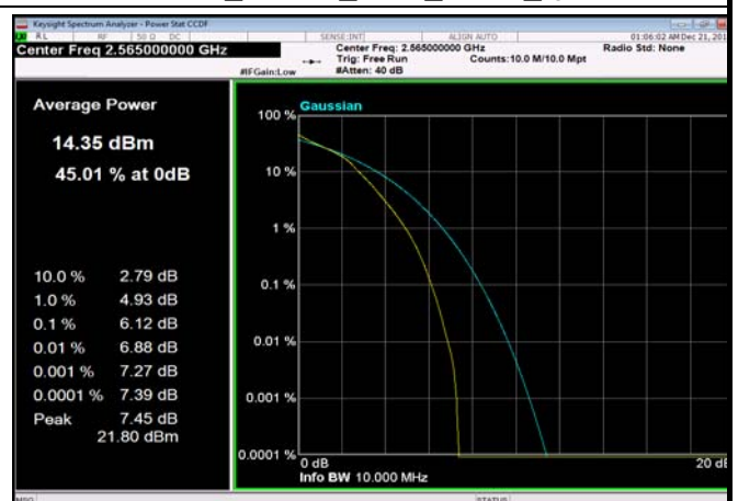
FDD07_10MHz_2565_fullRB_Q16
