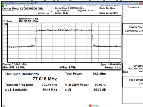
Band77-Part27_80MHz_DFT_s_OFDM_SCS30kHz_64QAM_RB216_0_CH633334
