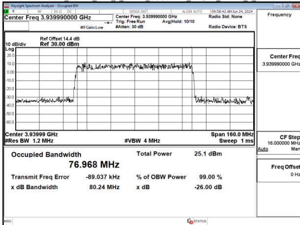
Band77-Part27_80MHz_DFT_s_OFDM_SCS30kHz_64QAM_RB216_0_CH662668
