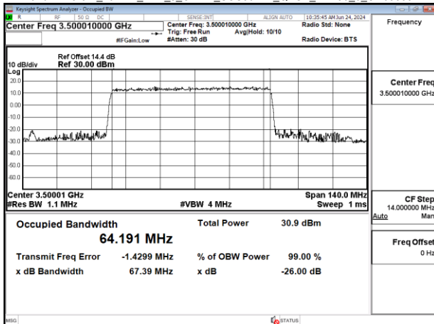
Band7-Part27_70MHz_DFT_s_OFDM_SCS30kHz_QPSK_RB180_0_CH633334
