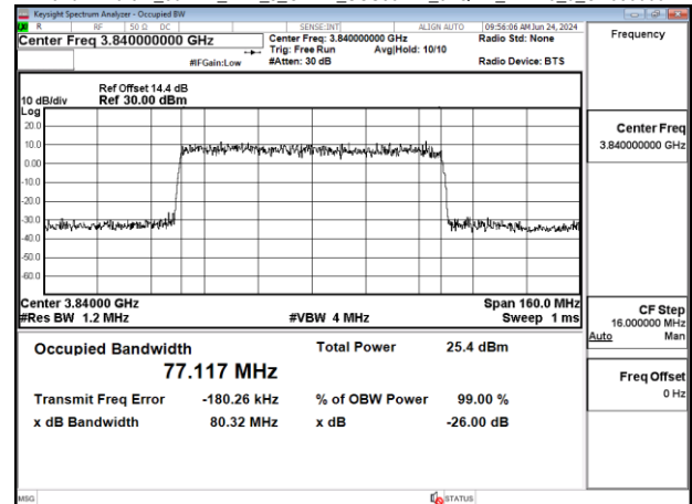
Band77-Part27_80MHz_DFT_s_OFDM_SCS30kHz_64QAM_RB216_0_CH656000
