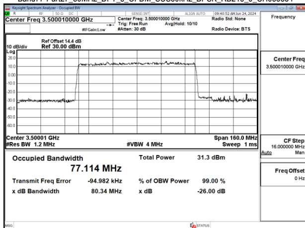
Band77-Part27_80MHz_DFT_s_OFDM_SCS30kHz_BPSK_RB216_0_CH633334
