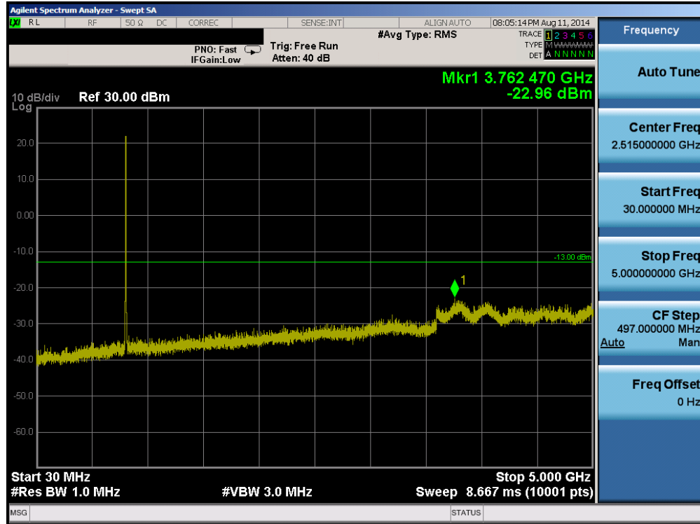
Plot 6-9. Conducted Spurious Plot (Cellular WCDMA Mode – Ch. 4132)
