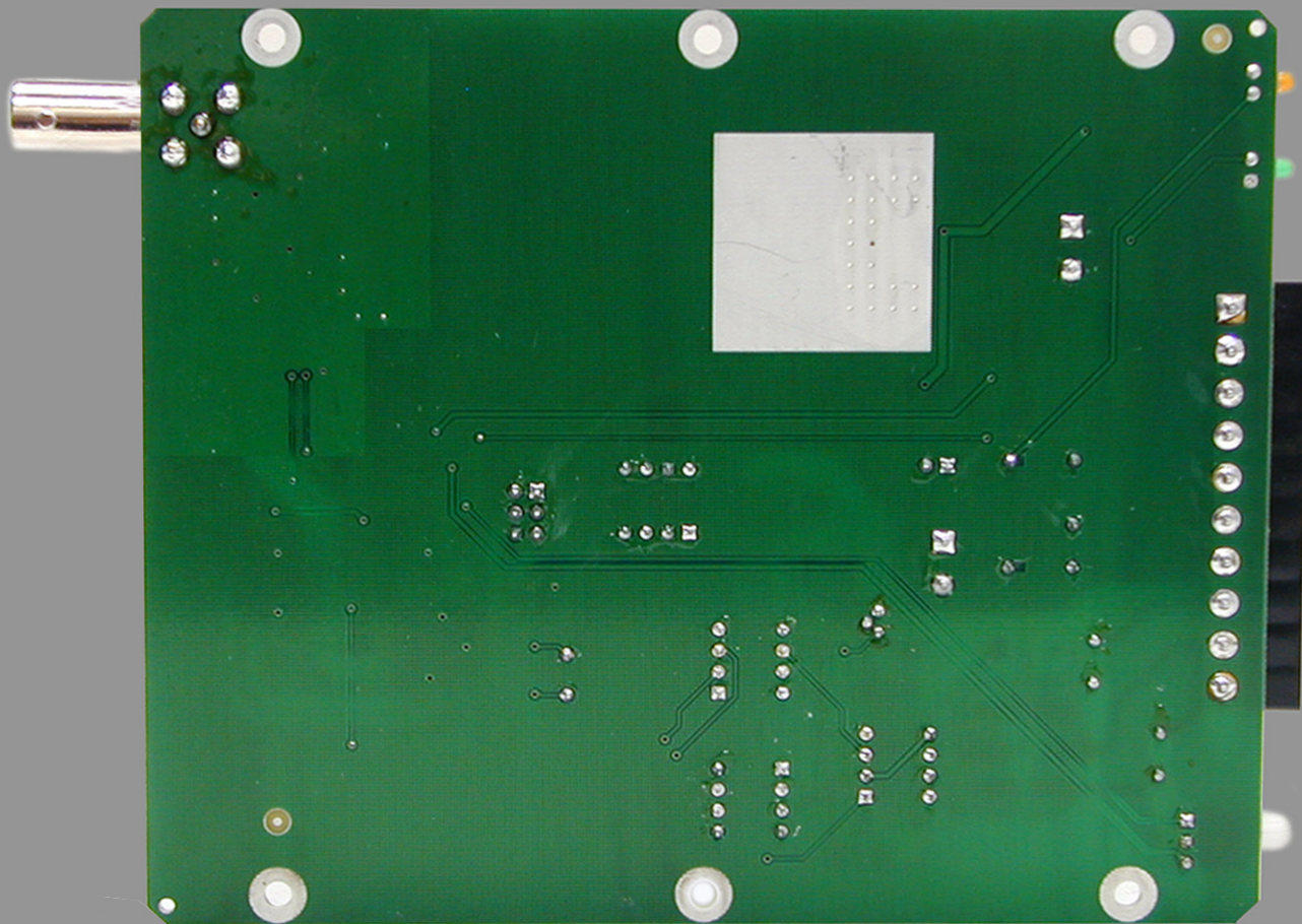
Receiver PCB Bottom View
