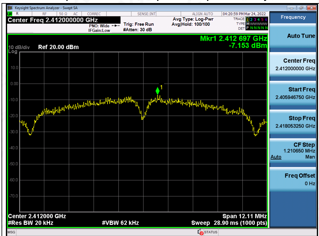
Test_Graph_802.11b_ANT2_2412_1Mbps_PSD
