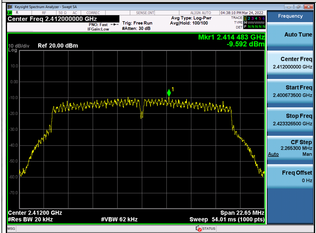
Test_Graph_802.11g_ANT2_2412_6Mbps_PSD
