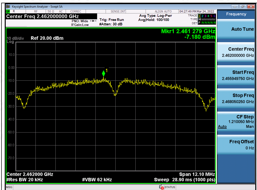
Test_Graph_802.11b_ANT2_2462_1Mbps_PSD
