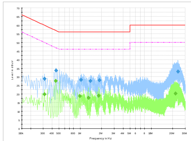
Fig.B.11.1 AC Powerline Conducted Emission-traffic
