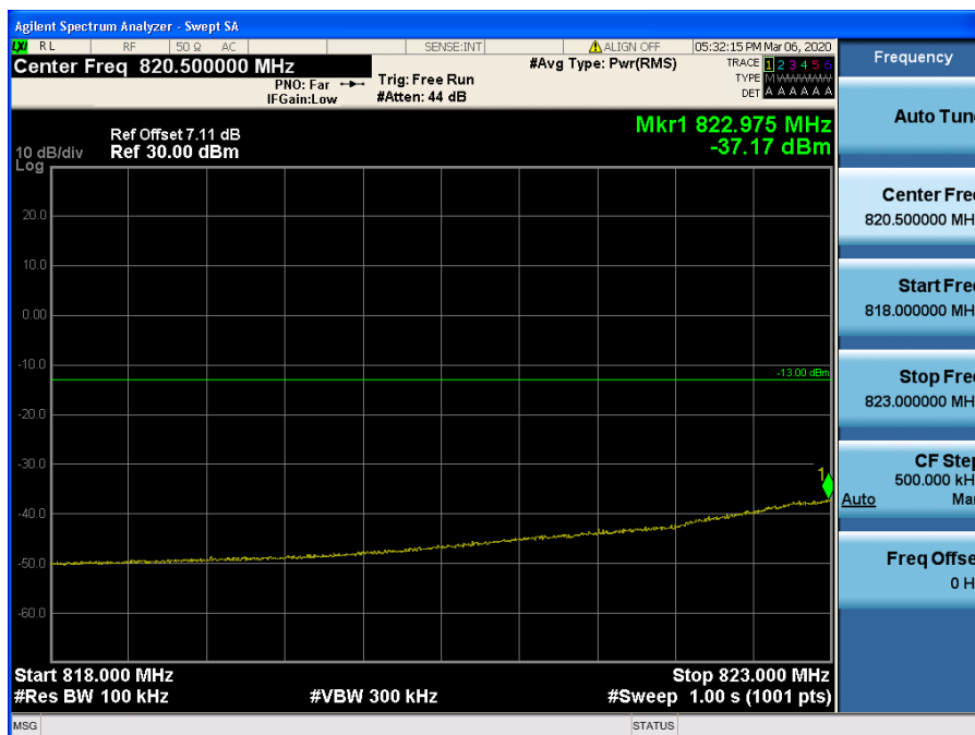
LTE Band 5 / 5MHz / 16QAM - RB Size/Offset (12/0)
