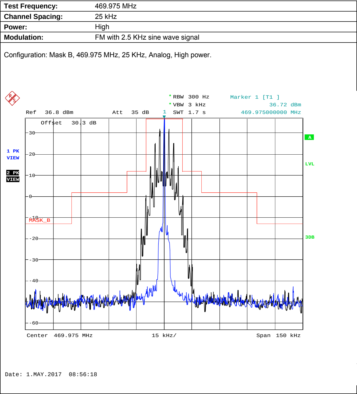
Plot 5.8.4.3.3. Emission Mask B, High Power
