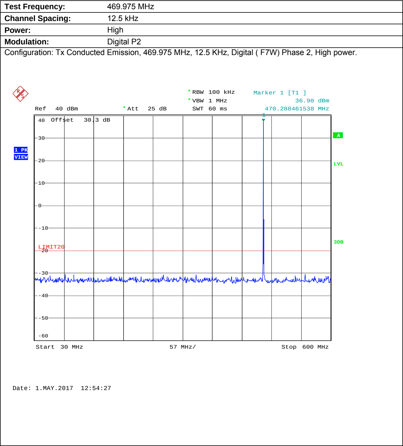
Plot 5.9.4.3.1. Conducted Transmitter Spurious Emissions for 469.975 MHz, High Power
