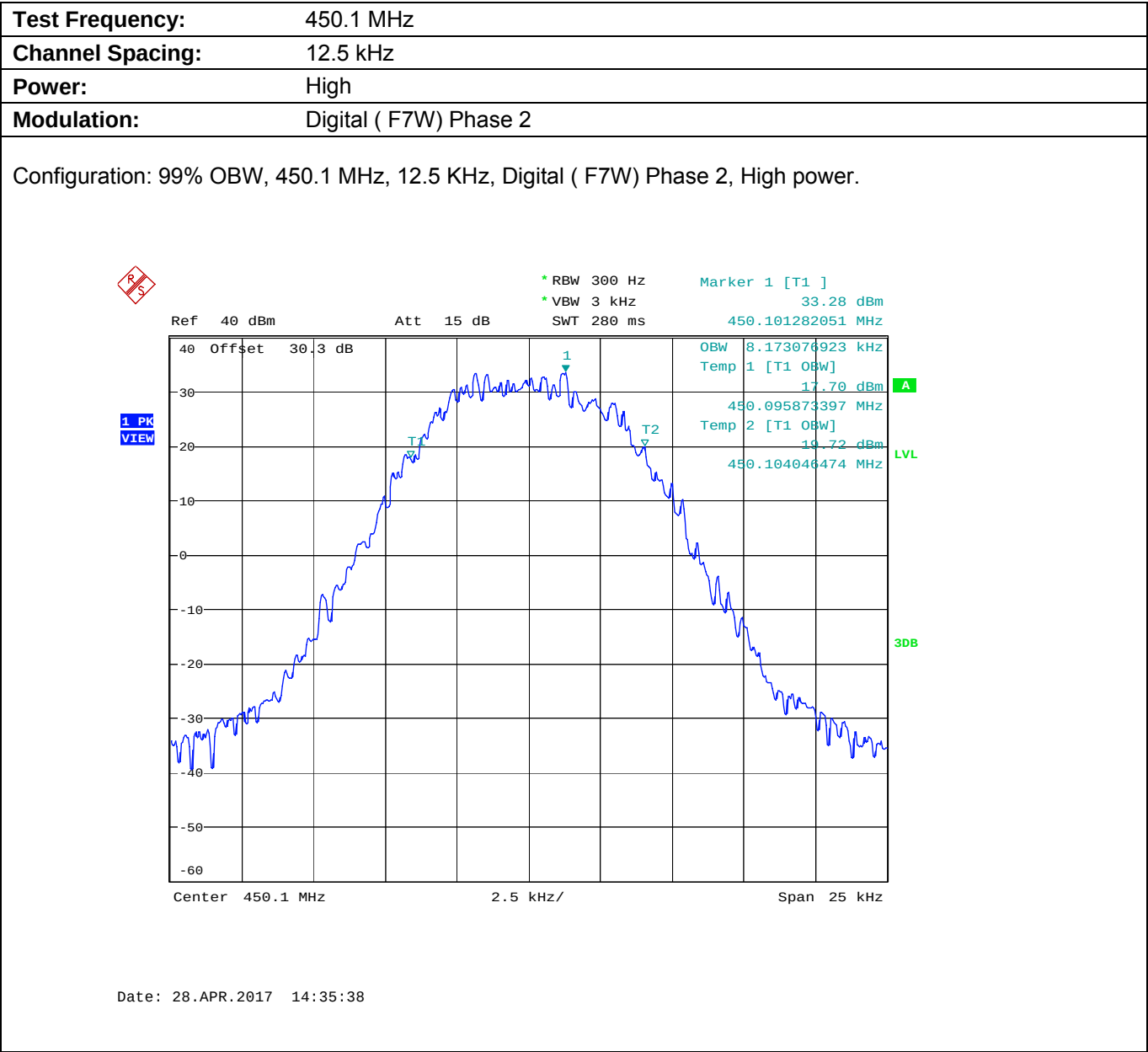
Plot 5.8.4.1.11. Occupied Bandwidth
