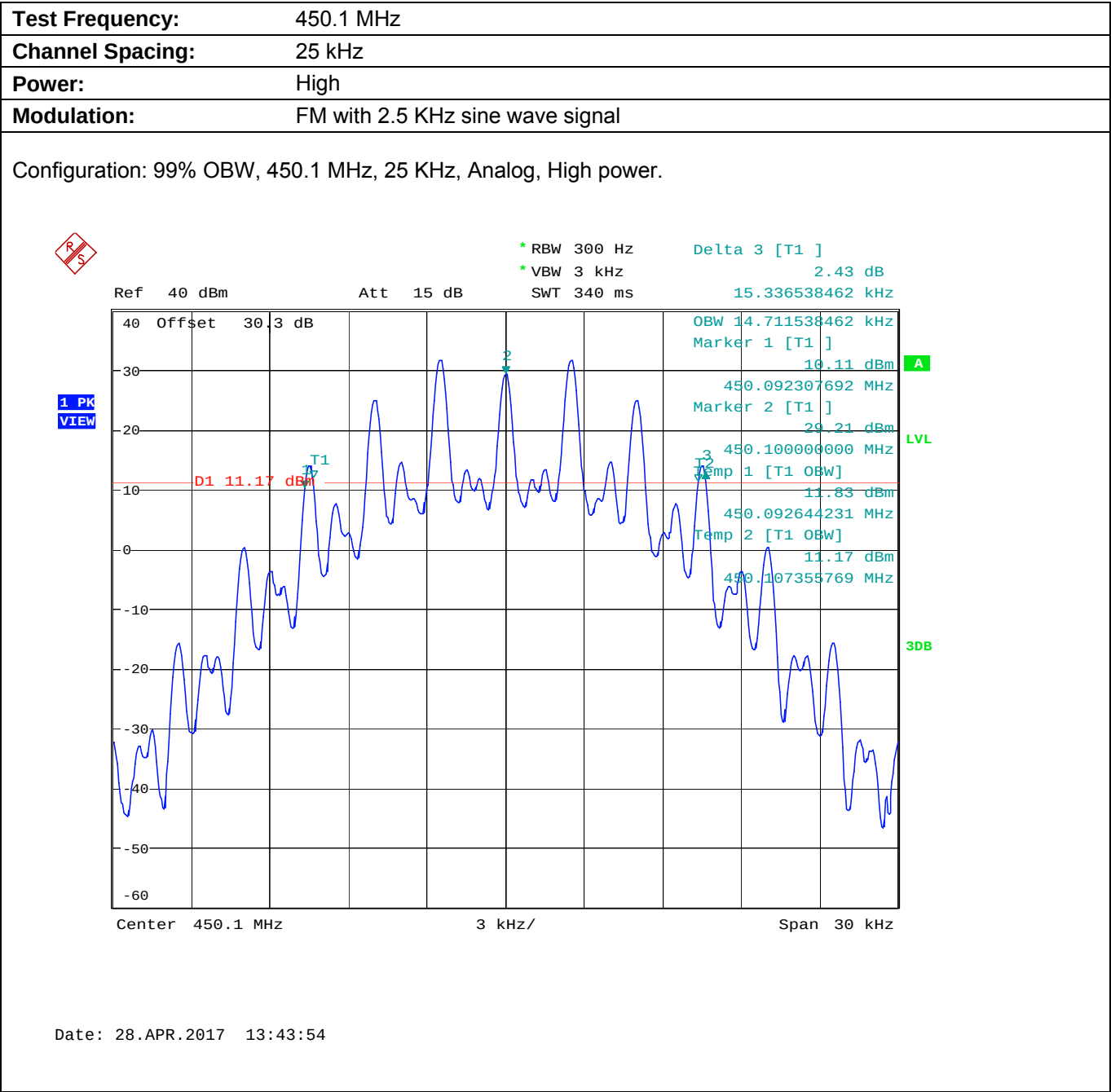
Plot 5.8.4.1.2. Occupied Bandwidth
