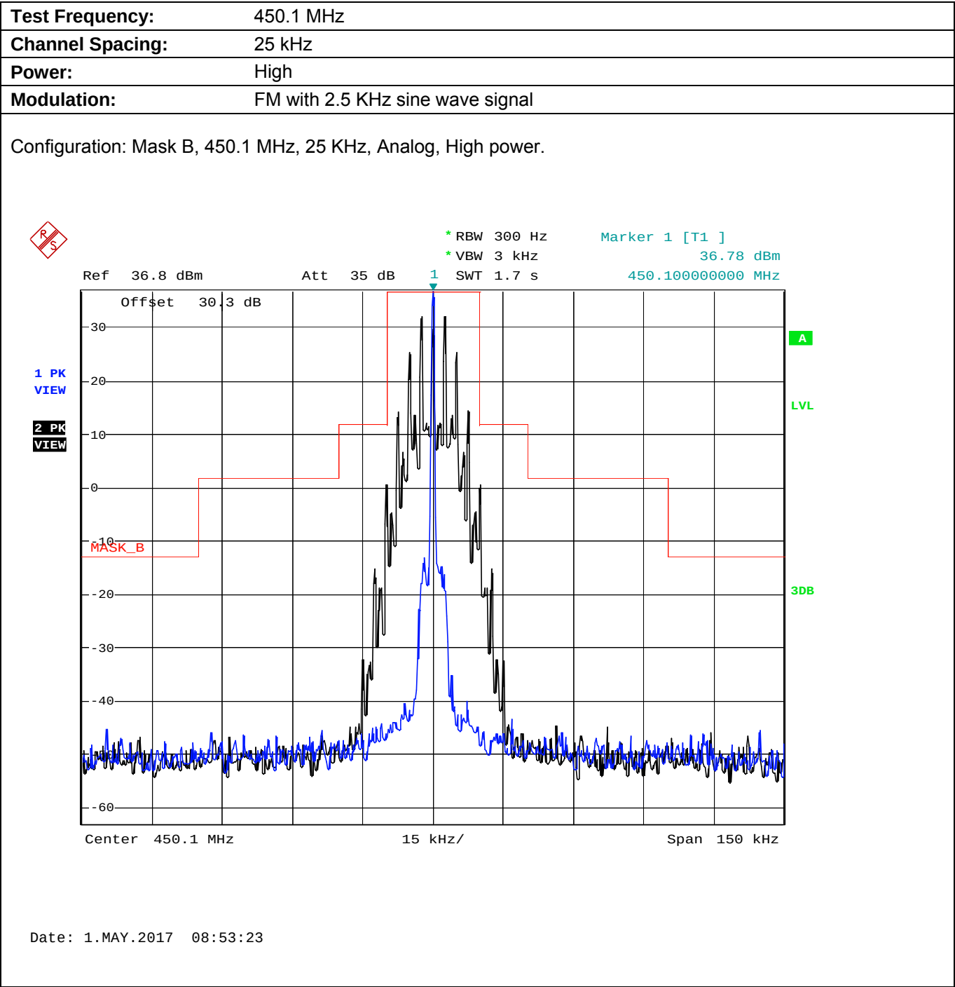
Plot 5.8.4.3.2. Emission Mask B, High Power
