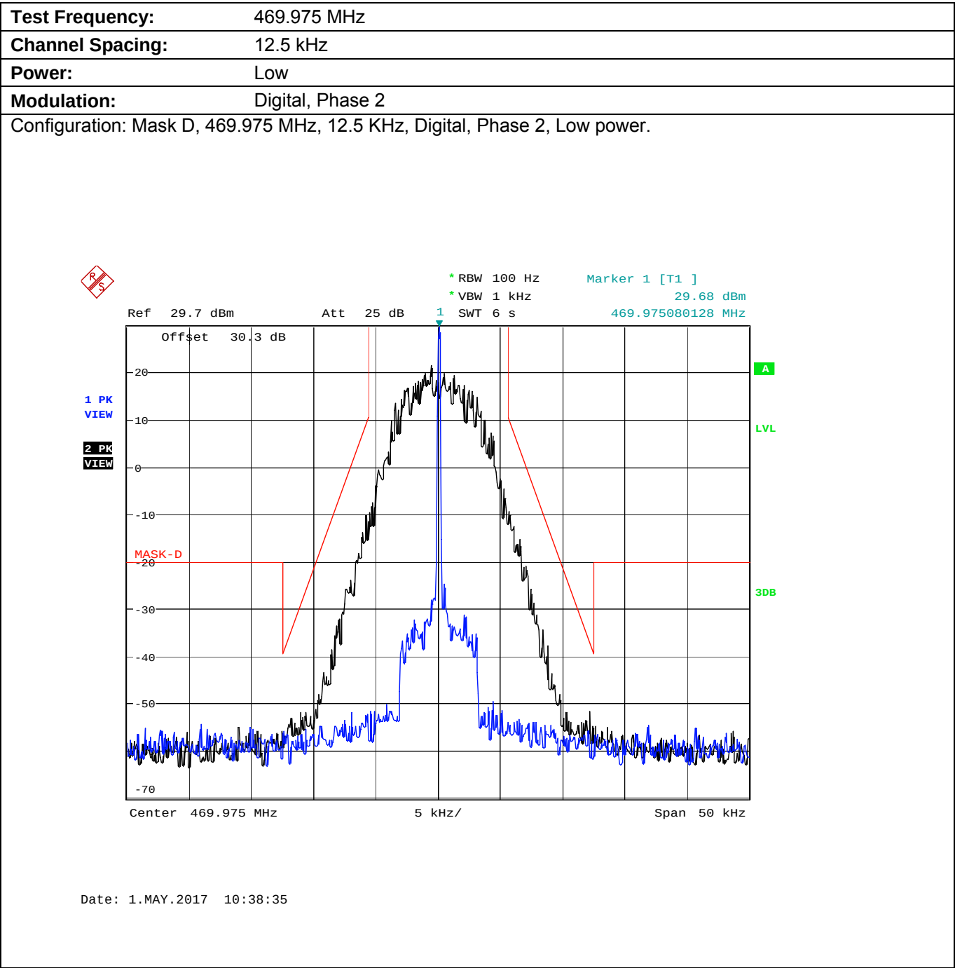
Plot 5.8.4.2.18. Emission Mask D, Low Power
