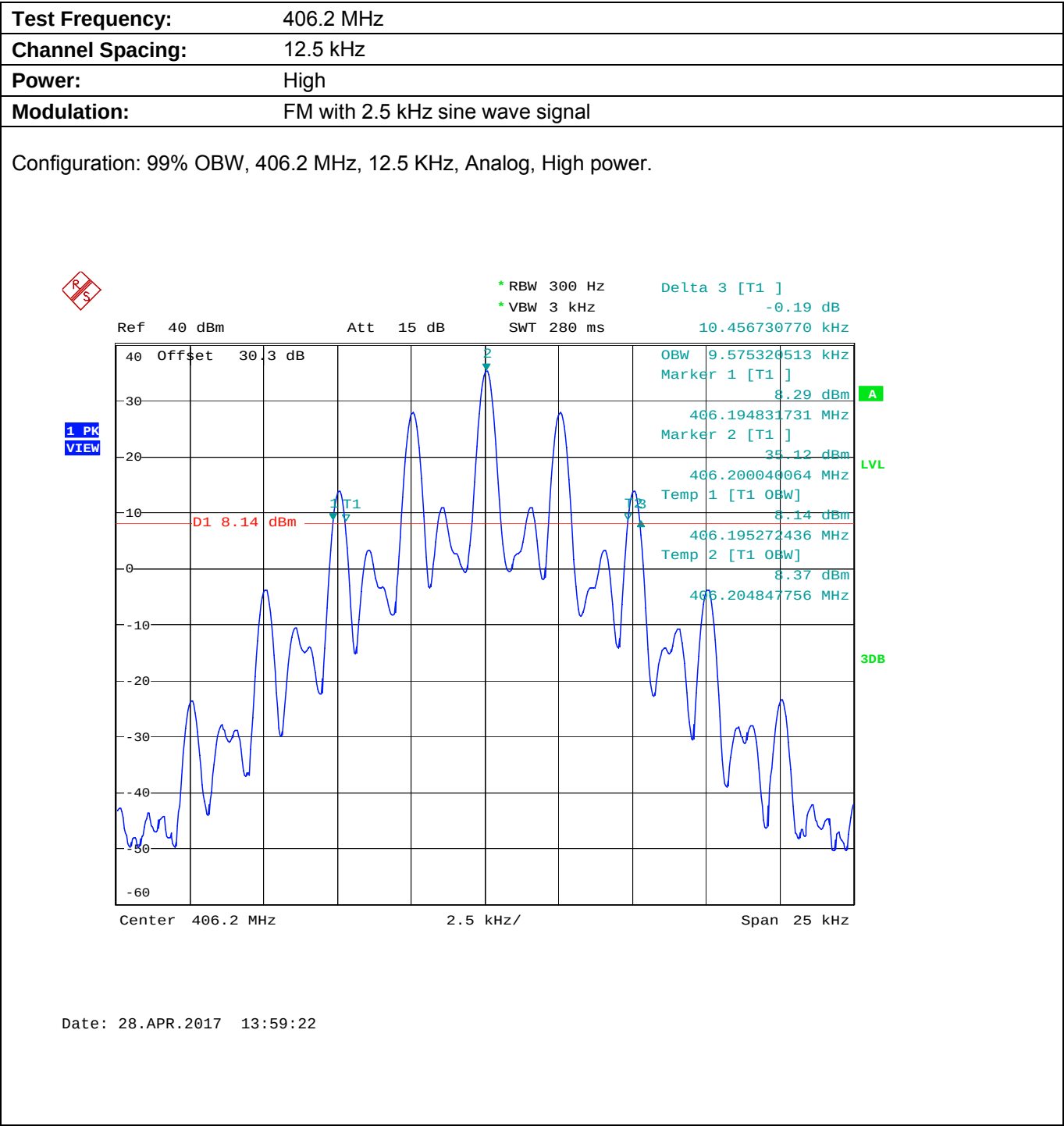
Plot 5.8.4.1.4. Occupied Bandwidth
