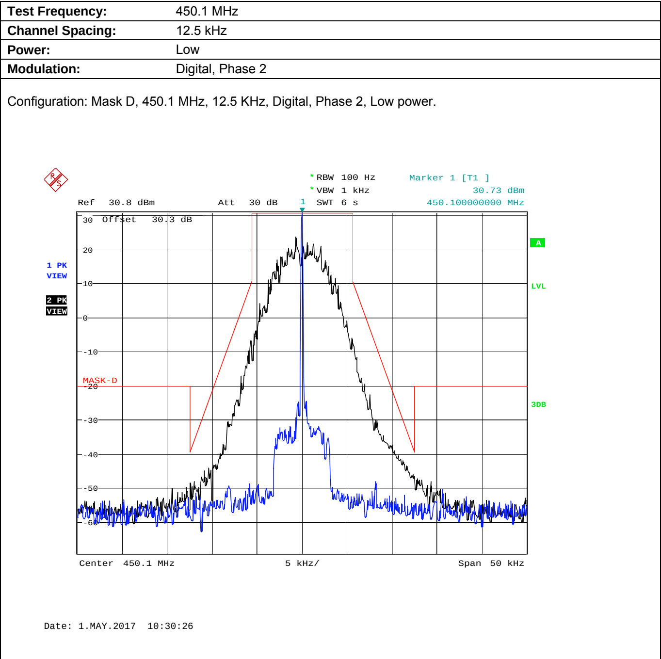
Plot 5.8.4.2.17. Emission Mask D, Low Power
