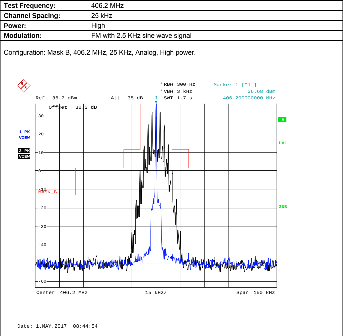
Plot 5.8.4.3.1. Emission Mask B, High Power
