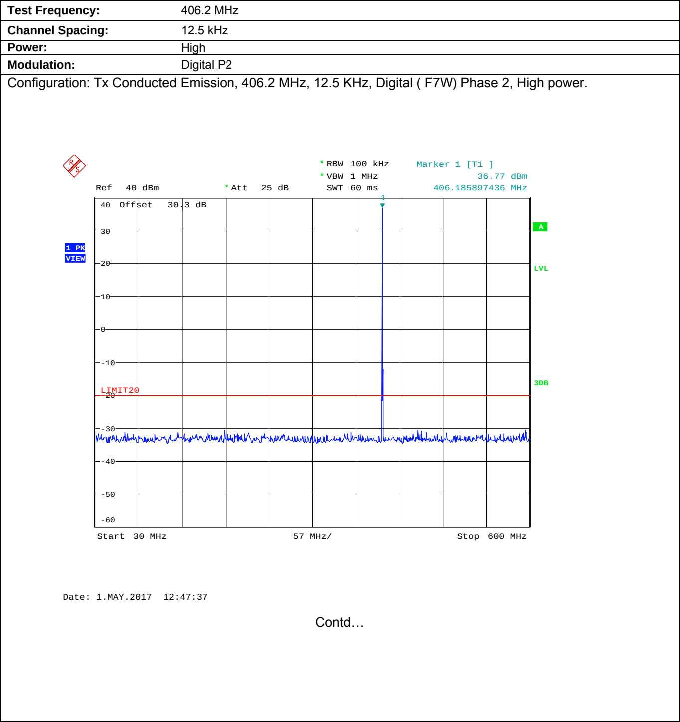
Plot 5.9.4.1.1. Conducted Transmitter Spurious Emissions for 406.2 MHz, High Power,
