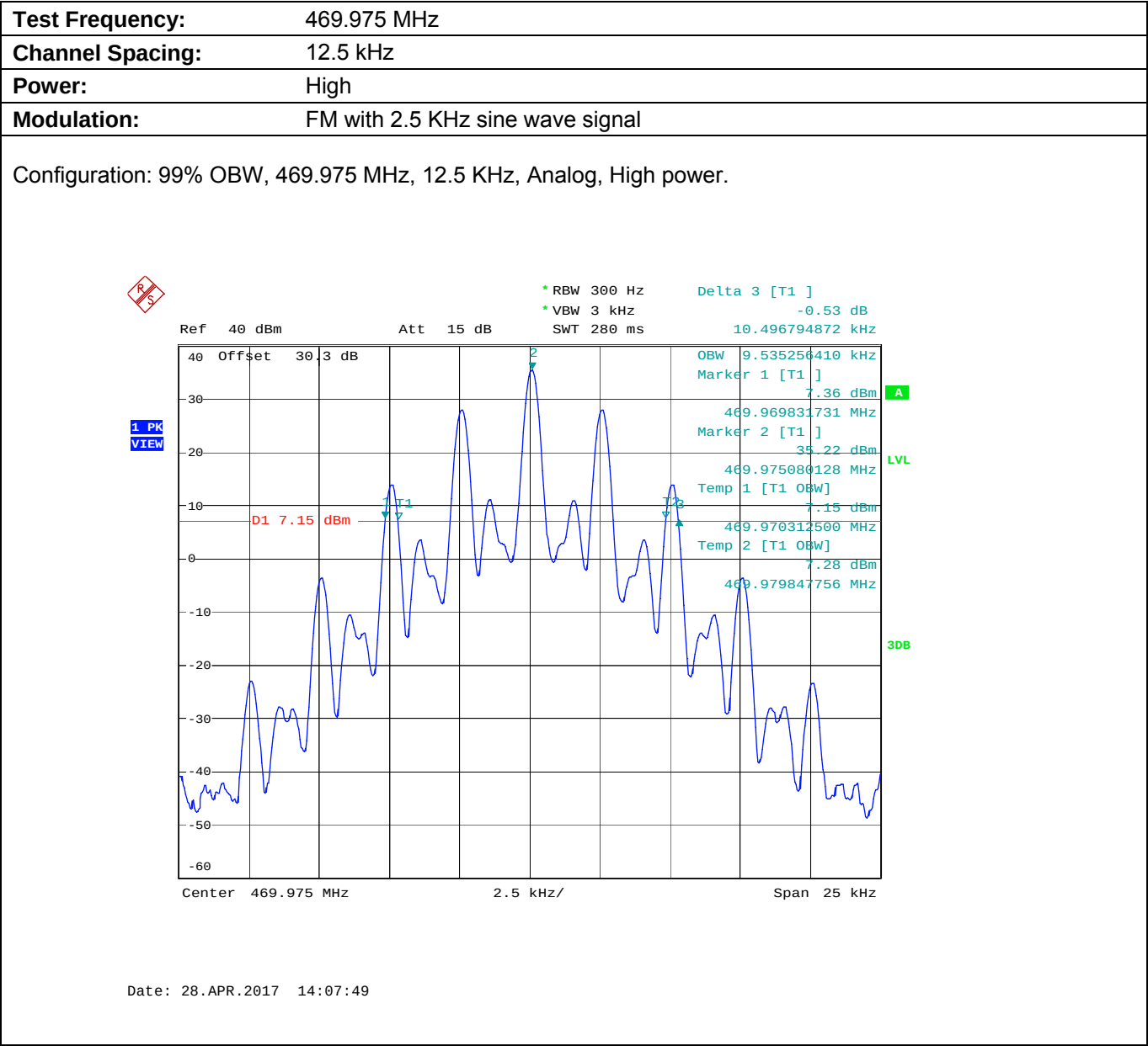
Plot 5.8.4.1.6. Occupied Bandwidth
