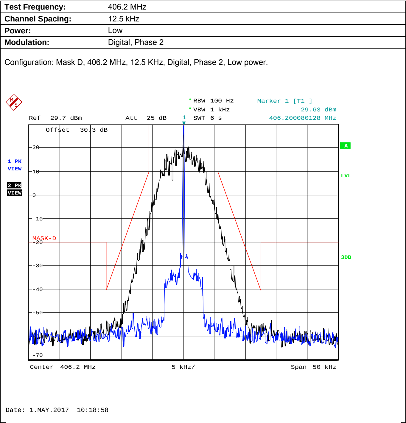
Plot 5.8.4.2.16. Emission Mask D, Low Power
