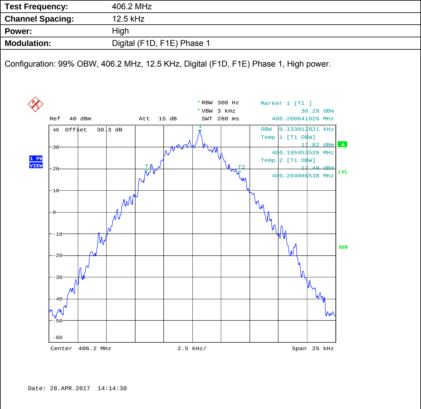
Plot 5.8.4.1.7. Occupied Bandwidth
