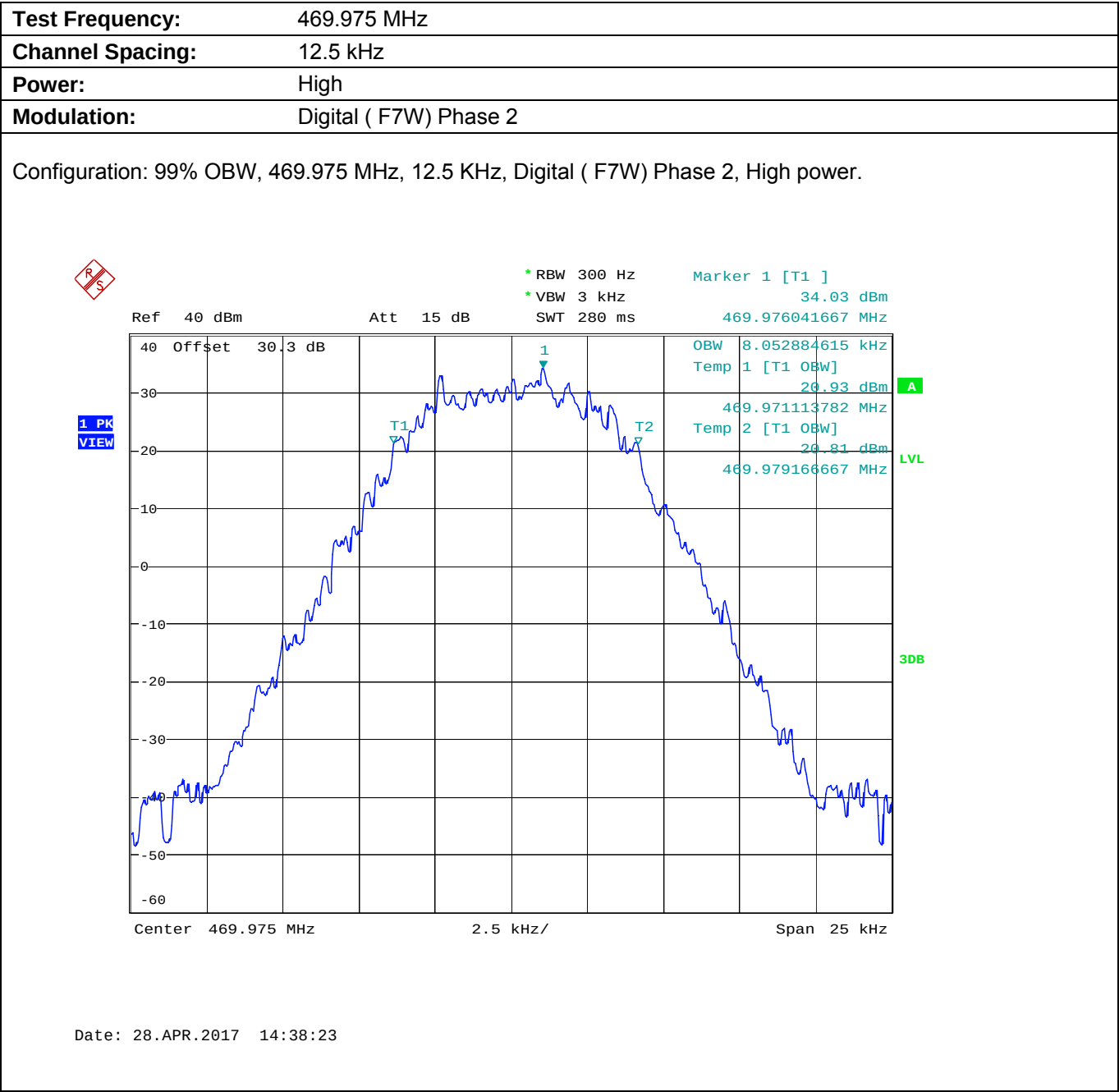
Plot 5.8.4.1.12. Occupied Bandwidth
