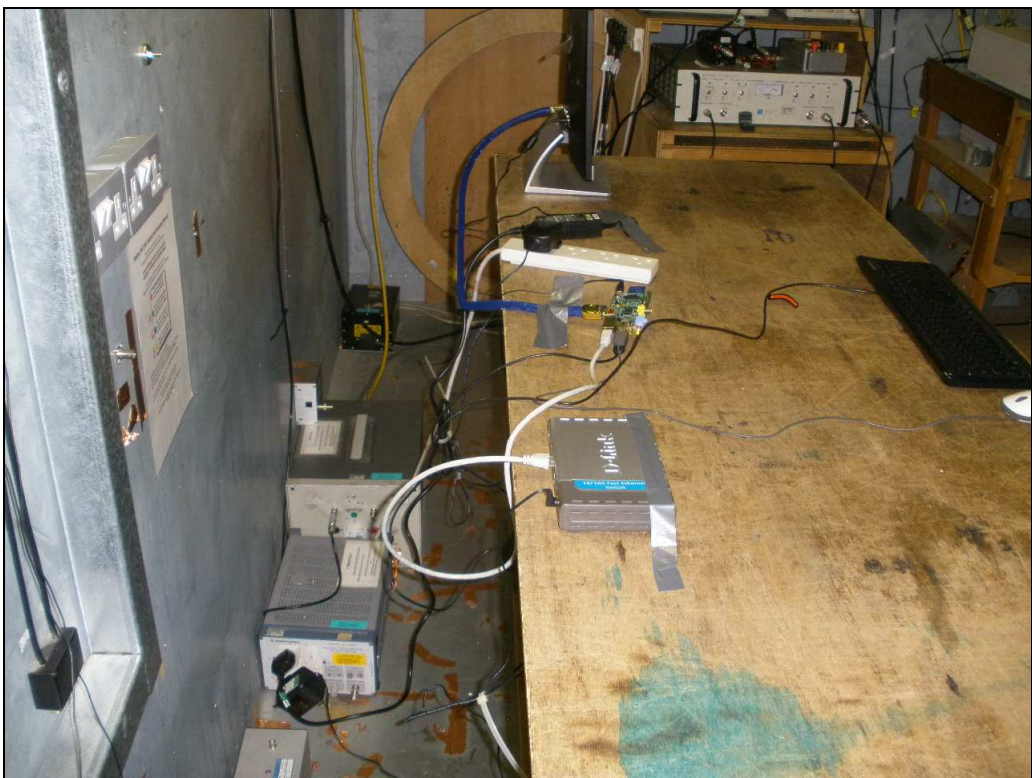
Photograph 2 Conducted Emissions - Back, HDMI
