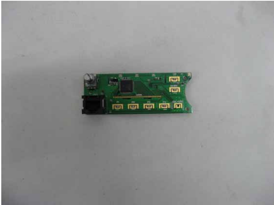
Internal View of Front Panel-2
