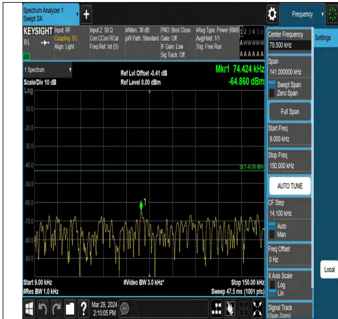
Band25_3MHz_QPSK_26365_1RB#0_0.009~0.15_0.009~0.1
