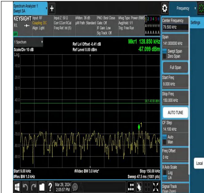
Band25_1.4MHz_QPSK_26047_1RB#0_0.009~0.15_0.009~0.15
