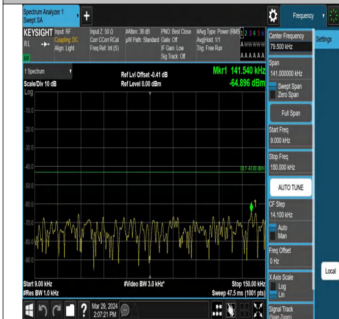
Band25_1.4MHz_QPSK_26683_1RB#0_0.009~0.15_0.009~0.
