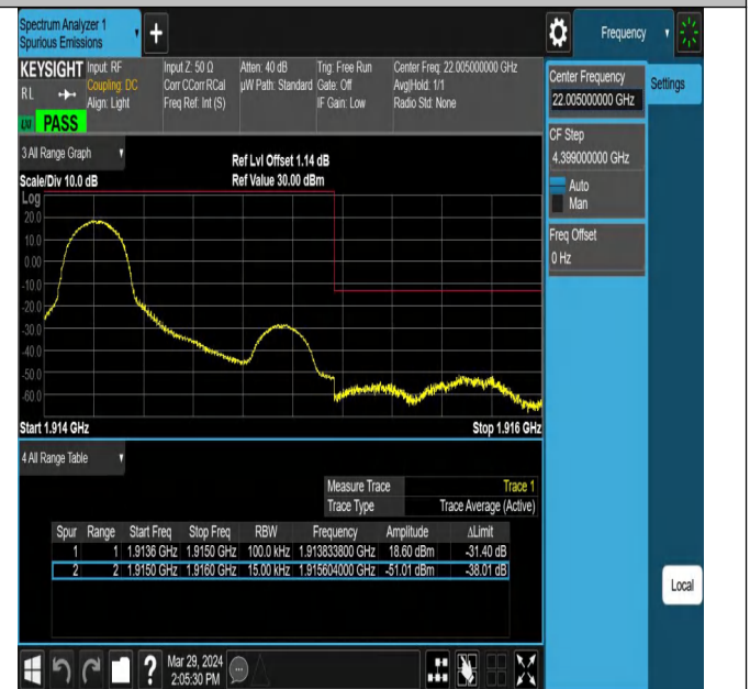
Band25_1.4MHz_QPSK_26683_1RB#0
