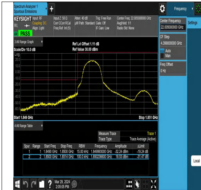
Band25_1.4MHz_QPSK_26047_1RB#0
