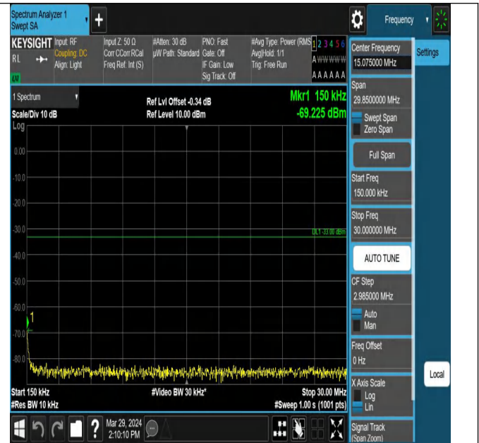
Band25_3MHz_QPSK_26365_1RB#0_0.15~30_0.15~30
