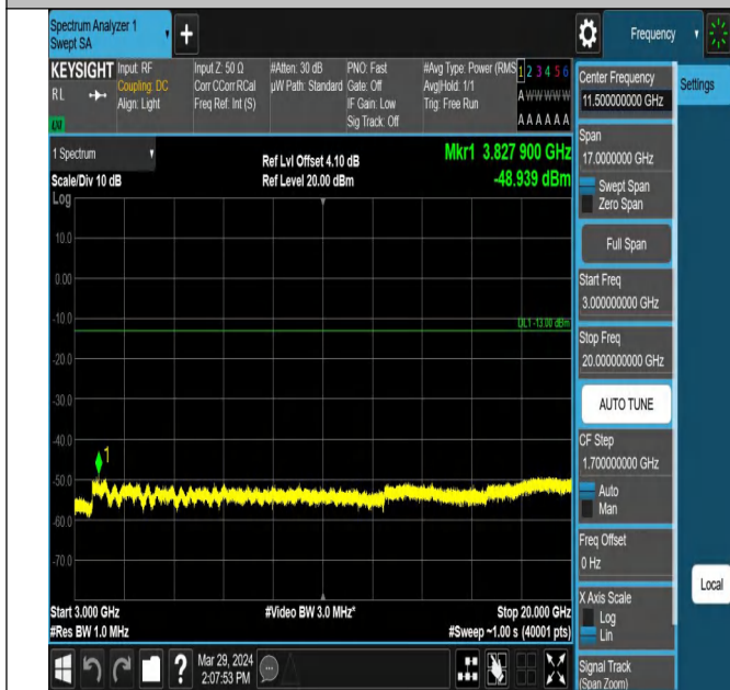
Band25_1.4MHz_QPSK_26683_1RB#0_3000~20000_3000~20000 0000
