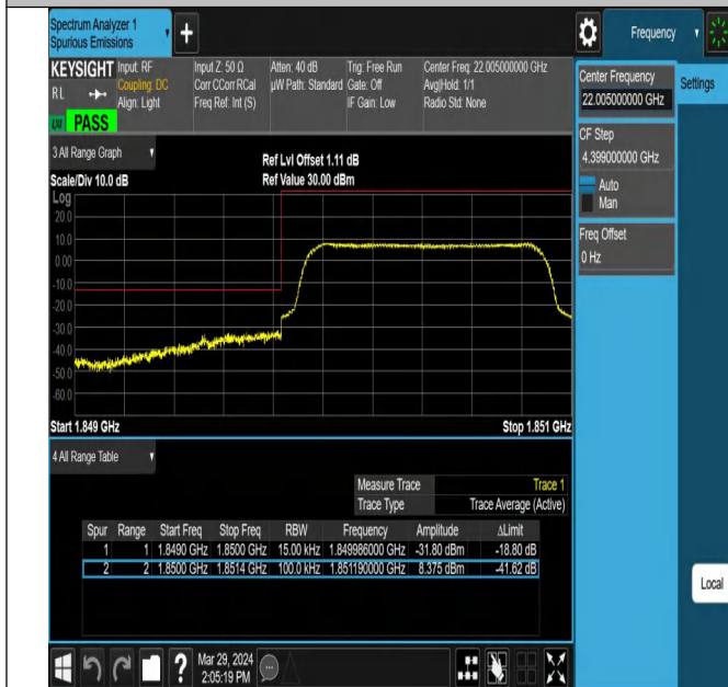
Band25_1.4MHz_QPSK_26047_6RB#0
