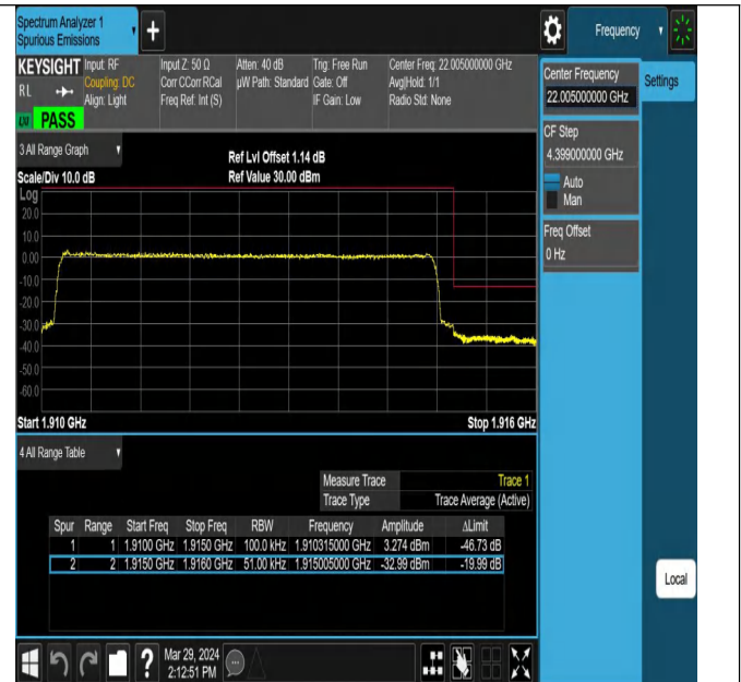
Band25_5MHz_QPSK_26665_25RB#0
