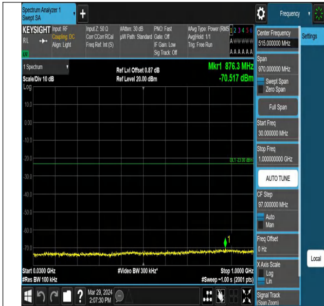
Band25_1.4MHz_QPSK_26683_1RB#0_30~1000_30~1000
