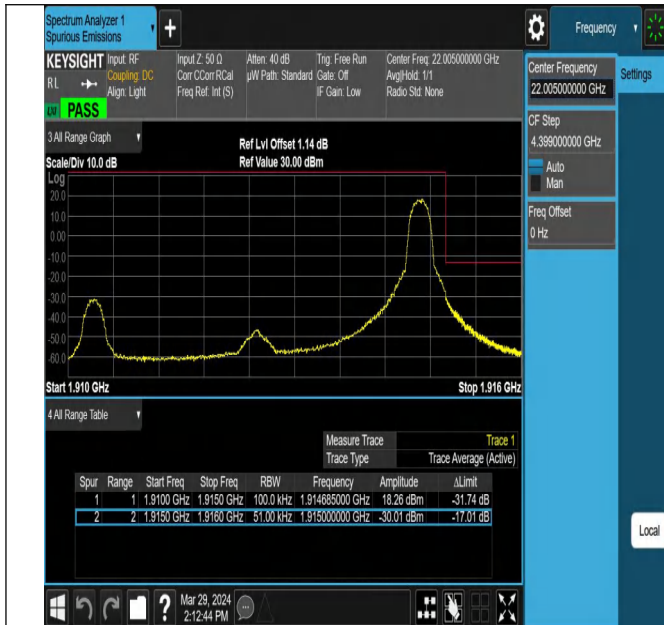
Band25_5MHz_QPSK_26665_1RB#24
