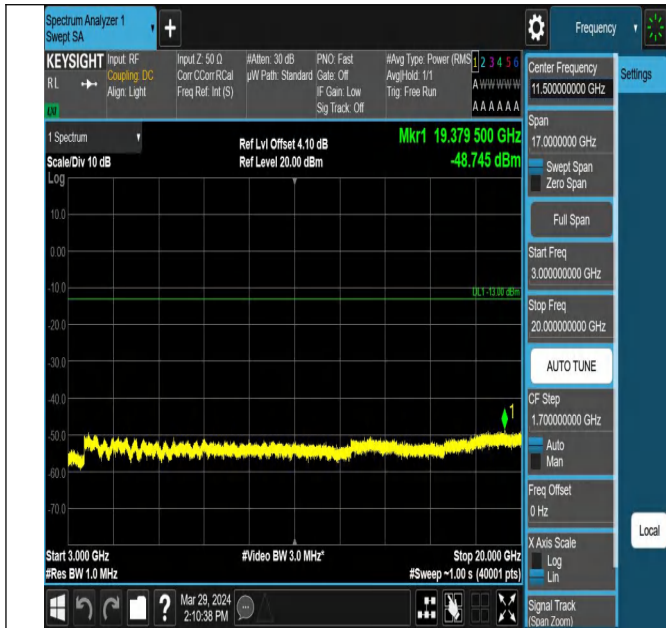
Band25_3MHz_QPSK_26365_1RB#0_3000~20000_3000~20000
