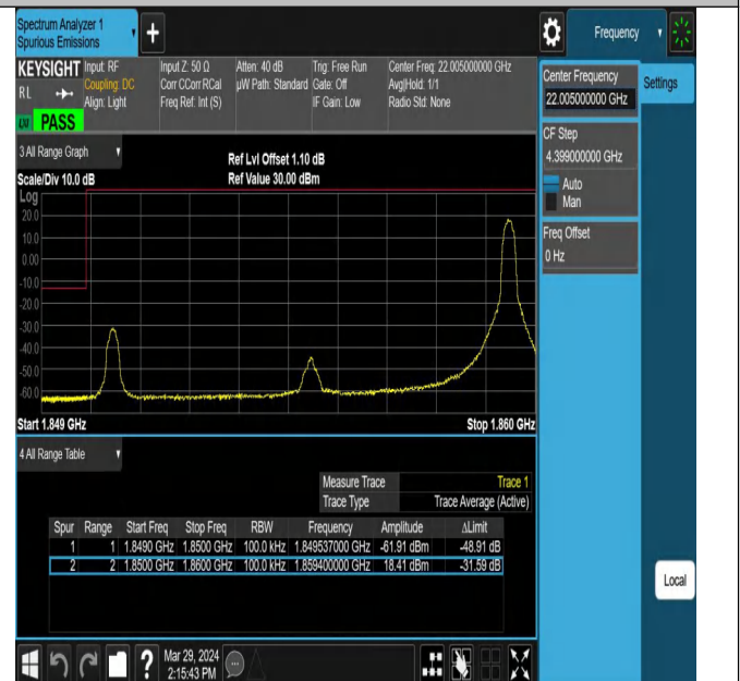
Band25_10MHz_QPSK_26090_1RB#49
