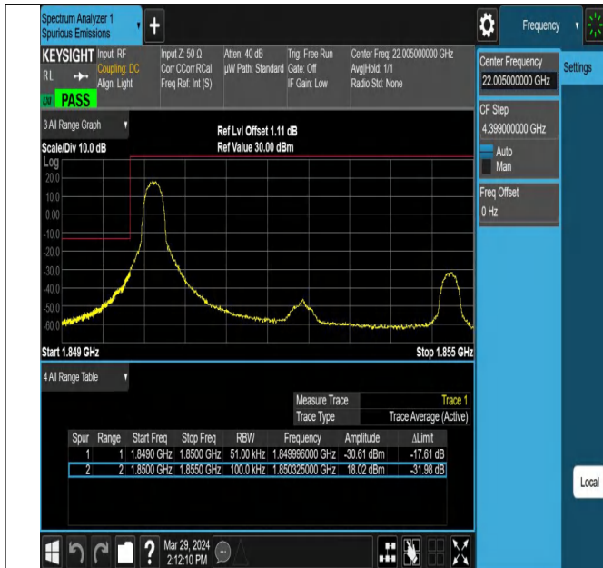
Band25_5MHz_QPSK_26065_1RB#0
