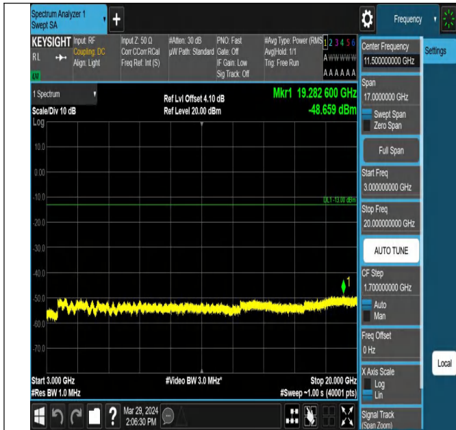
Band25_1.4MHz_QPSK_26047_1RB#0_3000~20000_3000~20000 0000
