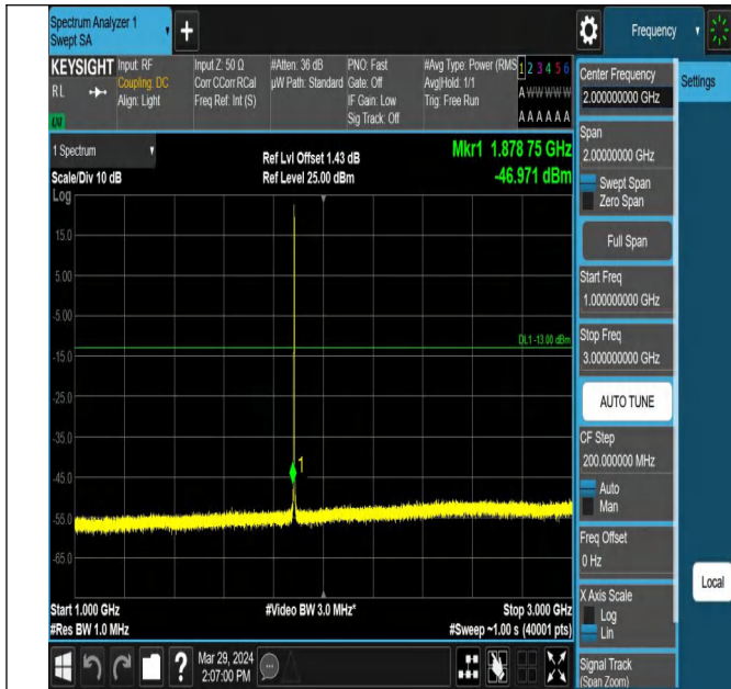
Band25_1.4MHz_QPSK_26365_1RB#0_1000~3000_1000~30
