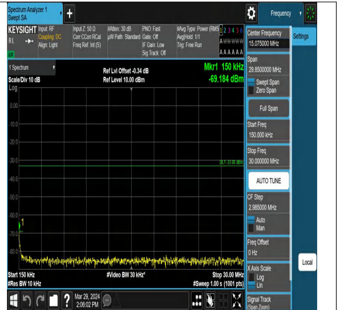
Band25_1.4MHz_QPSK_26047_1RB#0_0.15~30_0.15~30
