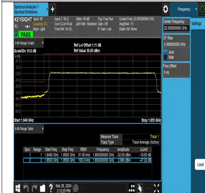
Band25_5MHz_QPSK_26065_25RB#0
