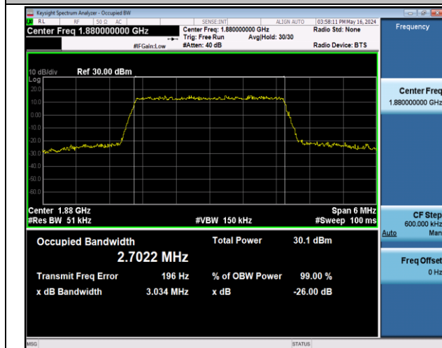
Band2-3MHz-16QAM-18900-15RB#0-PASS
