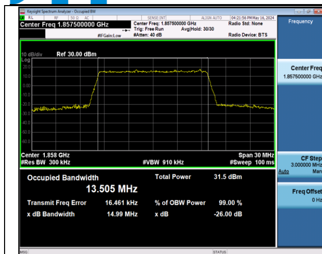
Band2-15MHz-QPSK-18675-75RB#0-PASS
