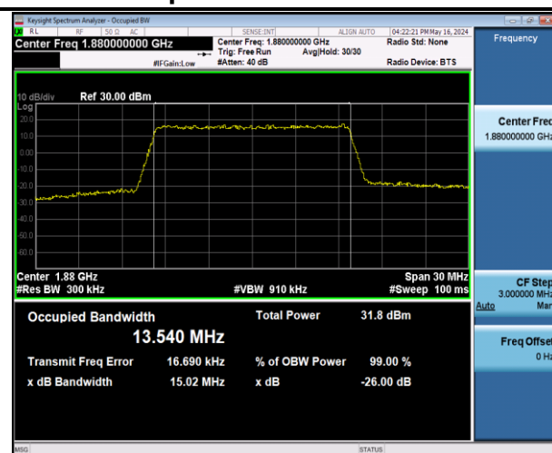
Band2-15MHz-QPSK-18900-75RB#0-PASS
