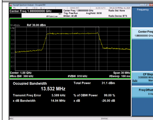
Band2-15MHz-16QAM-18900-75RB#0-PASS
