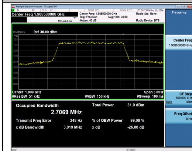
Band2-3MHz-QPSK-19185-15RB#0-PASS
