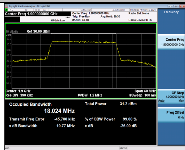
Band2-20MHz-16QAM-19100-100RB#0-PASS
