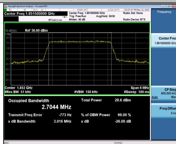
Band2-3MHz-16QAM-18615-15RB#0-PASS
