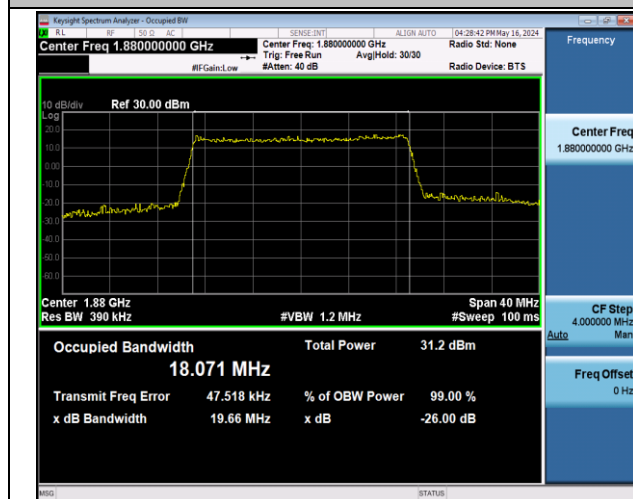
Band2-20MHz-16QAM-18900-100RB#0-PASS
