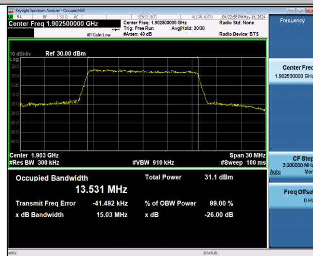
Band2-15MHz-16QAM-19125-75RB#0-PASS
