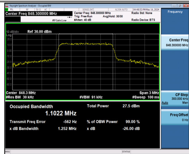
Band5-1.4MHz-16QAM-20643-6RB#0-PASS
