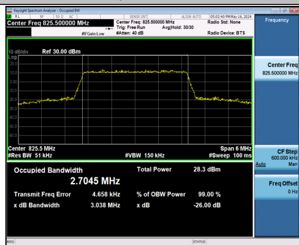
Band5-3MHz-16QAM-20415-15RB#0-PASS
