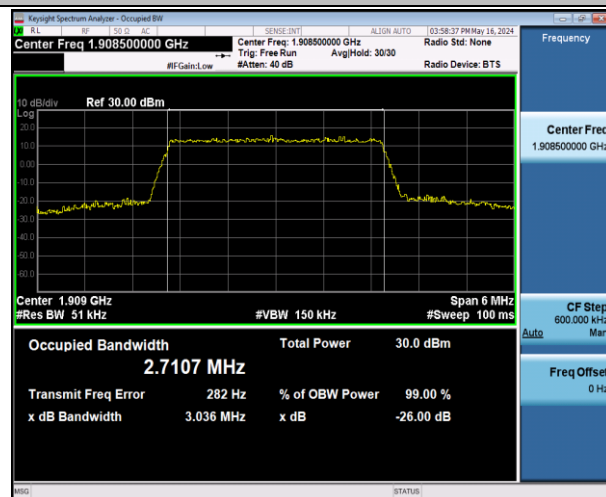
Band2-3MHz-16QAM-19185-15RB#0-PASS
