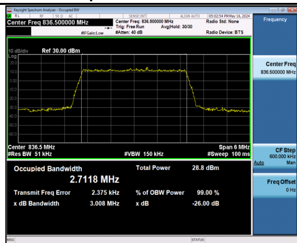
Band5-3MHz-QPSK-20525-15RB#0-PASS
