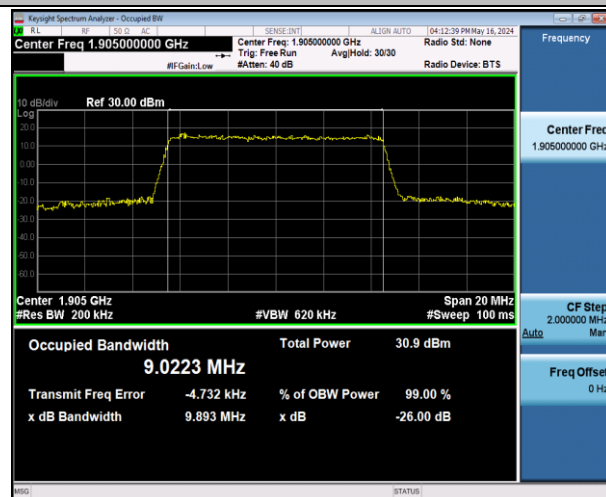
Band2-10MHz-16QAM-19150-50RB#0-PASS
