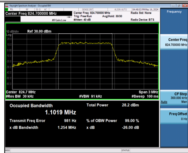
Band5-1.4MHz-16QAM-20407-6RB#0-PASS
