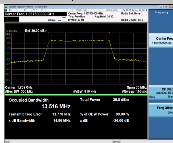
Band2-15MHz-16QAM-18675-75RB#0-PASS
