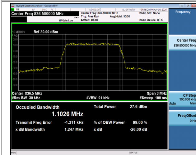
Band5-1.4MHz-16QAM-20525-6RB#0-PASS
