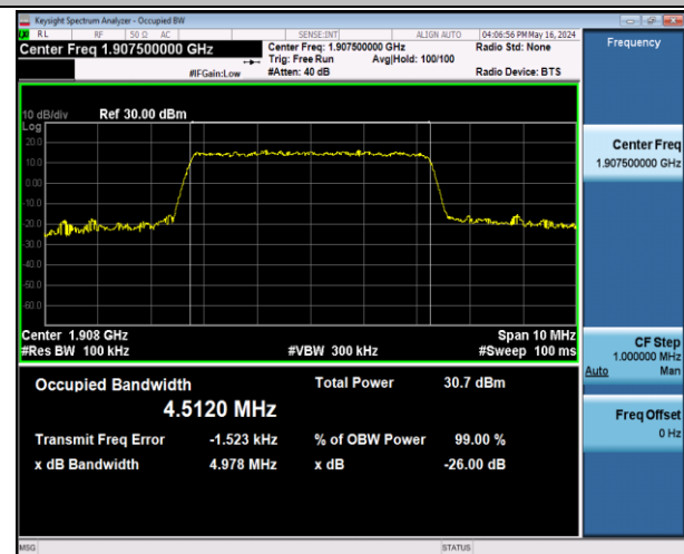
Band2-5MHz-16QAM-19175-25RB#0-PASS
