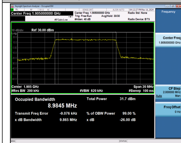
Band2-10MHz-QPSK-19150-50RB#0-PASS
