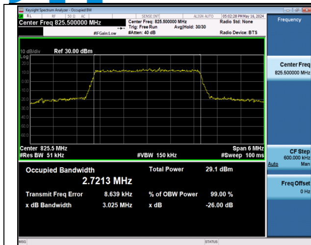
Band5-3MHz-QPSK-20415-15RB#0-PASS
