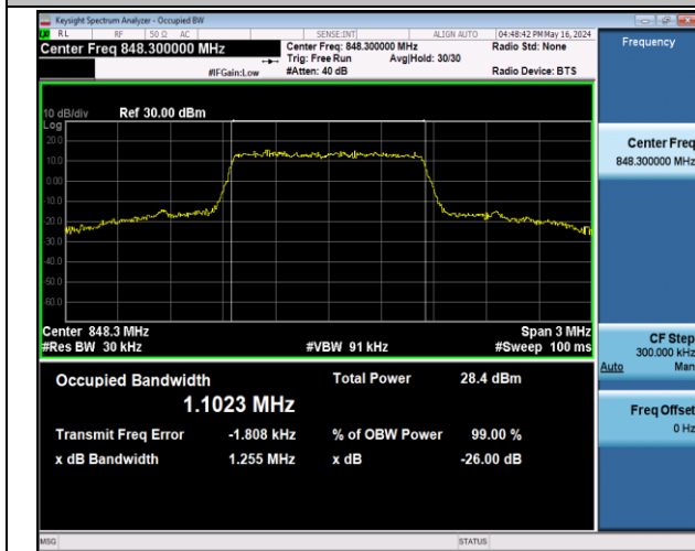
Band5-1.4MHz-QPSK-20643-6RB#0-PASS
