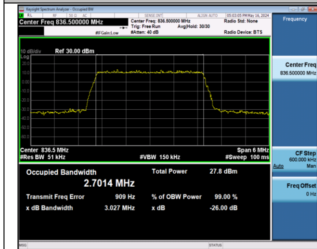
Band5-3MHz-16QAM-20525-15RB#0-PASS
