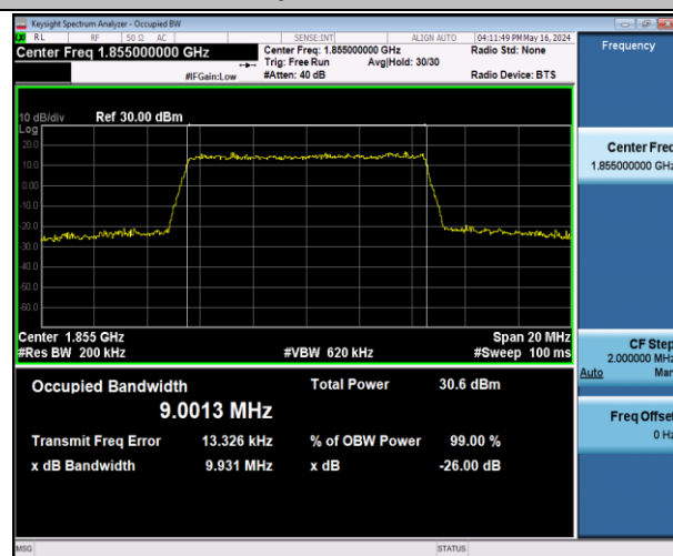
Band2-10MHz-16QAM-18650-50RB#0-PASS
