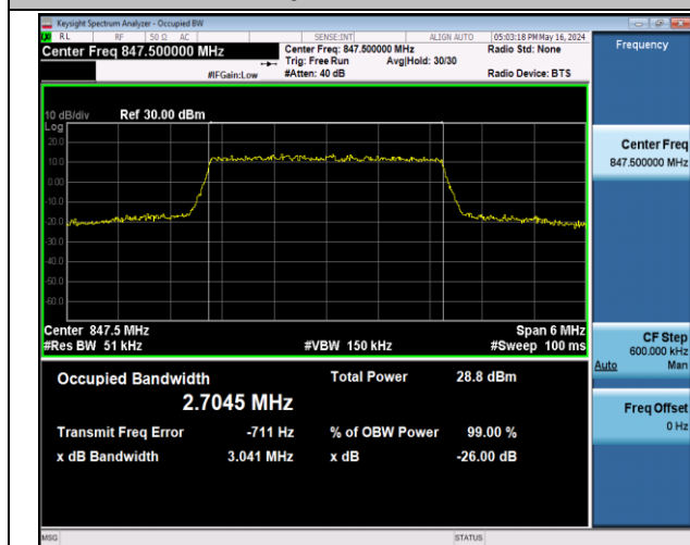
Band5-3MHz-QPSK-20635-15RB#0-PASS
