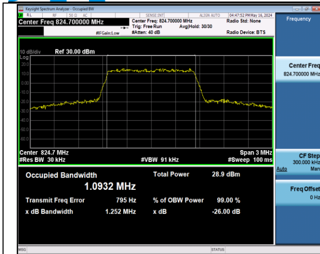
Band5-1.4MHz-QPSK-20407-6RB#0-PASS
