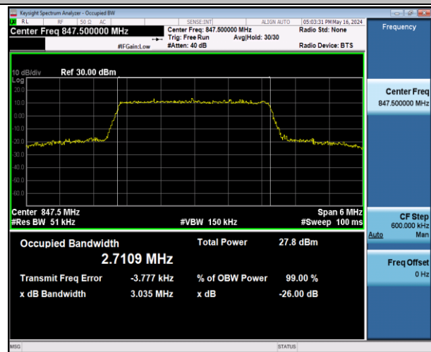
Band5-3MHz-16QAM-20635-15RB#0-PASS
