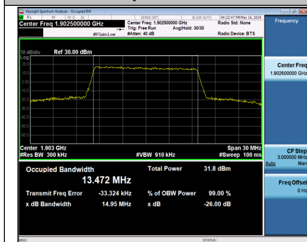
Band2-15MHz-QPSK-19125-75RB#0-PASS
