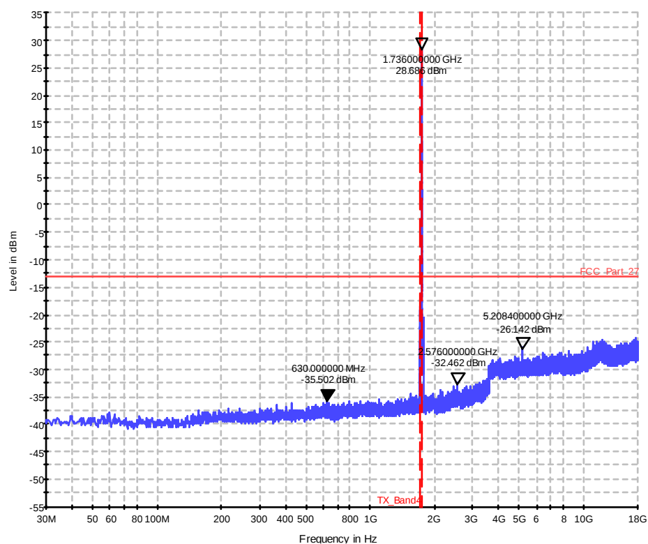
Diagram 36.45b_CSE_Ch20300_BW_20_1RB_low_16QAM_Sweep2
