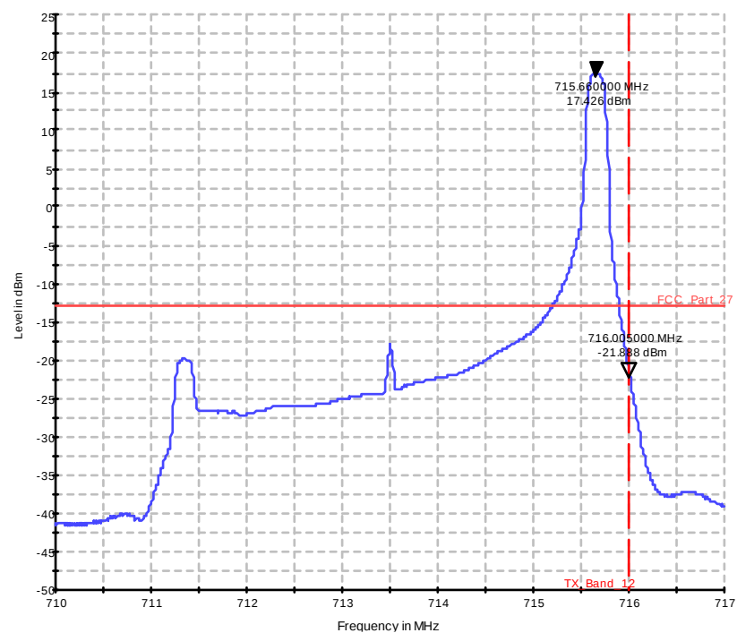
Diagram 37.1213b_Ch23155_BW_5_1RB_high_16QAM
