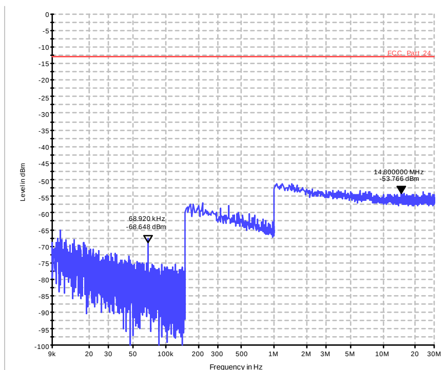
Diagram 36.1201b_Ch23060_BW_10_1RB_low_16QAM_Sweep1
