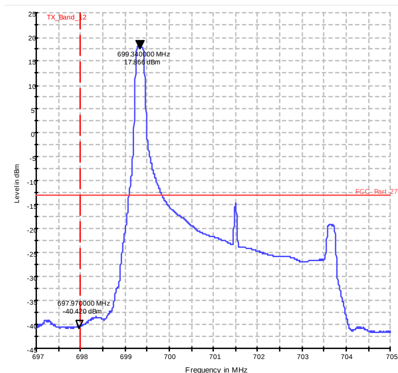
Diagram 37.1205a_Ch23035_BW_5_1RB_low_QPSK
