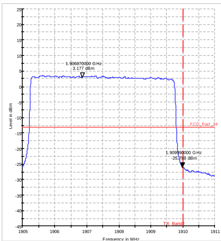
Diagram 37.218b_ch19175_25RB_high_QAM
