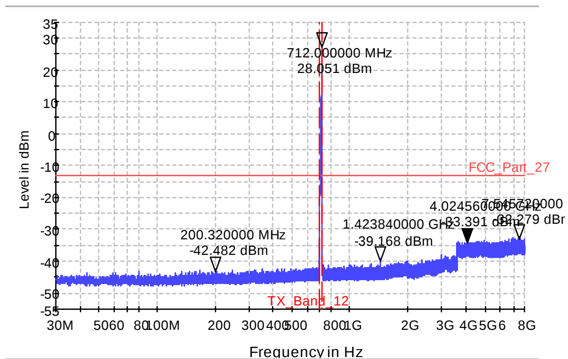
Diagram 36.1204a_Ch23095_BW_10_1RB_high_QPSK_Sweep2
