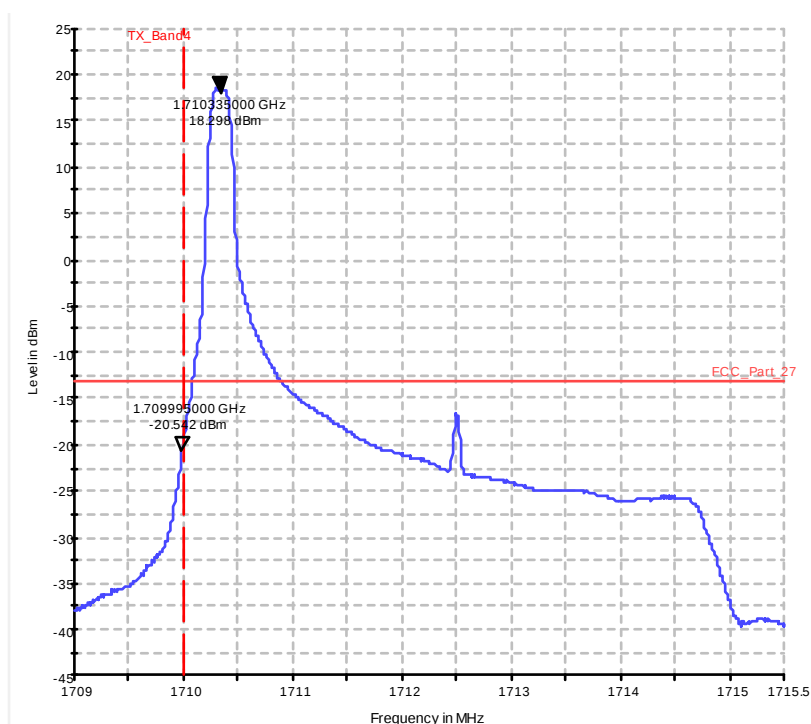
Diagram 37.405b_Ch19975_BW_5_1RB_low_16QAM
