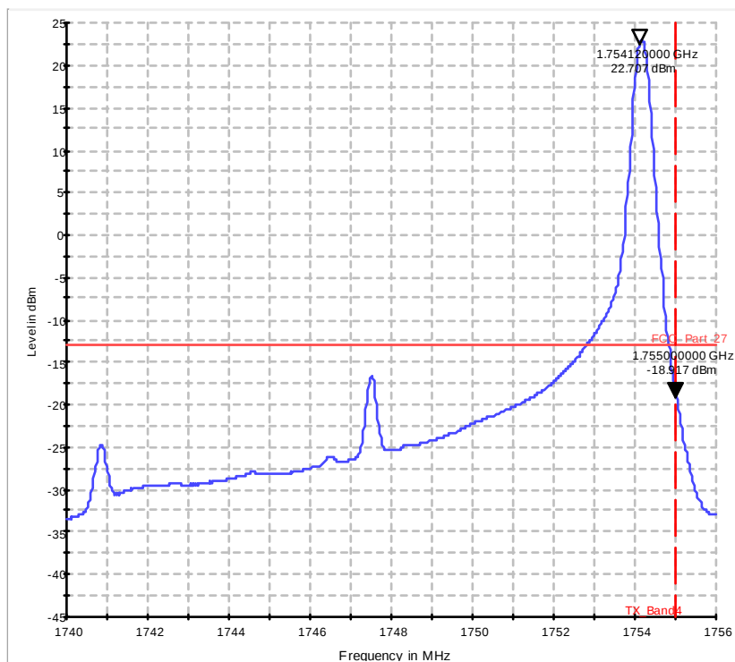
Diagram 37.421a_Ch20325_BW_15_1RB_high_QPSK
