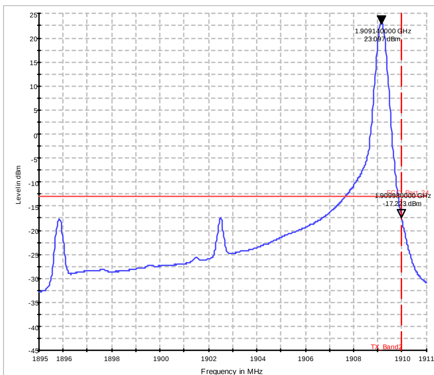
Diagram 37.221a_ch19125_1RB_high_QPSK
