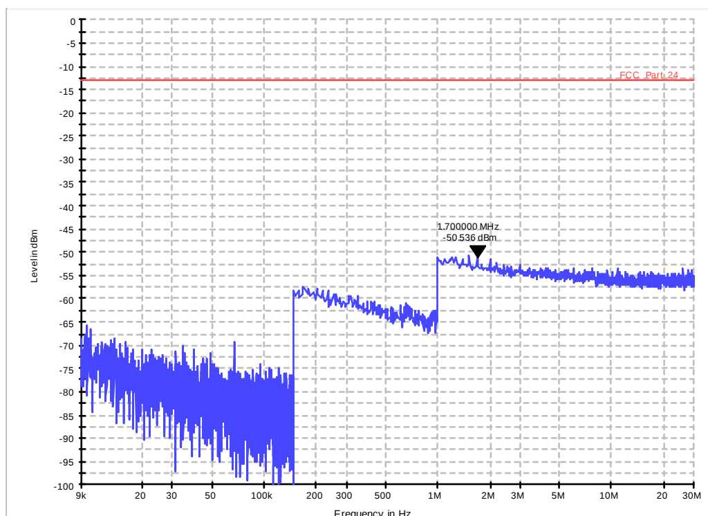
Diagram 36.1205b_Ch23155_BW_5_1RB_high_16QAM_Sweep1
