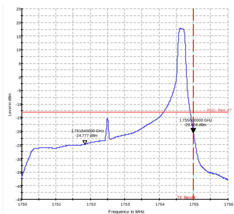
Diagram 37.417b_Ch20375_BW_5_1RB_high_16QAM
