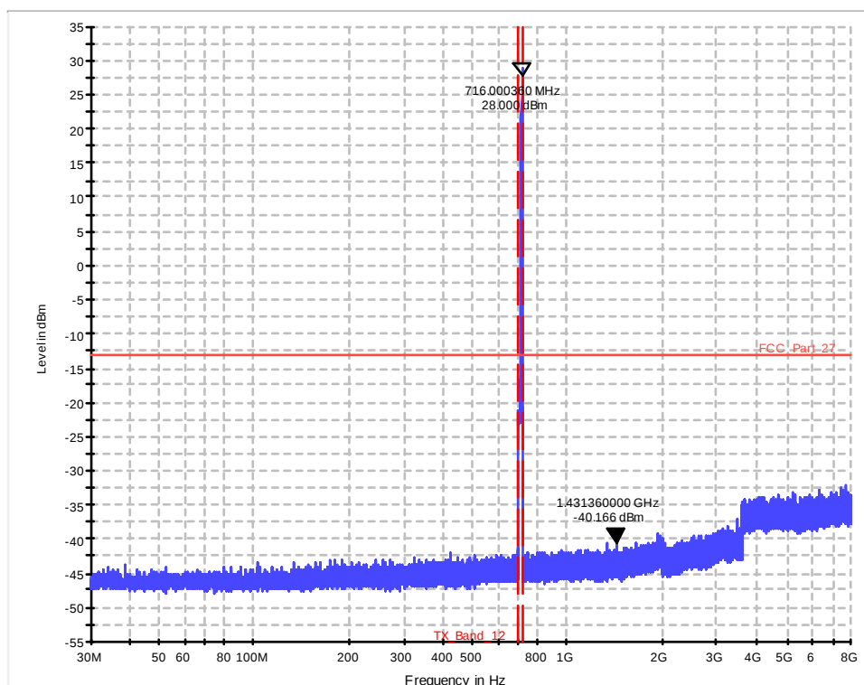
Diagram 36.1206a_Ch23155_BW_5_1RB_high_QPSK_Sweep2
