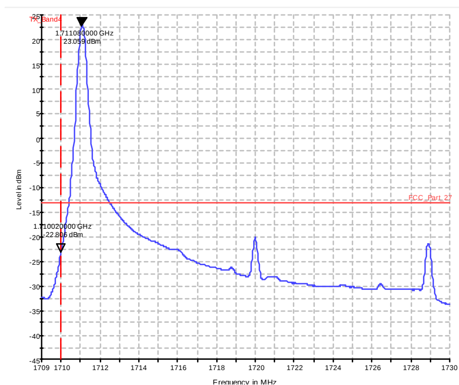
Diagram 37.411b_Ch20050_BW_20_1RB_low_16QAM
