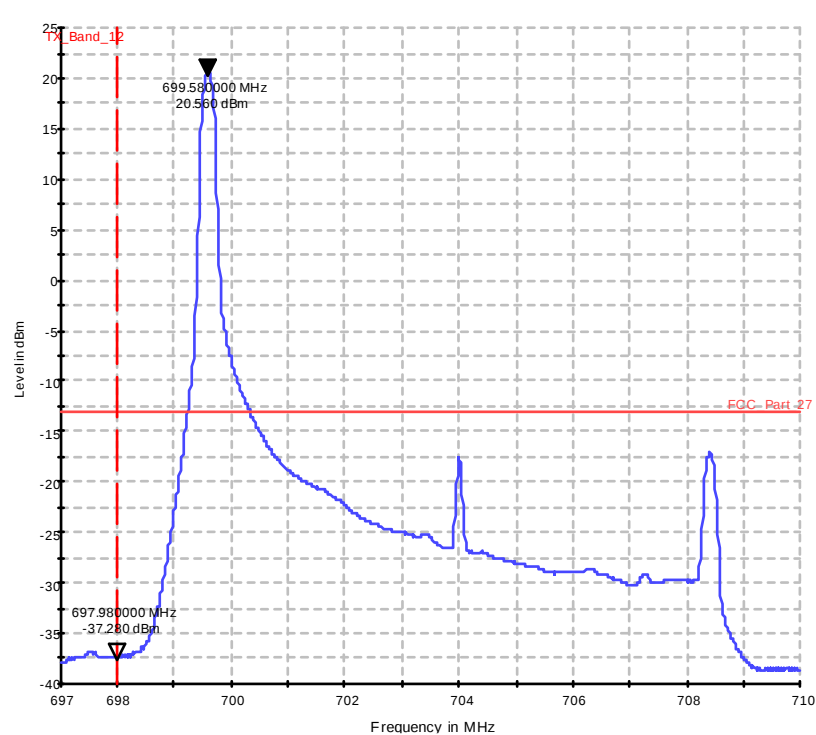
Diagram 37.1207b_Ch23060_BW_10_1RB_low_16QAM
