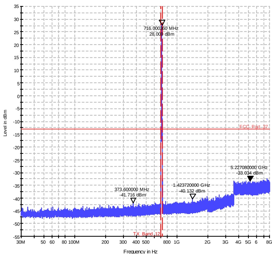
Diagram 36.1204b_Ch23095_BW_10_1RB_high_16QAM_Sweep2
