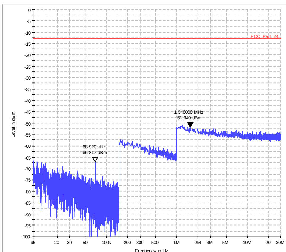
Diagram 36.1205a_Ch23155_BW_5_1RB_high_QPSK_Sweep1
