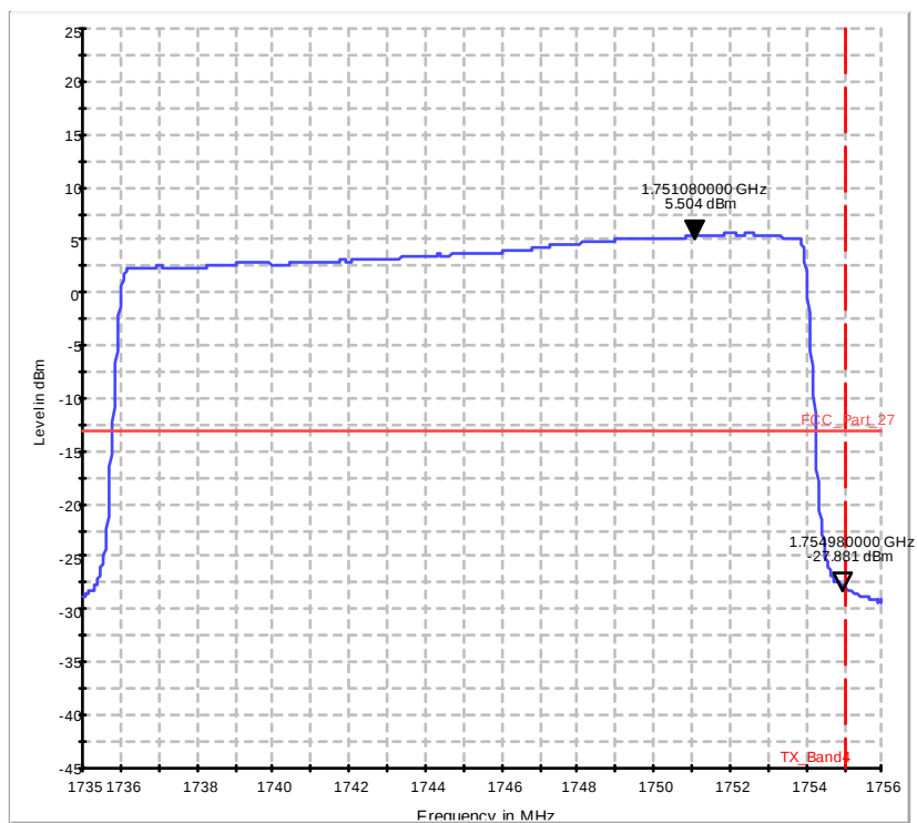
Diagram 37.424a_Ch20300_BW_20_100RBs_QPSK
