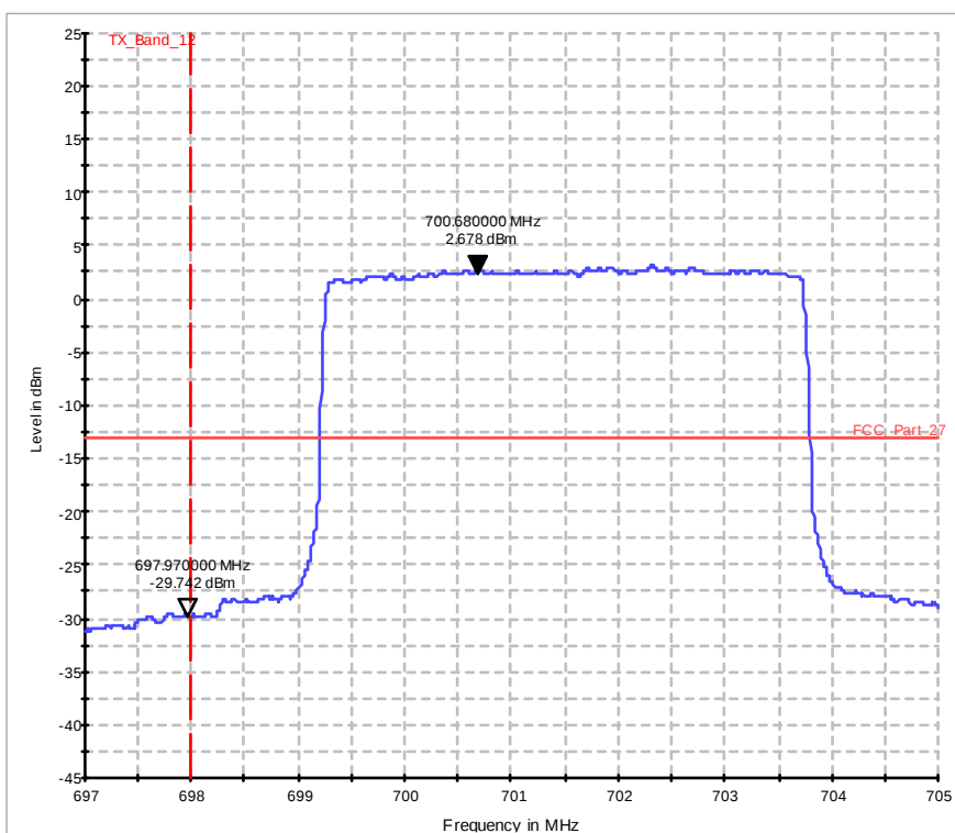
Diagram 37.1206b_Ch23035_BW_5_25RBs_16QAM
