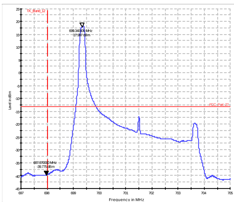
Diagram 37.1205b_Ch23035_BW_5_1RB_low_16QAM
