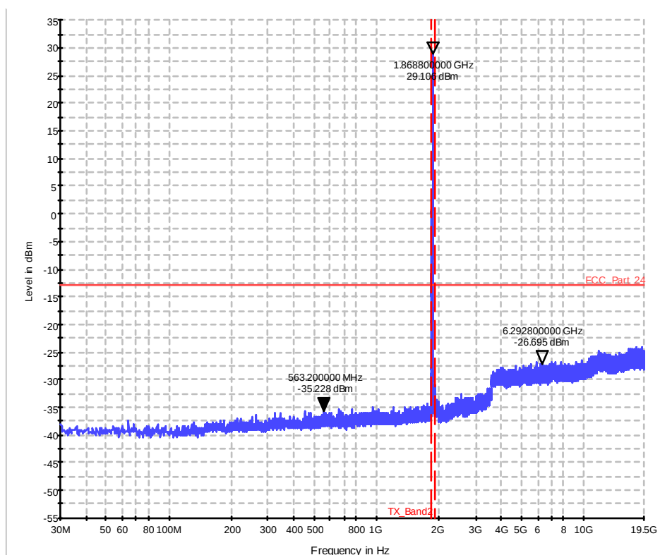
Diagram 36.21a_CSE_Ch18700_BW_20_1RB_high_QPSK_Sweep2
