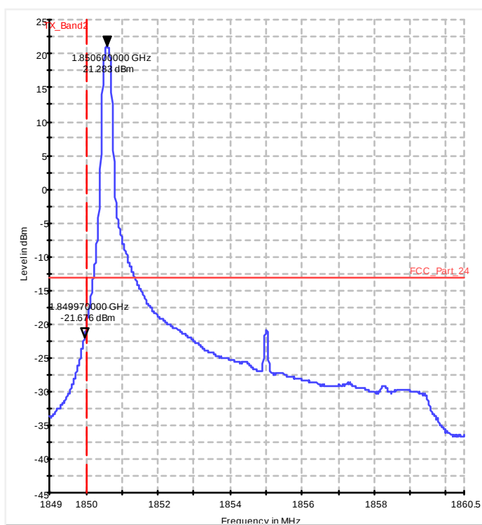
Diagram 37.207b_ch18650_1RB_QAM
