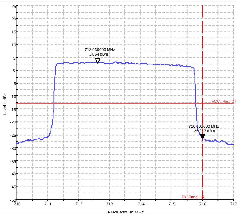
Diagram 37.1214b_Ch23155_BW_5_25RBs_16QAM
