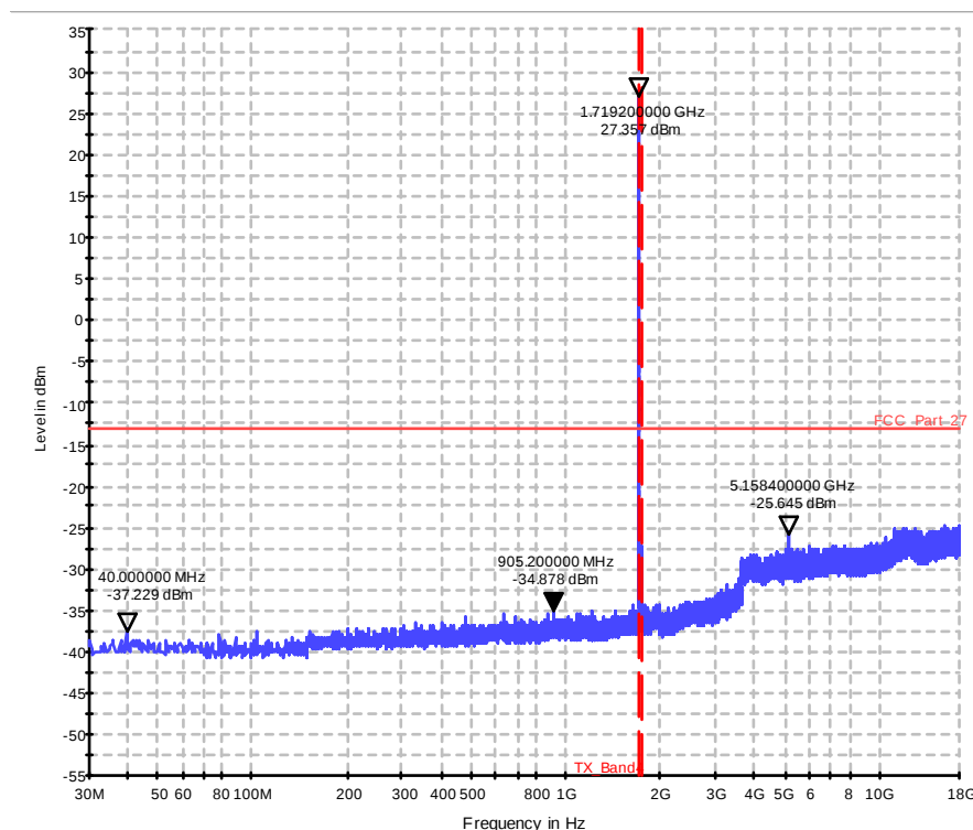
Diagram 36.41a_CSE_Ch2000_BW_10_1RB_high_QPSK_Sweep2
