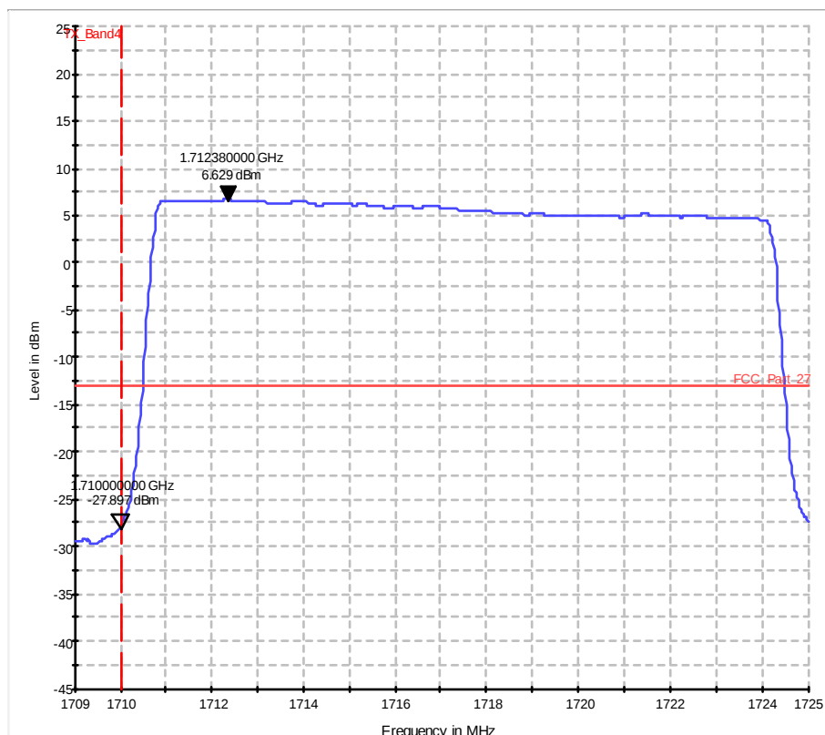
Diagram 37.410a_Ch20025_BW_15_75RBs_QPSK
