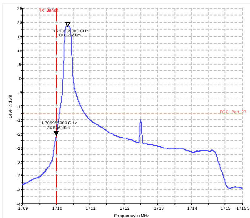
Diagram 37.405a_Ch19975_BW_5_1RB_low_QPSK
