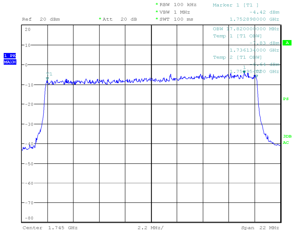
Diagram 35.417 BW 20MHz Ch_20175
