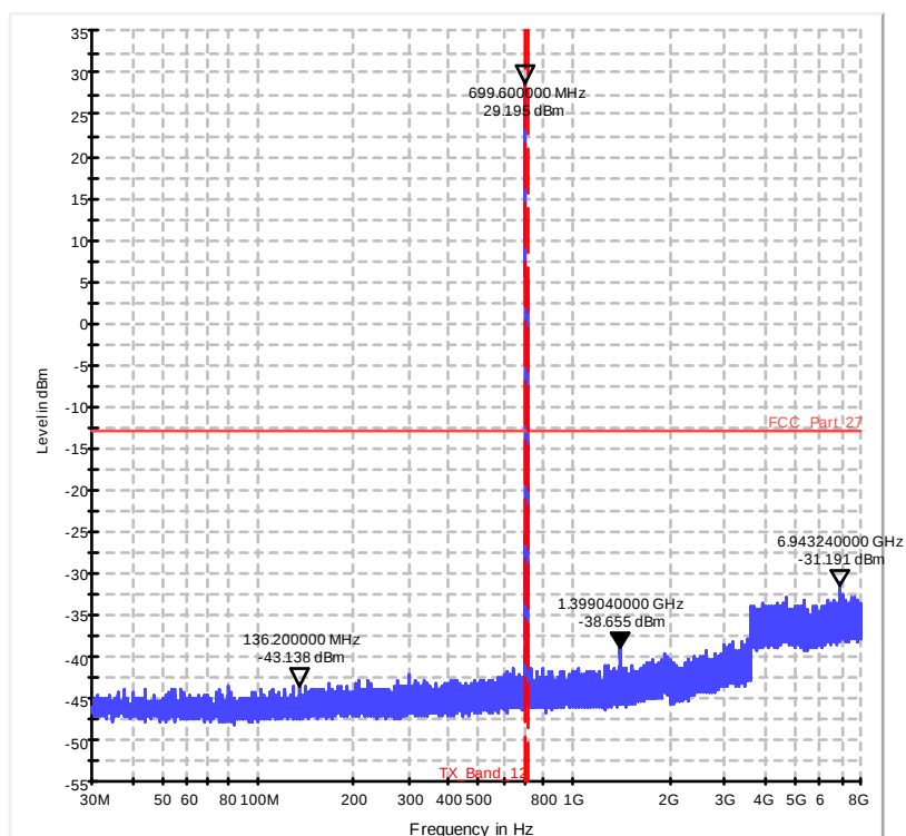
Diagram 36.1202a_Ch23060_BW_10_1RB_low_QPSK_Sweep2
