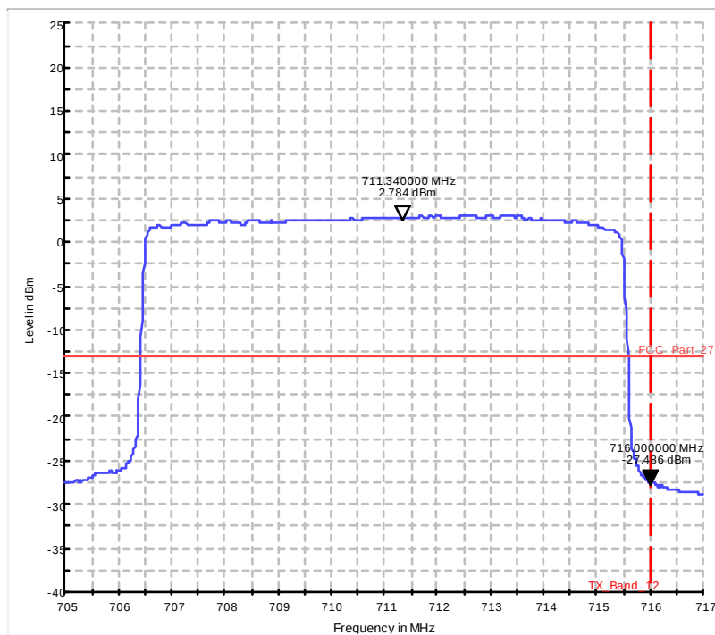
Diagram 37.1216b_Ch23130_BW_10_50RBs_16QAM
