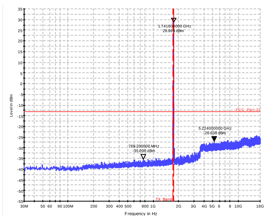
Diagram 36.43a_CSE_Ch20175_BW_20_1RB_high_QPSK_Sweep2
