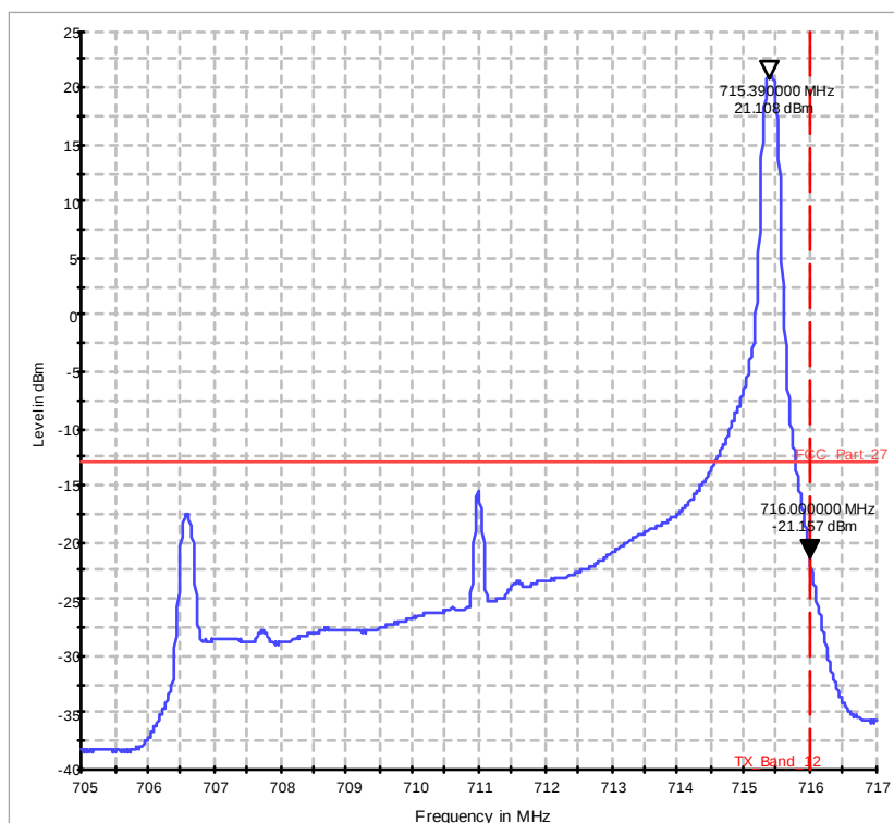
Diagram 37.1215a_Ch23130_BW_10_1RB_high_QPSK
