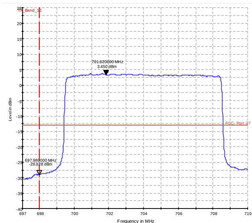
Diagram 37.1208a_Ch23060_BW_10_50RBs_QPSK
