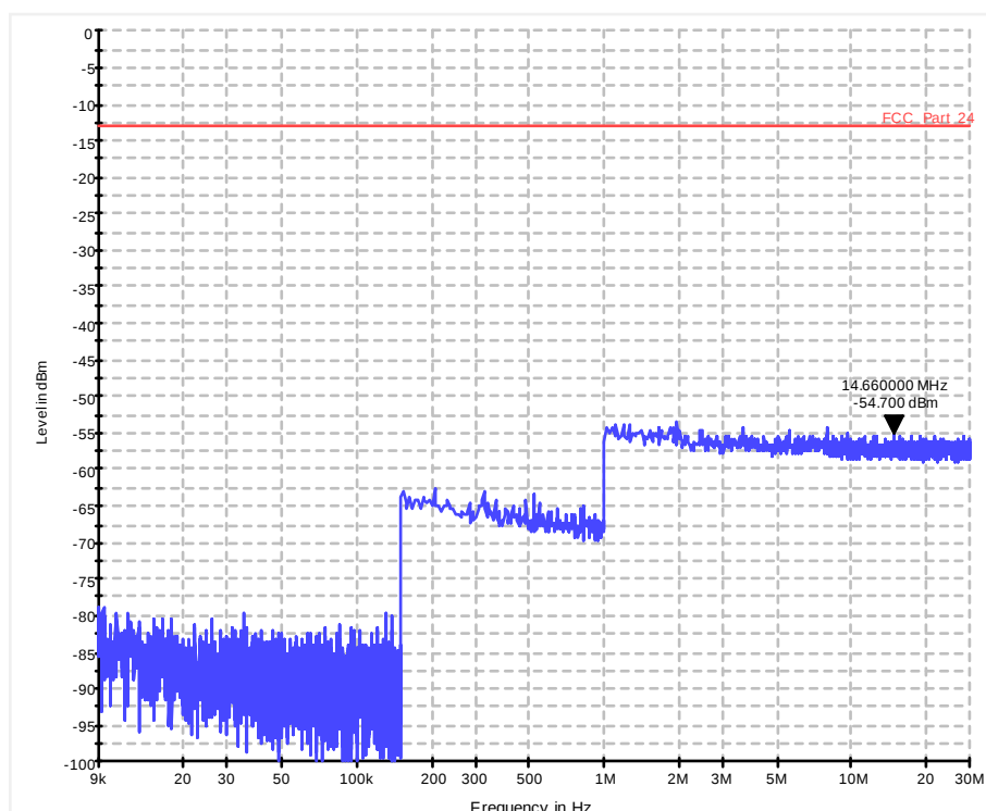
Diagram 36.40b_CSE_Ch2000_BW_10_1RB_high_16QAM_Sweep1
