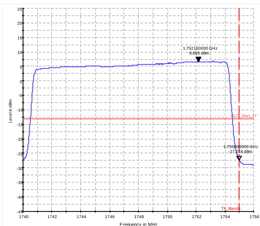
Diagram 37.422a_Ch20325_BW_15_75RBs_QPSK
