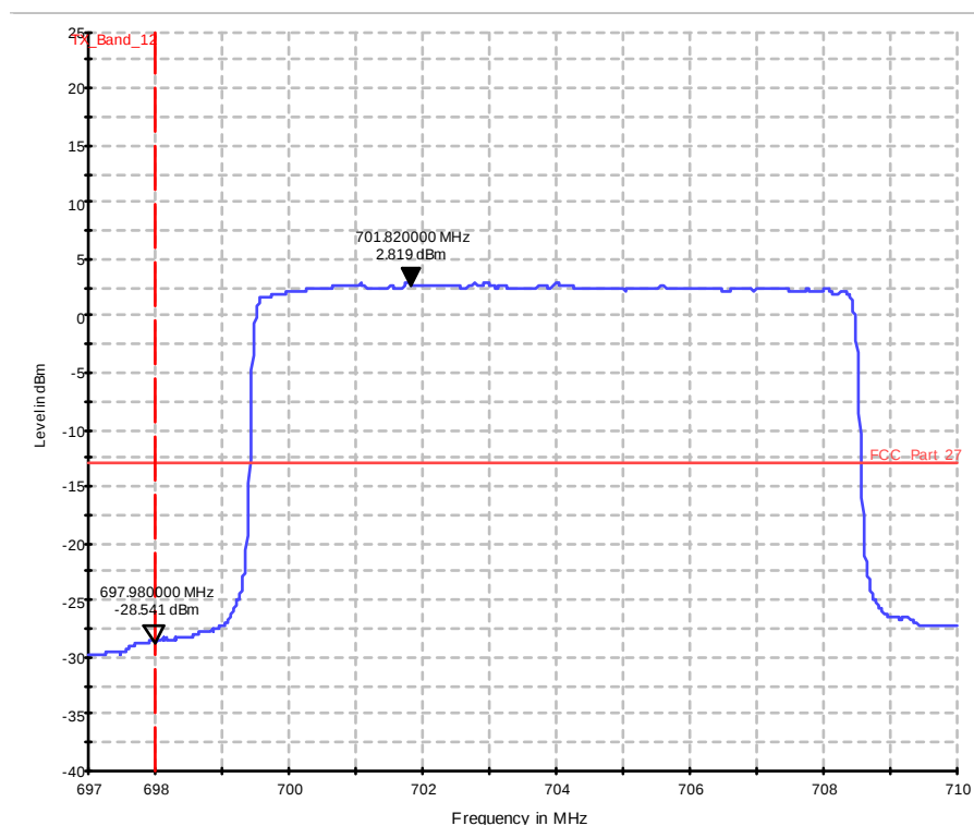
Diagram 37.1208b_Ch23060_BW_10_50RBs_16QAM
