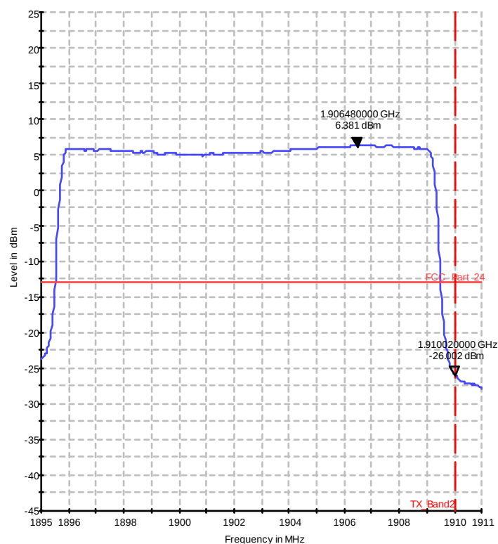
Diagram 37.222a_ch19125_75RB_high_QPSK
