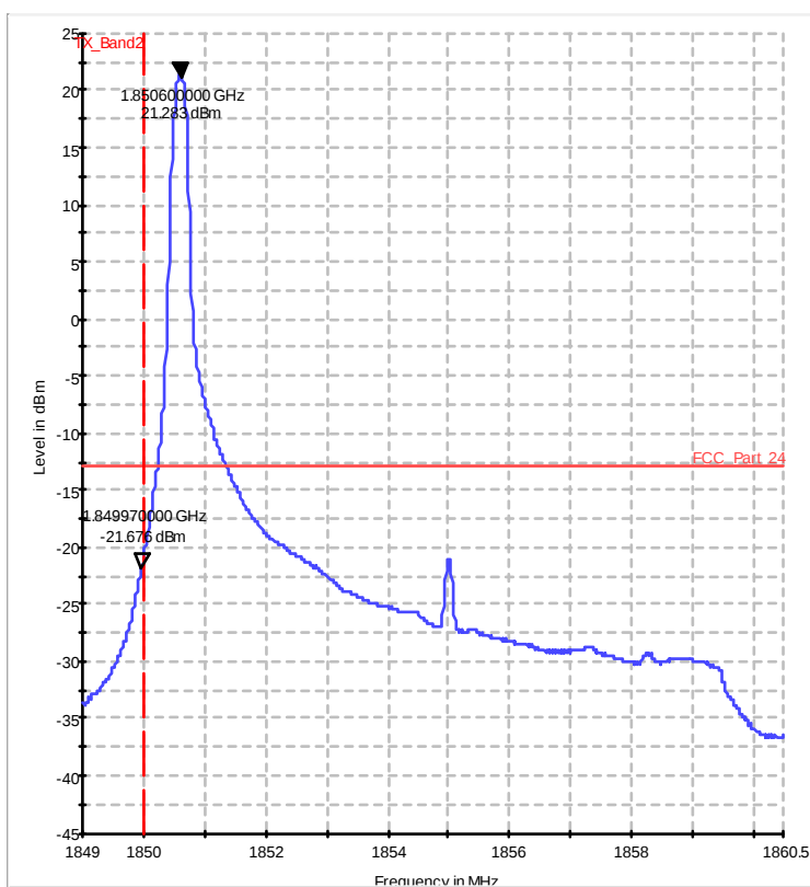
Diagram 37.208b_ch18650_50RB_QAM
