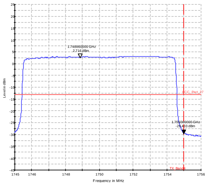
Diagram 37.420b_Ch20350_BW_10_50RBs_16QAM
