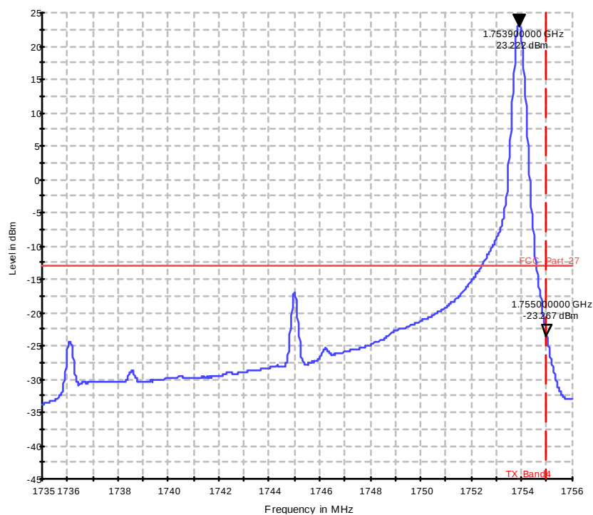
Diagram 37.423a_Ch20300_BW_20_1RB_high_QPSK
