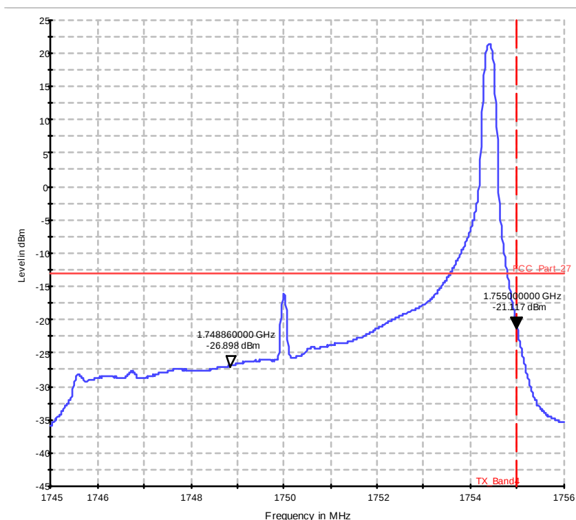
Diagram 37.419a_Ch20350_BW_10_1RB_high_QPSK
