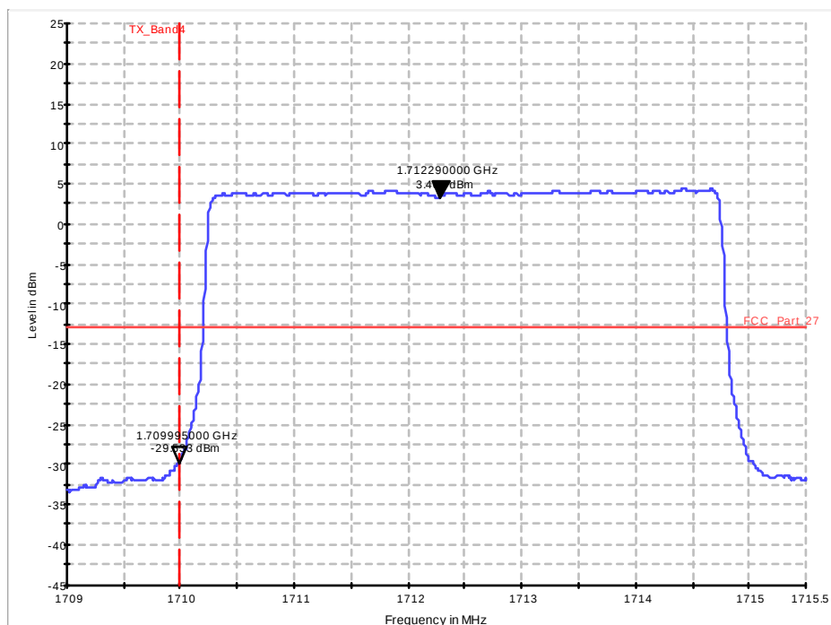
Diagram 37.406a_Ch19975_BW_5_25RBs_QPSK
