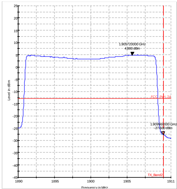
Diagram 37.224a_ch19100_100RB_high_QPSK
