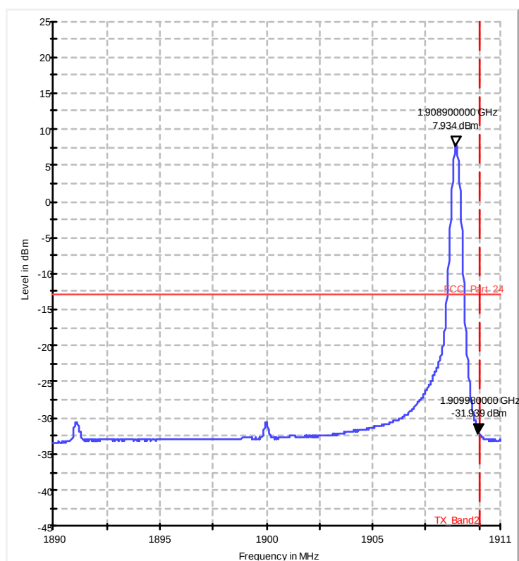
Diagram 37.223b_ch19100_1RB_high_QAM
