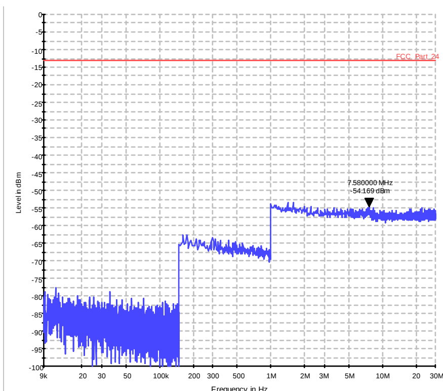
Diagram 36.42b_CSE_Ch20175_BW_20_1RB_high_16QAM_Sweep1
