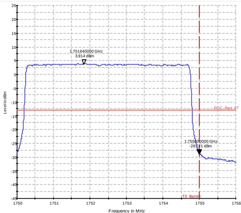
Diagram 37.418a_Ch20375_BW_5_25RBs_QPSK
