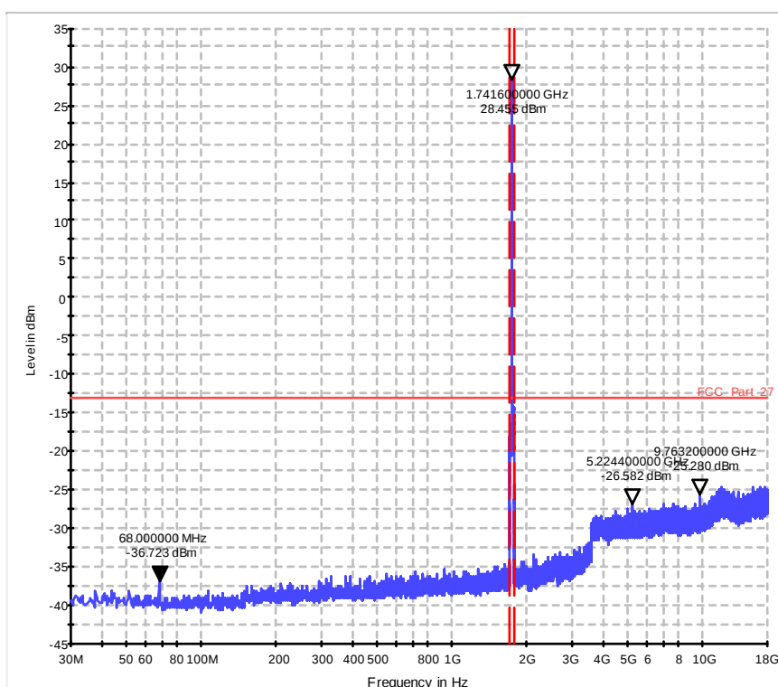
Diagram 36.43b_CSE_Ch20175_BW_20_1RB_high_16QAM_Sweep2
