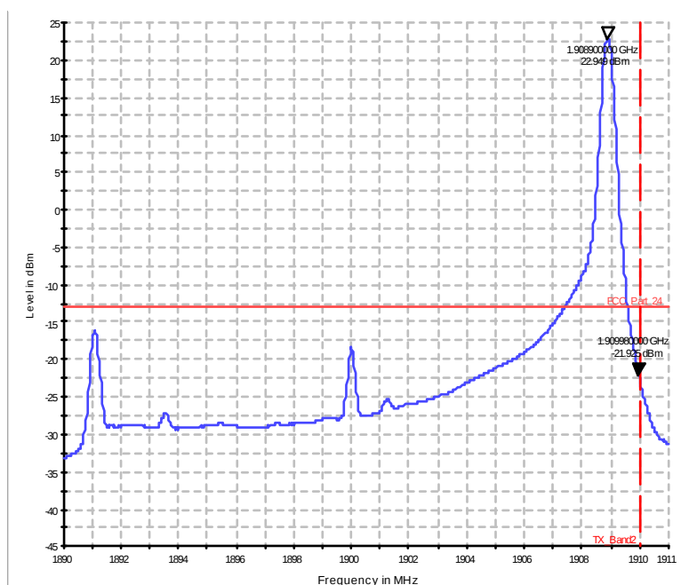
Diagram 37.223a_ch19100_1RB_high_QPSK
