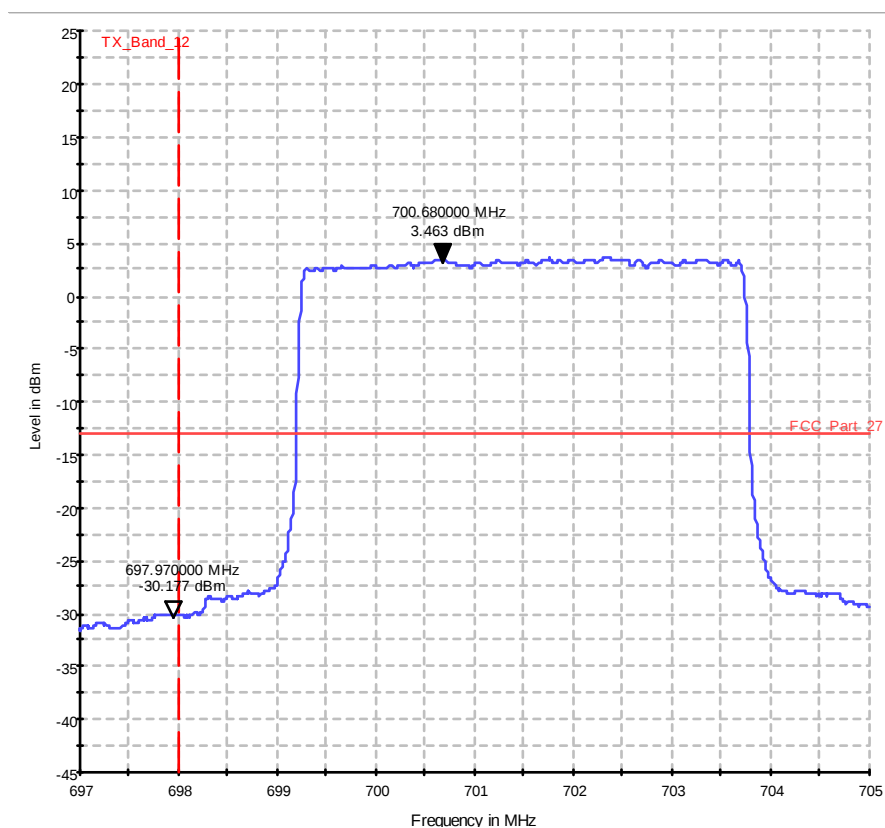
Diagram 37.1206a_Ch23035_BW_5_25RBs_QPSK
