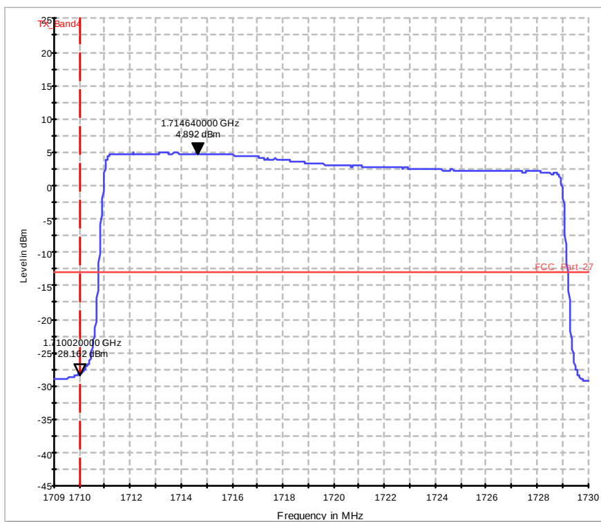
Diagram 37.412b_Ch20050_BW_20_100RBs_16QAM
