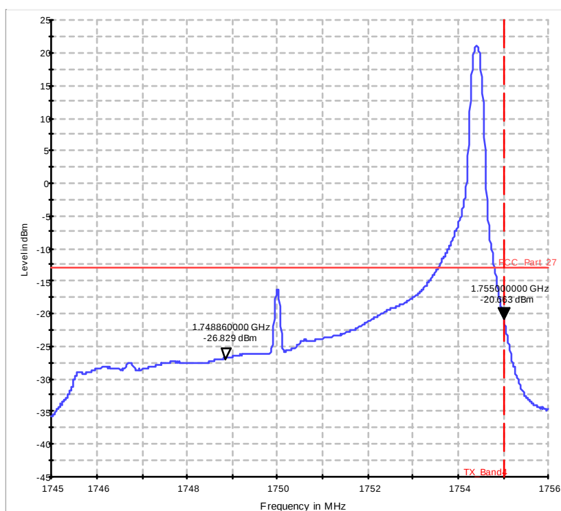
Diagram 37.419b_Ch20350_BW_10_1RB_high_16QAM
