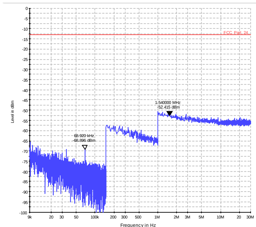
Diagram 36.1203a_Ch23095_BW_10_1RB_high_QPSK_Sweep1
