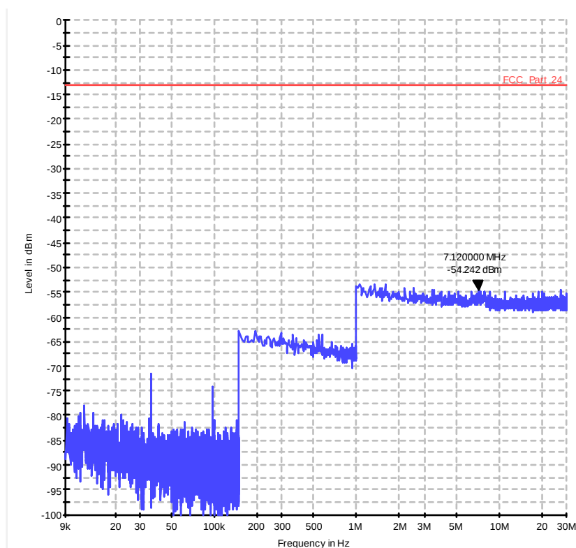
Diagram 26.24b_CSE_Ch19150_BW_10_1RB_low_16QAM_Sweep1
