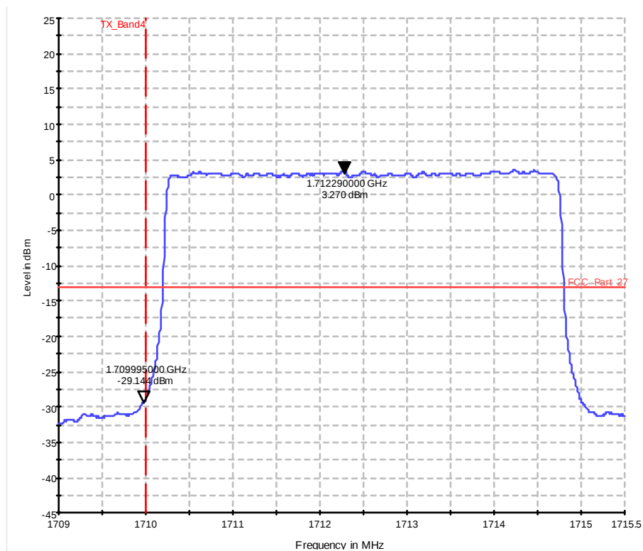
Diagram 37.406b_Ch19975_BW_5_25RBs_16QAM
