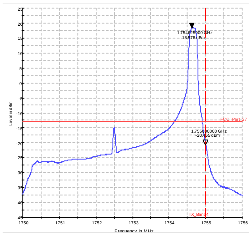
Diagram 37.417a_Ch20375_BW_5_1RB_high_QPSK
