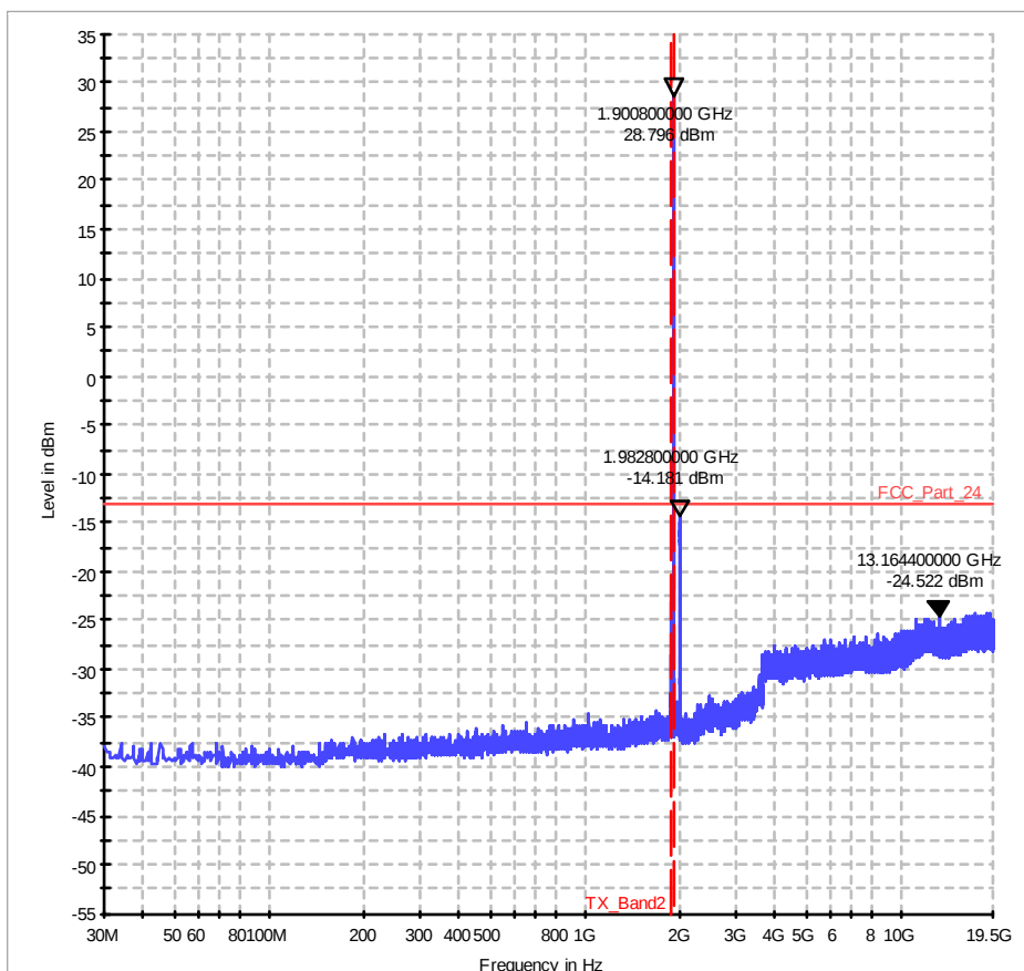
Diagram 26.25a_CSE_Ch19150_BW_10_1RB_low_QPSK_Sweep2
