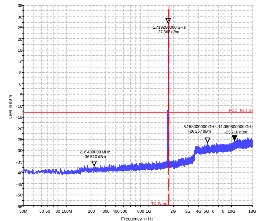
Diagram 36.41b_CSE_Ch2000_BW_10_1RB_high_16QAM_Sweep2
