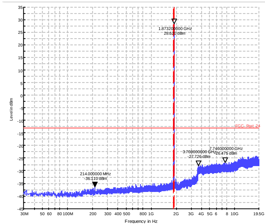
Diagram 36.23a_CSE_Ch18900_BW_15_1RB_low_QPSK_Sweep2
