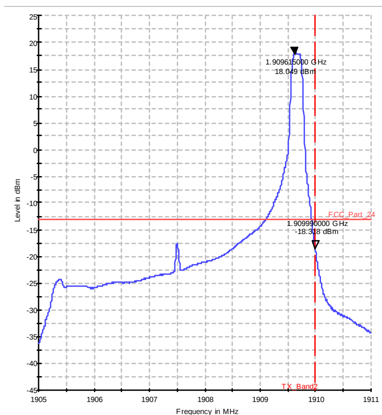
Diagram 37.217b_ch19175_1RB_high_QAM
