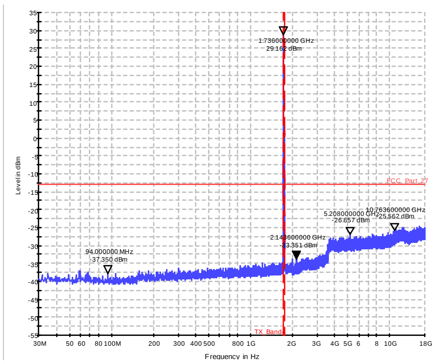
Diagram 36.45a_CSE_Ch20300_BW_20_1RB_low_QPSK_Sweep2
