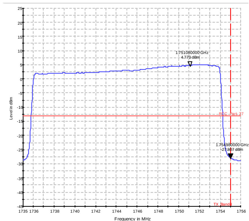
Diagram 37.424b_Ch20300_BW_20_100RBs_16QAM
