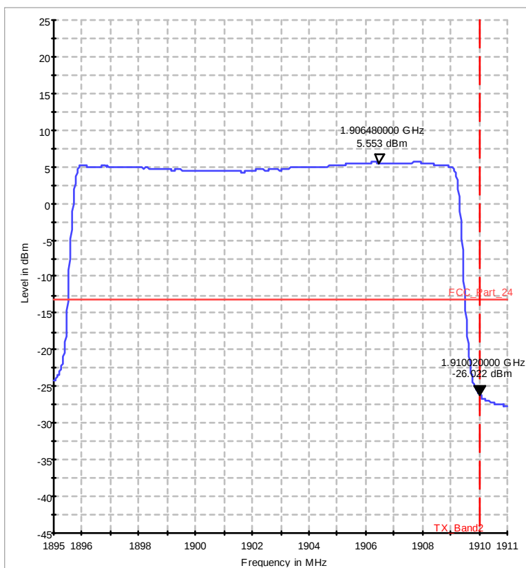
Diagram 37.222b_ch19125_75RB_high_QAM
