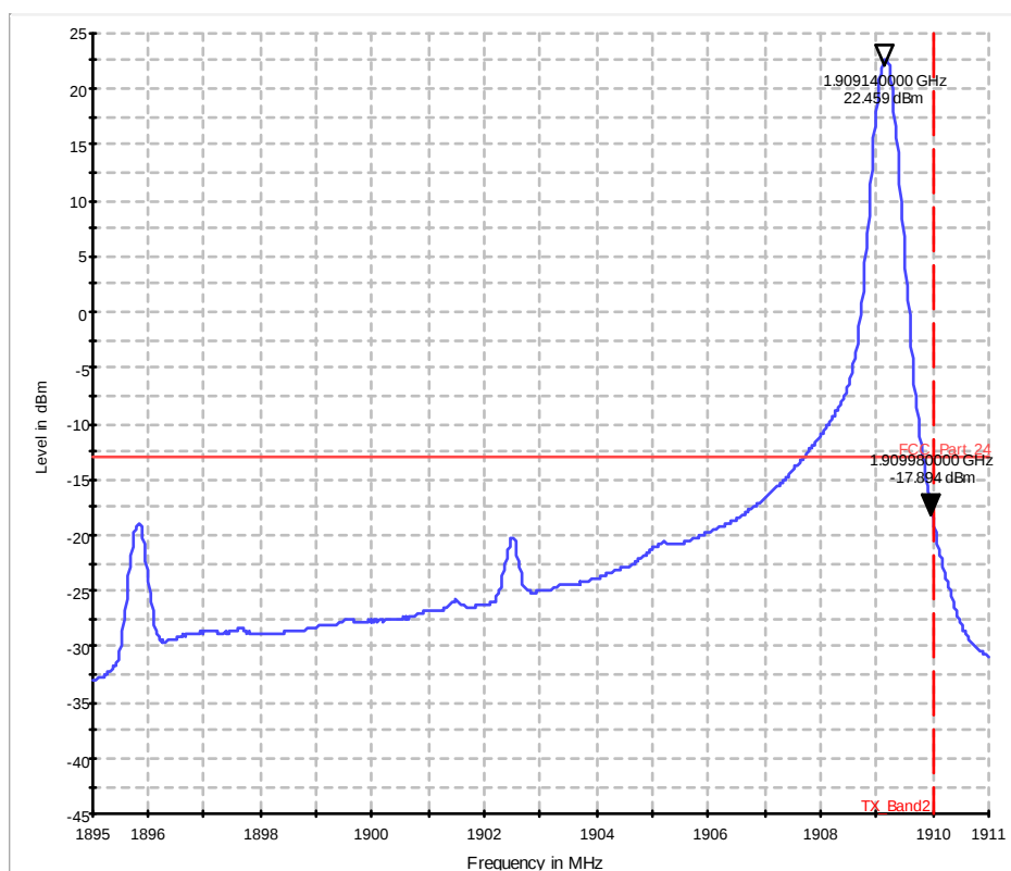
Diagram 37.221b_ch19125_1RB_high_QAM
