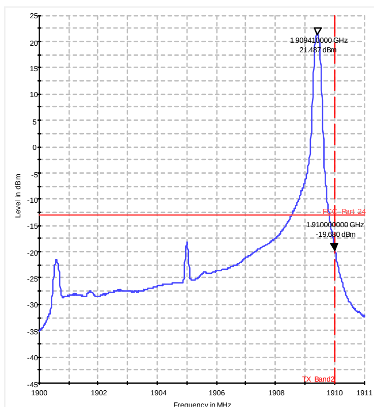
Diagram 37.219a_ch19150_1RB_high_QPSK
