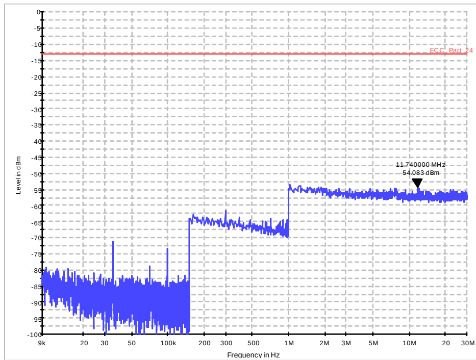
Diagram 26.24a_CSE_Ch19150_BW_10_1RB_low_QPSK_Sweep1
