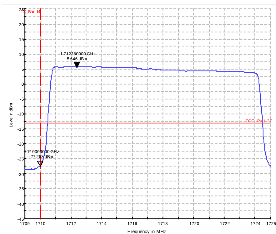
Diagram 37.410b_Ch20025_BW_15_75RBs_16QAM
