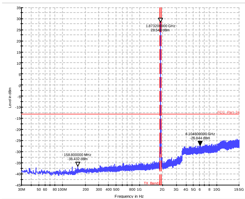
Diagram 36.23b_CSE_Ch18900_BW_15_1RB_low_16QAM_Sweep2
