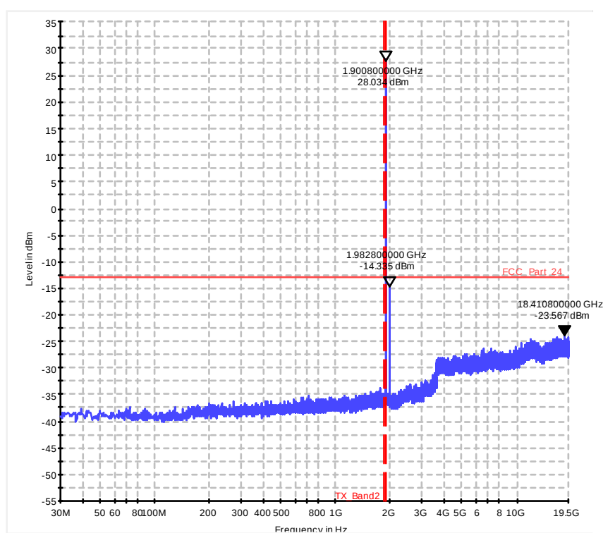
Diagram 26.25b_CSE_Ch19150_BW_10_1RB_low_16QAM_Sweep2
