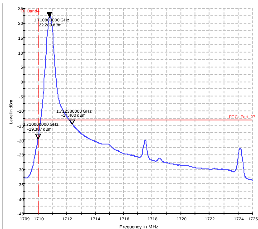
Diagram 37.409b_Ch20025_BW_15_1RB_low_16QAM
