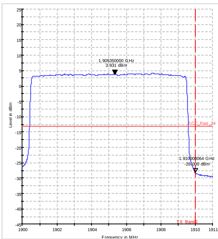
Diagram 37.220a_ch19150_50RB_high_QPSK
