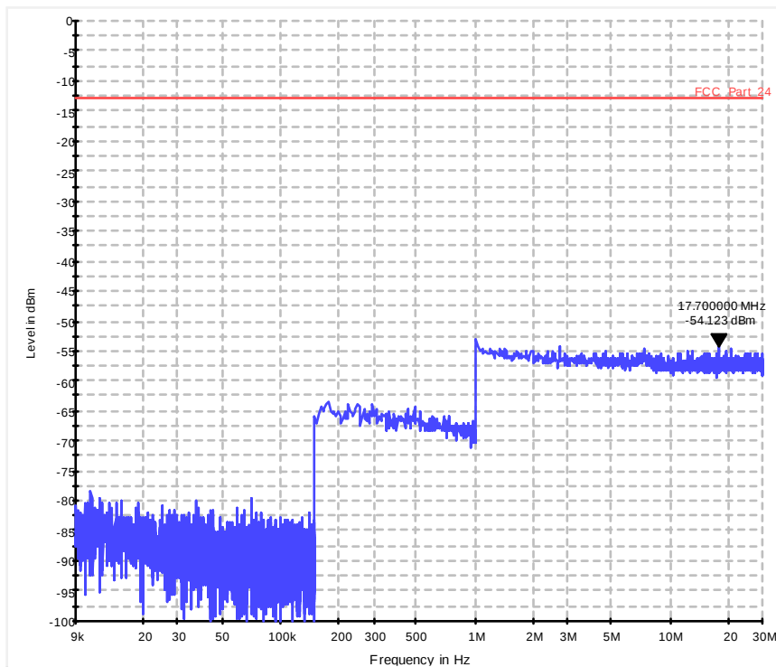
Diagram 36.40a_CSE_Ch2000_BW_10_1RB_high_QPSK_Sweep1
