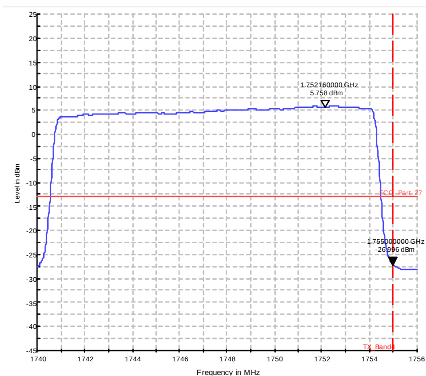
Diagram 37.422b_Ch20325_BW_15_75RBs_16QAM
