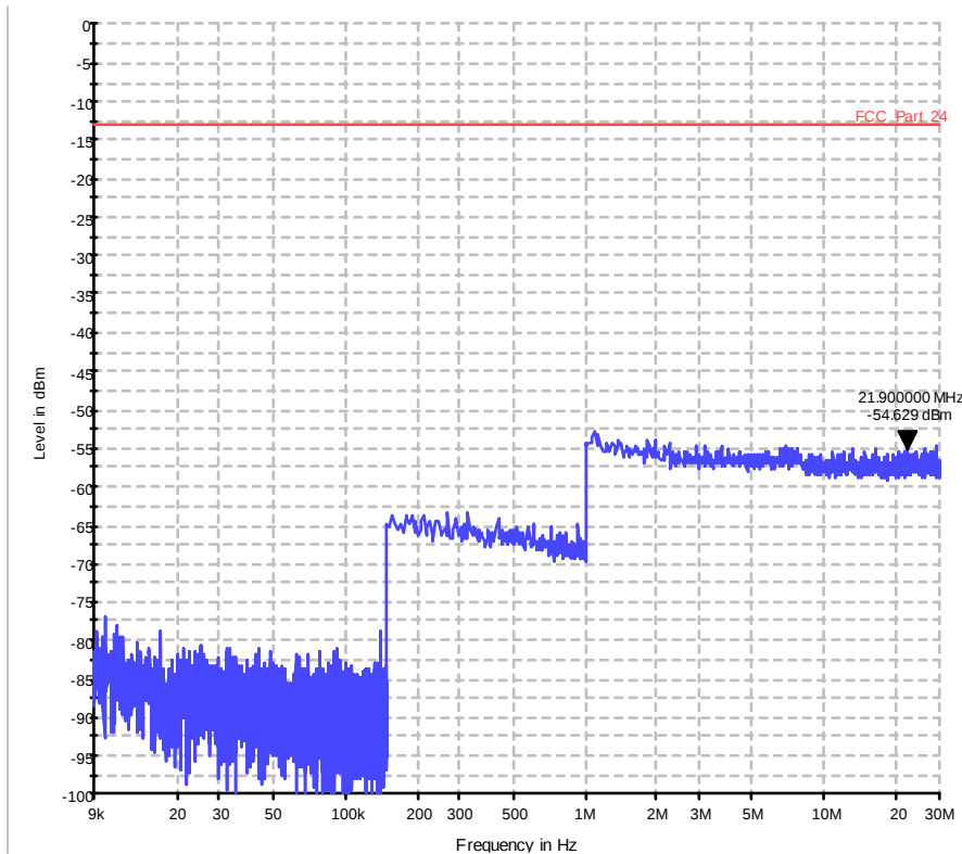
Diagram 36.44a_CSE_Ch20300_BW_20_1RB_low_QPSK_Sweep1
