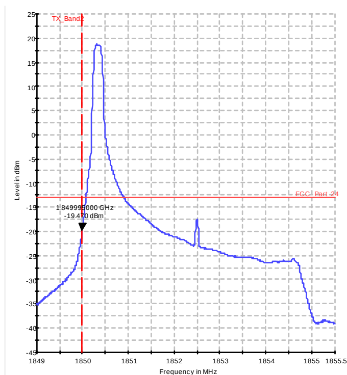
Diagram 37.205b_ch18625_1RB_low_QAM
