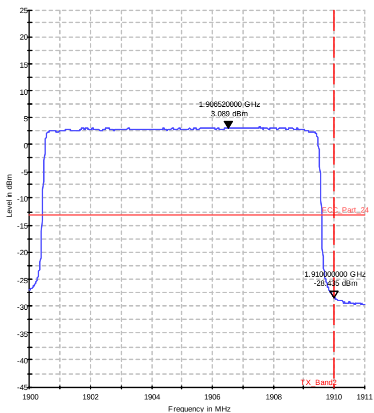
Diagram 37.220b_ch19150_50RB_high_QAM
