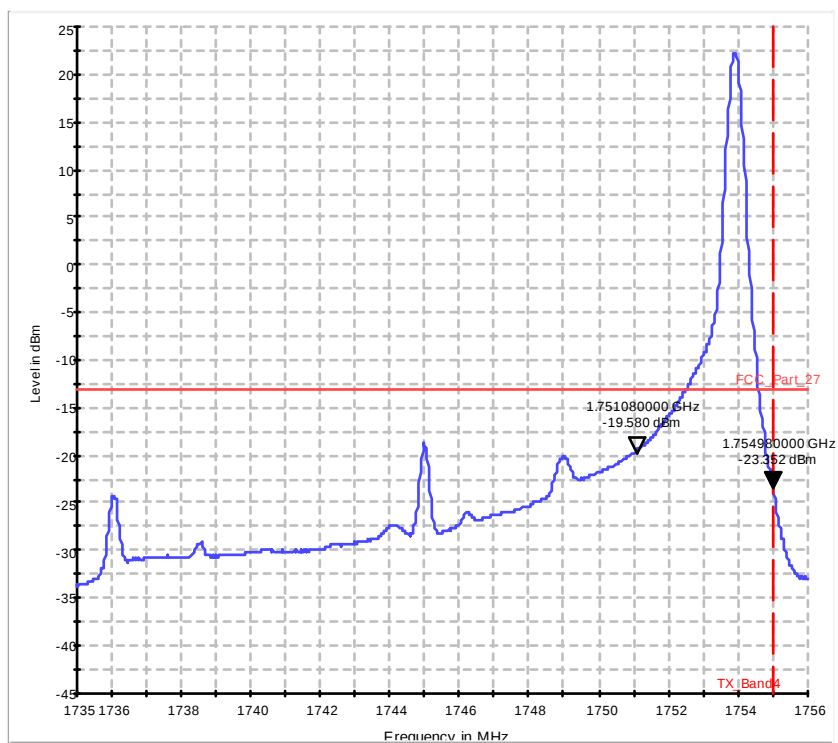
Diagram 37.423b_Ch20300_BW_20_1RB_high_16QAM
