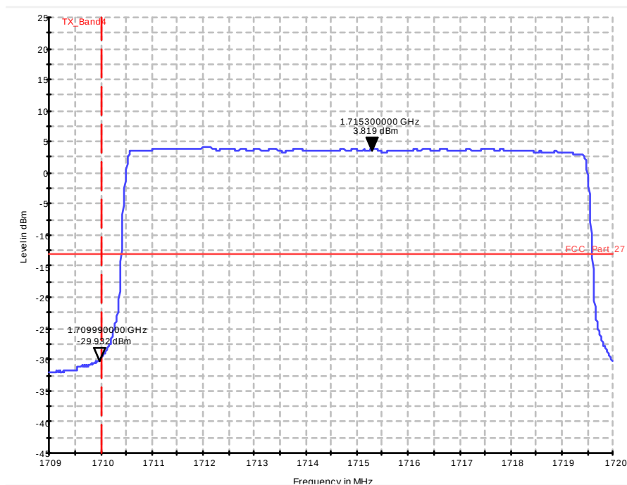
Diagram 37.408a_Ch20000_BW_10_50RBs_QPSK
