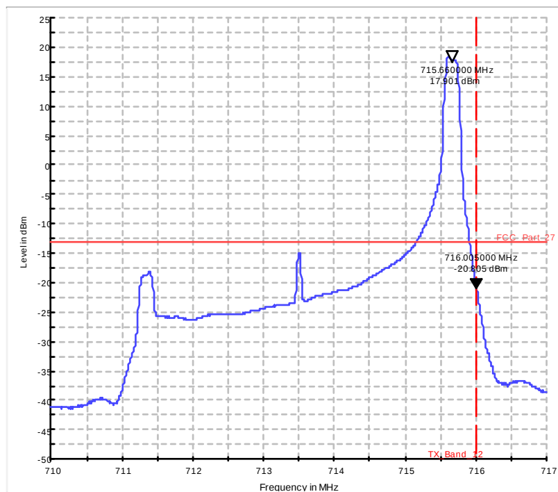
Diagram 37.1213a_Ch23155_BW_5_1RB_high_QPSK
