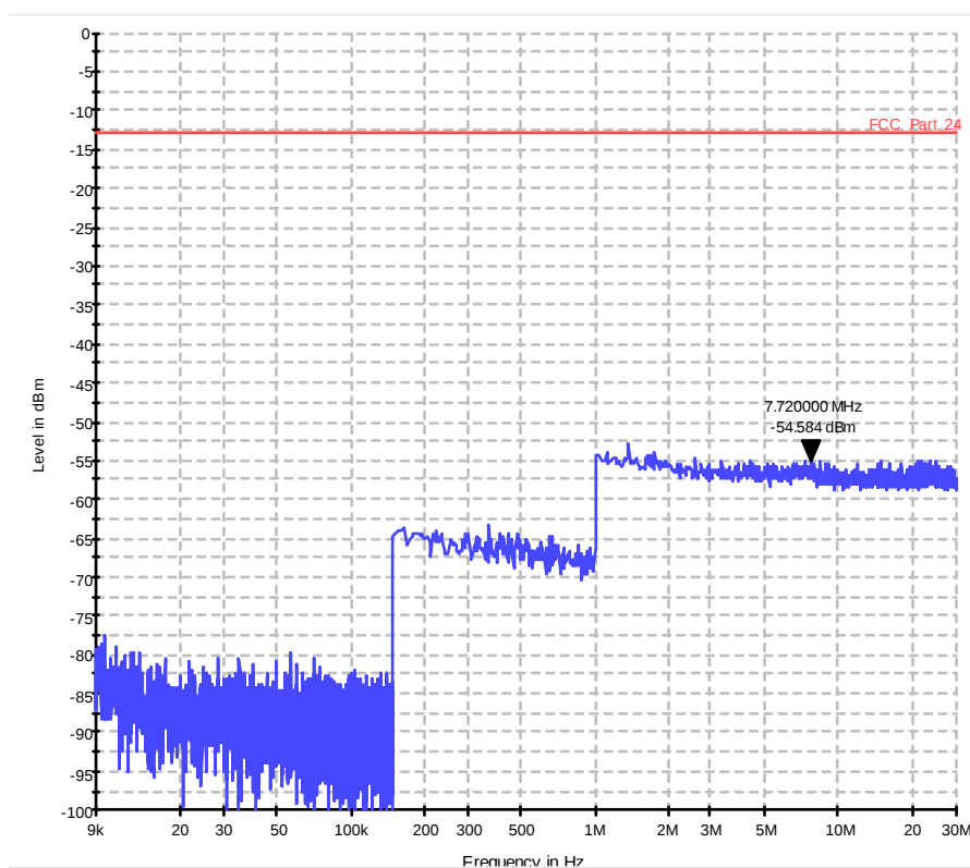
Diagram 36.42a_CSE_Ch20175_BW_20_1RB_high_QPSK_Sweep1
