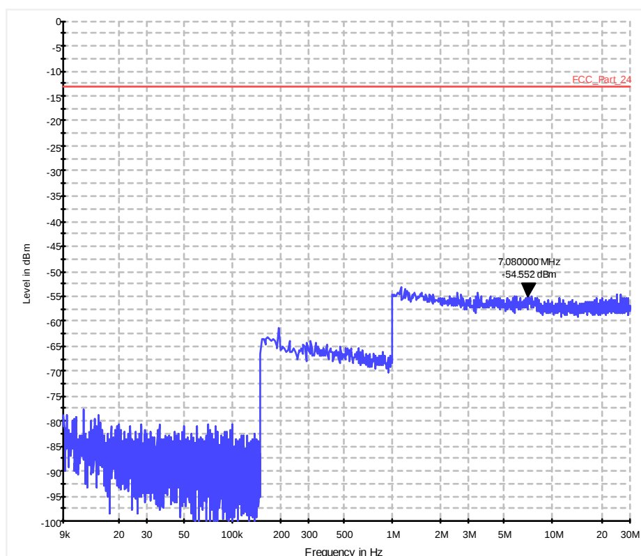
Diagram 36.20b_CSE_Ch18700_BW_20_1RB_high_16QAM_Sweep1
