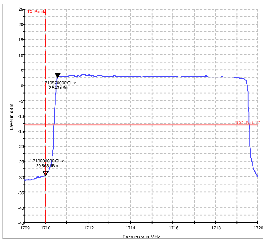
Diagram 37.408b_Ch20000_BW_10_50RBs_16QAM
