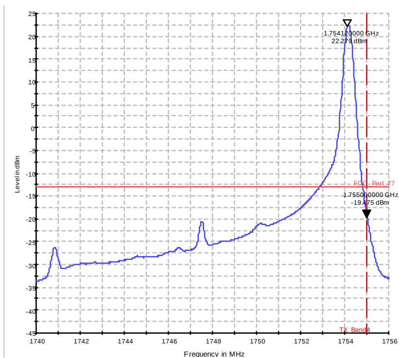
Diagram 37.421b_Ch20325_BW_15_1RB_high_16QAM
