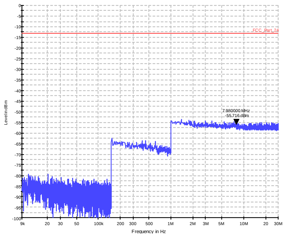
Diagram 36.20a_CSE_Ch18700_BW_20_1RB_high_QPSK_Sweep1
