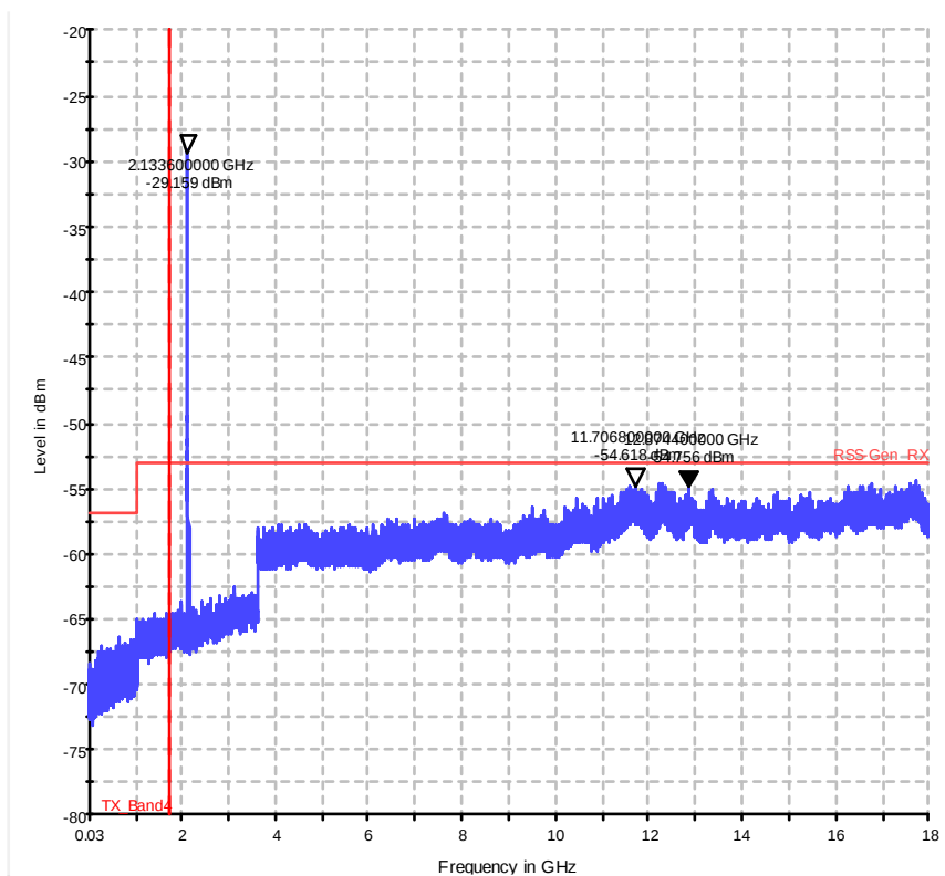
Diagram 50_02_CH_20175_QPSK_RB_Full_FDD4
