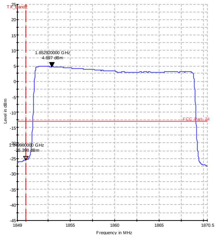
Diagram 37.212b_ch18700_100RB_low_QAM
