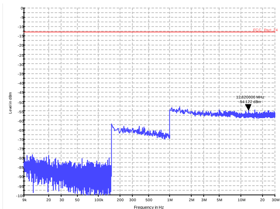
Diagram 36.44b_CSE_Ch20300_BW_20_1RB_low_16QAM_Sweep1
