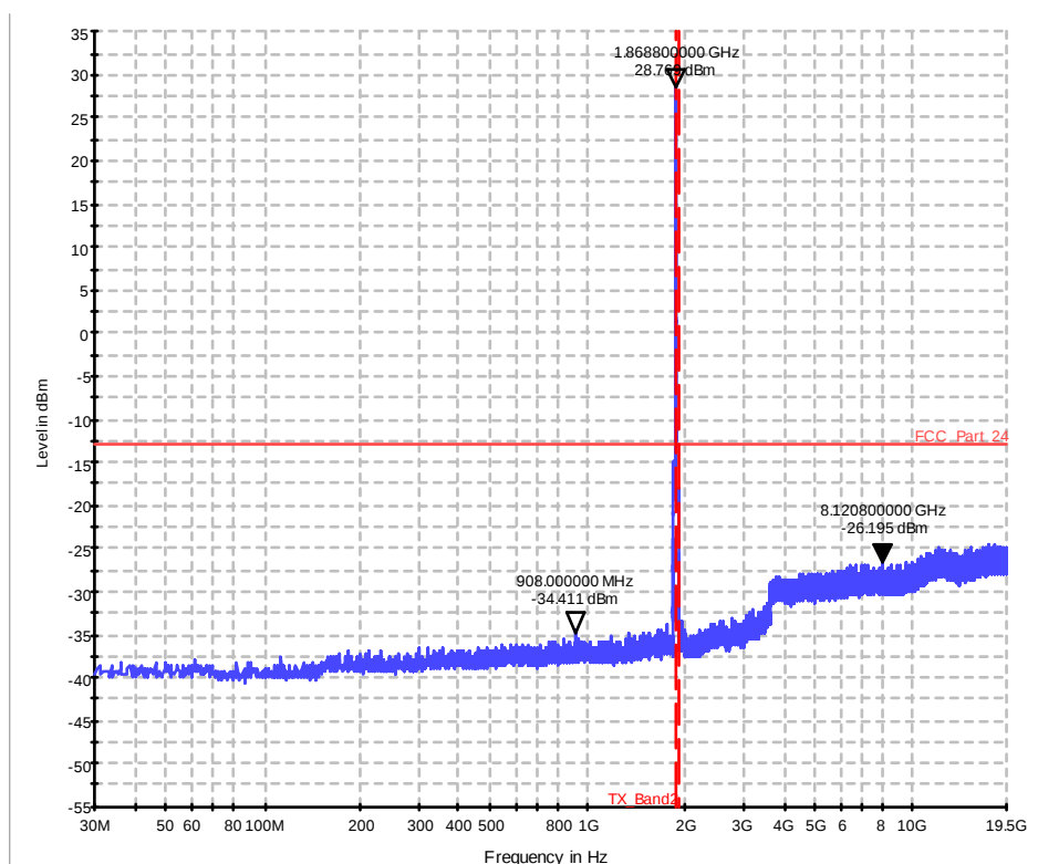
Diagram 36.21b_CSE_Ch18700_BW_20_1RB_high_16QAM_Sweep2
