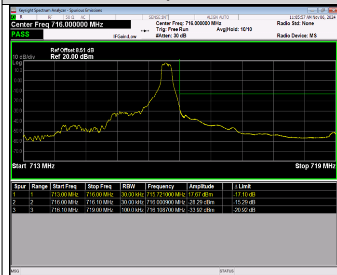
Band12-1.4MHz-16QAM-23017-1RB#0
