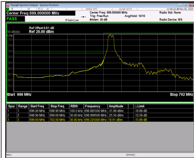
Band12-1.4MHz-QPSK-23017-6RB#0
