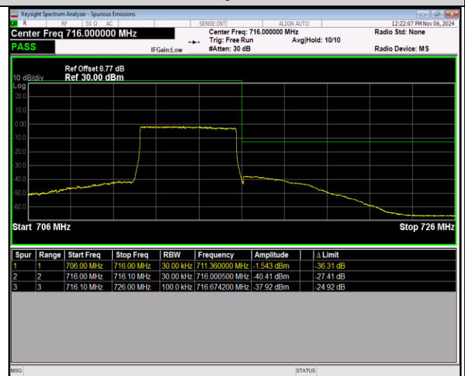
Band17-10MHz-QPSK-23780-1RB#49
