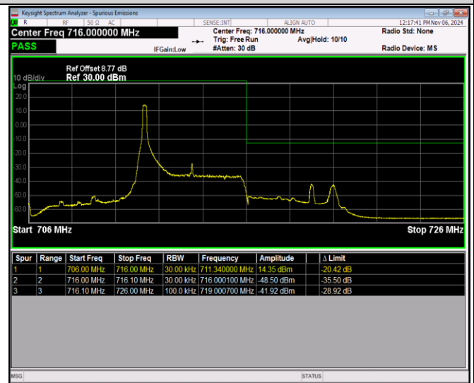
Band17-5MHz-16QAM-23825-25RB#0
