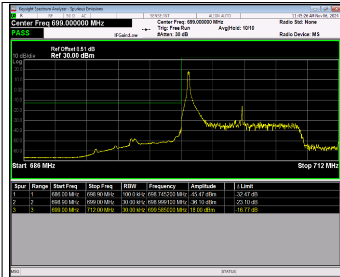
Band12-10MHz-QPSK-23060-50RB#0
