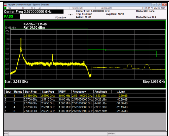
Band7-20MHz-64QAM-21350-100RB#0
