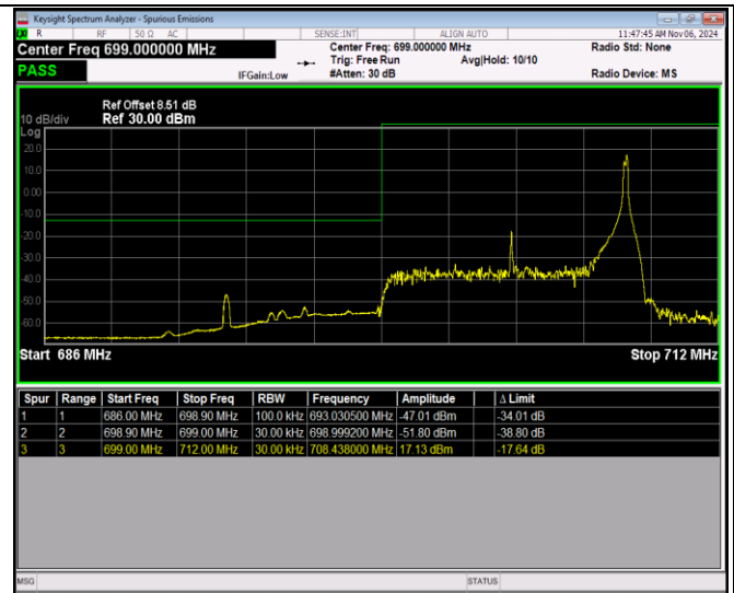
Band12-10MHz-64QAM-23130-1RB#0
