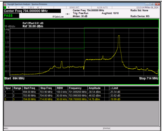
Band17-5MHz-QPSK-23825-1RB#0
