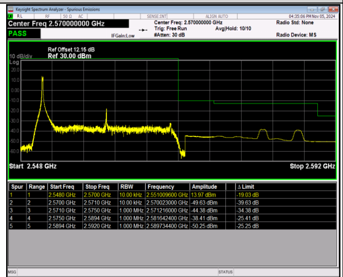
Band7-20MHz-16QAM-21350-100RB#0
