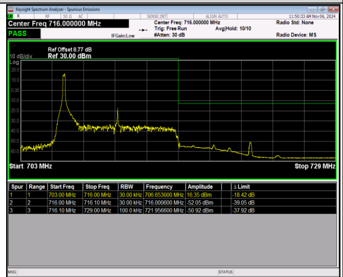
Band12-10MHz-64QAM-23130-50RB#0
