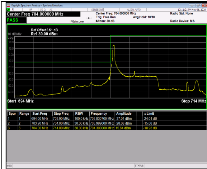
Band17-5MHz-QPSK-23755-25RB#0
