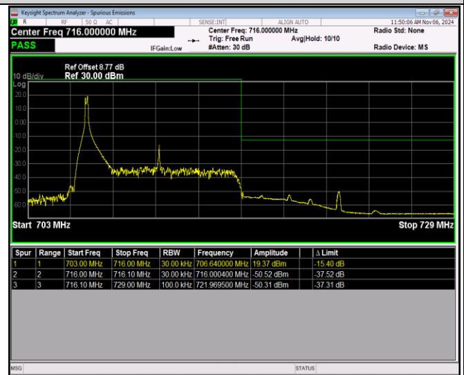
Band12-10MHz-16QAM-23130-50RB#0
