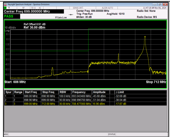
Band12-10MHz-16QAM-23130-1RB#0
