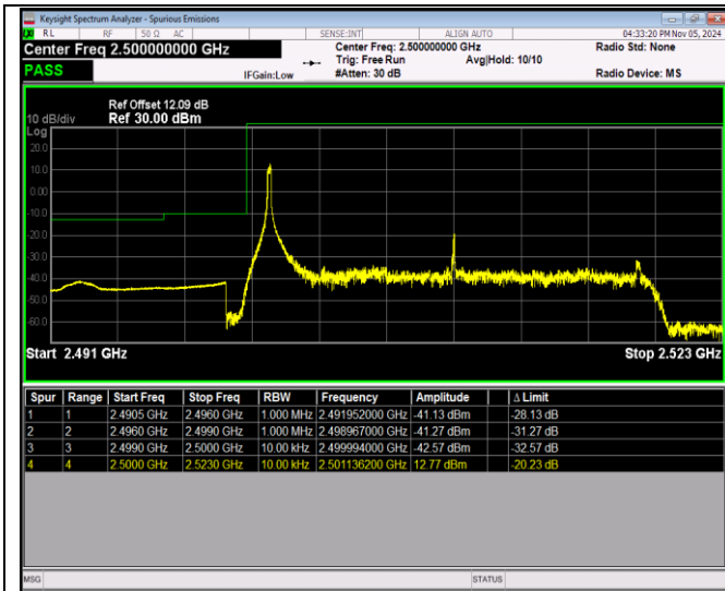
Band7-20MHz-64QAM-20850-100RB#0
