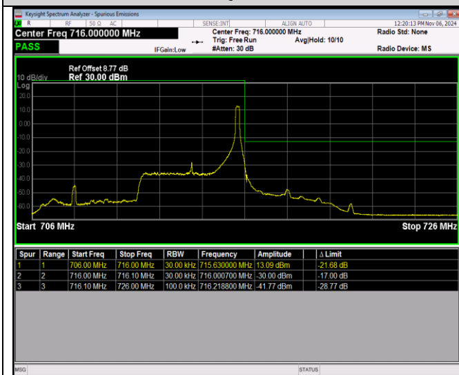
Band17-10MHz-QPSK-23780-1RB#0
