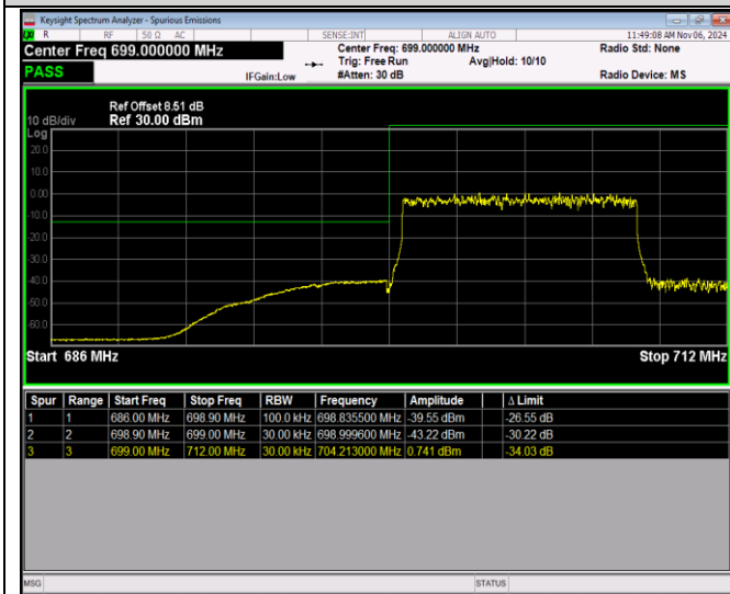
Band12-10MHz-64QAM-23130-1RB#49
