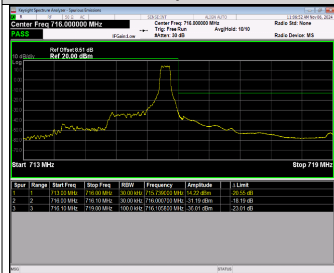
Band12-10MHz-QPSK-23060-1RB#0
