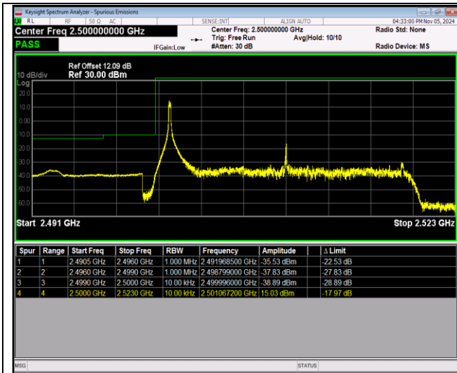
Band7-20MHz-QPSK-20850-100RB#0
