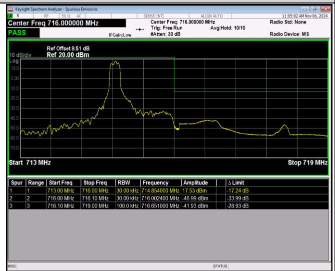
Band12-1.4MHz-16QAM-23173-6RB#0
