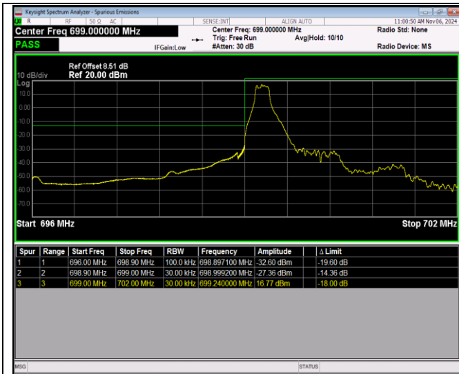
Band12-1.4MHz-16QAM-23017-6RB#0
