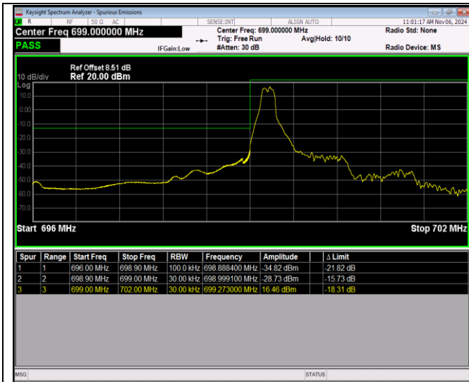
Band12-1.4MHz-64QAM-23017-6RB#0
