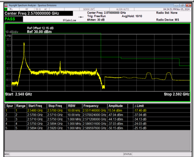
Band7-20MHz-QPSK-21350-100RB#0
