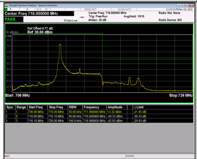
Band17-5MHz-64QAM-23825-25RB#0
