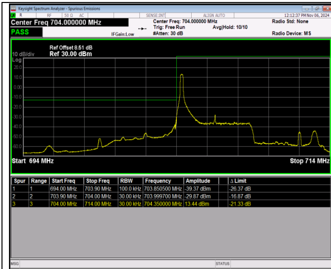
Band17-5MHz-64QAM-23755-25RB#0
