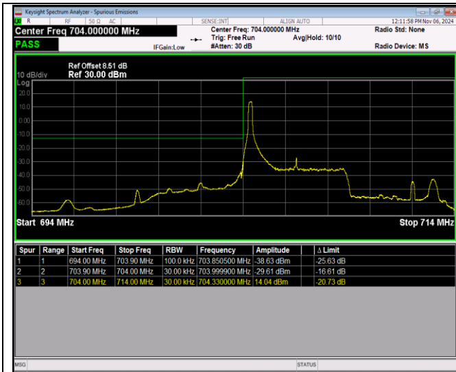
Band17-5MHz-16QAM-23755-25RB#0
