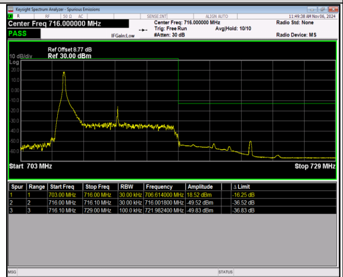
Band12-10MHz-QPSK-23130-50RB#0
