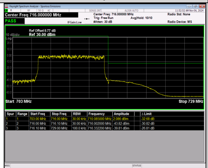
Band12-10MHz-64QAM-23060-1RB#49
