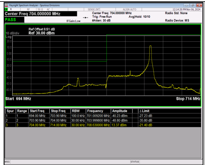
Band17-5MHz-64QAM-23825-1RB#0
