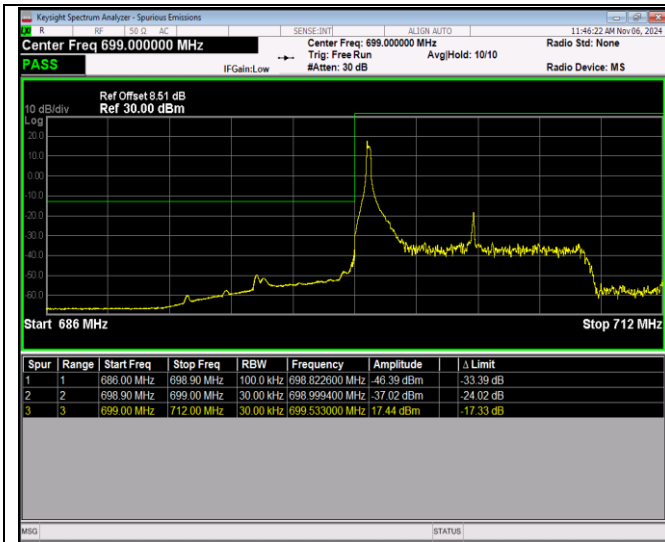
Band12-10MHz-64QAM-23060-50RB#0
