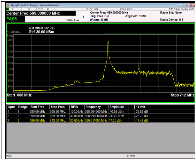
Band12-10MHz-16QAM-23060-50RB#0
