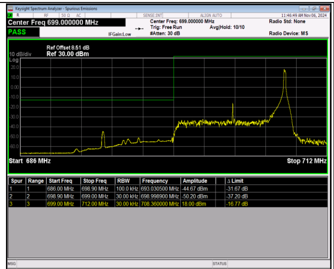
Band12-10MHz-QPSK-23130-1RB#0
