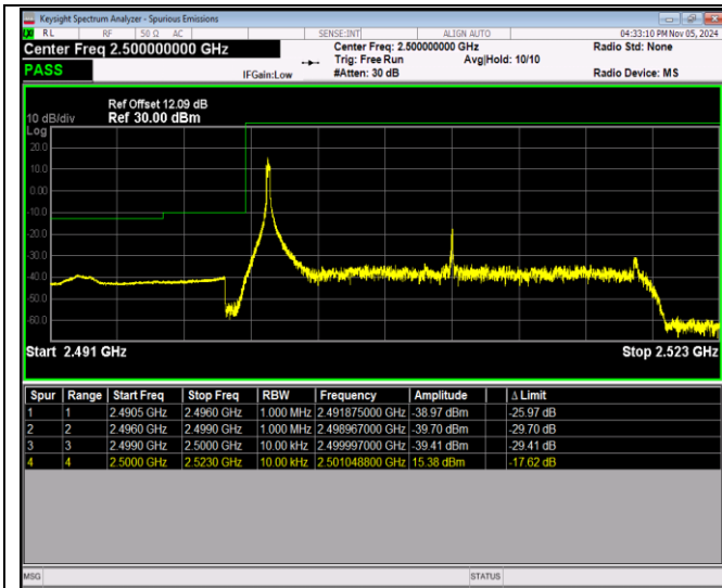
Band7-20MHz-16QAM-20850-100RB#0
