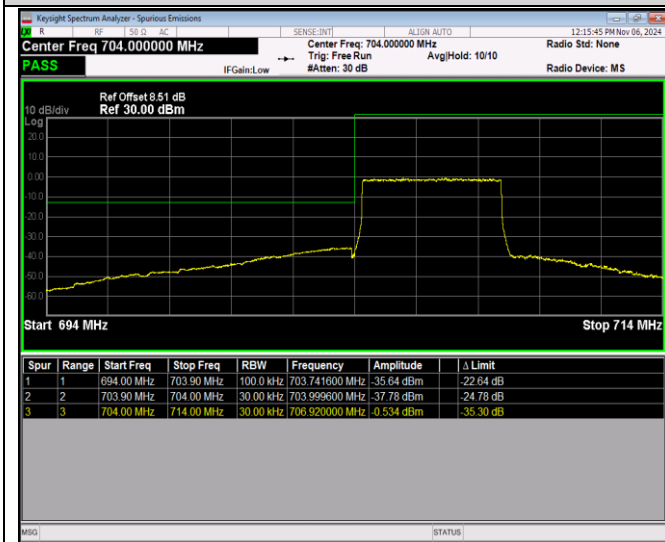
Band17-5MHz-16QAM-23825-1RB#24
