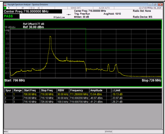
Band17-5MHz-QPSK-23825-25RB#0
