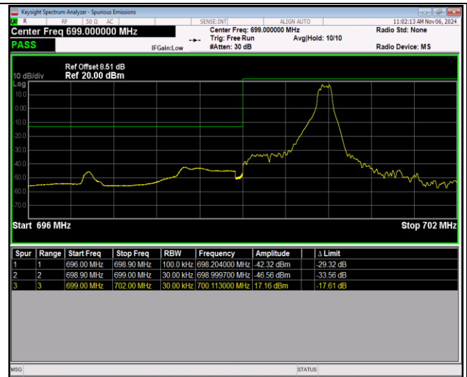
Band12-1.4MHz-16QAM-23173-1RB#0
