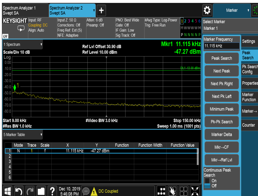
Figure 10 - 806.025 MHz, 9 kHz to 150 kHz
