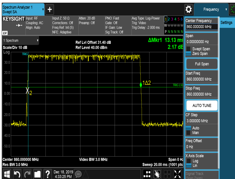
Figure 58 - Burst Length
