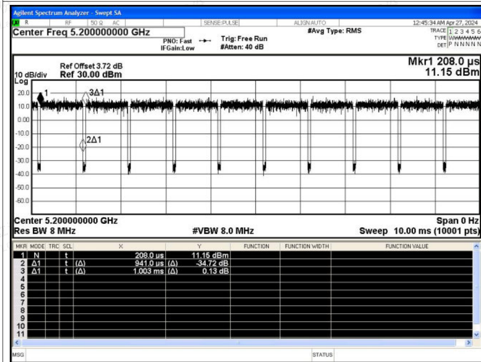
Duty Cycle NVNT ac20 5200MHz Ant4
