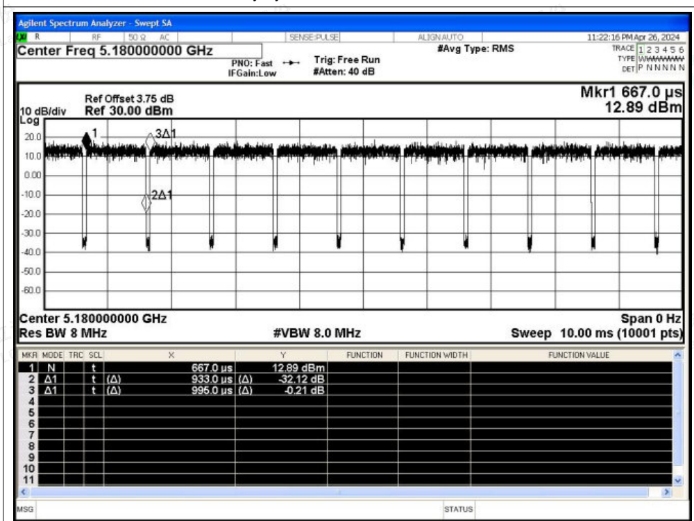
Duty Cycle NVNT n20 5180MHz Ant3
