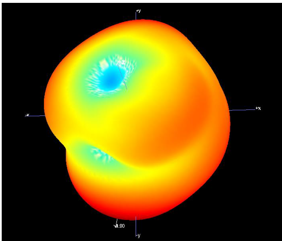
3D Pattern for 2450MHz
