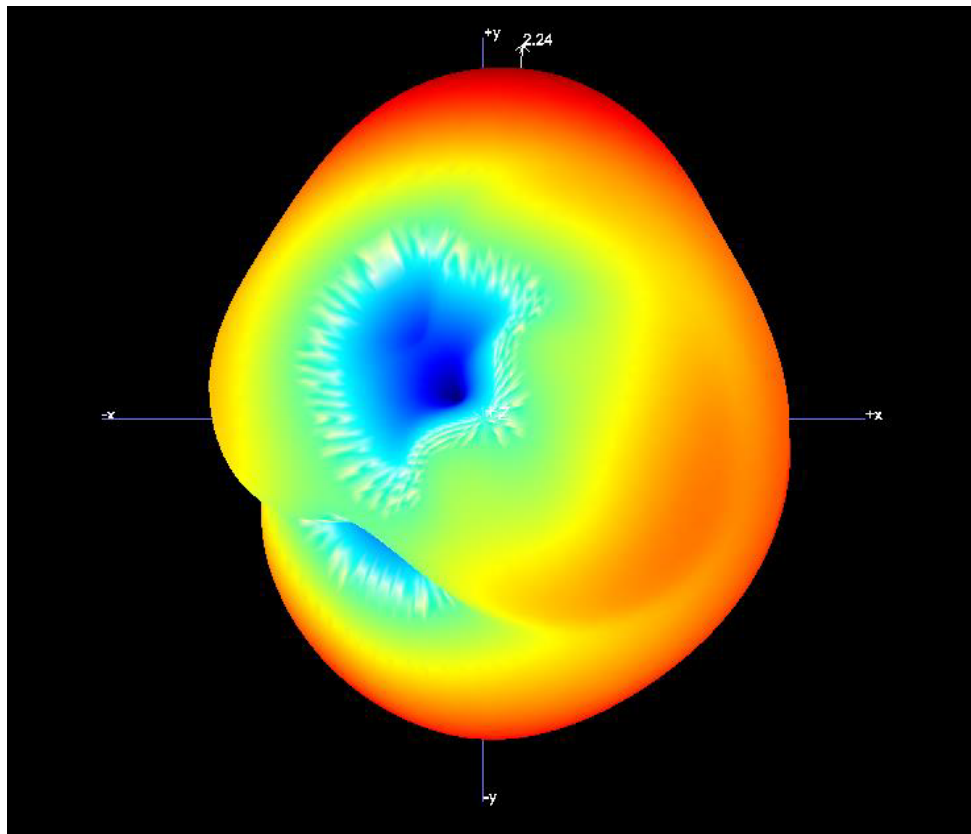
3D Pattern for 2400MHz
