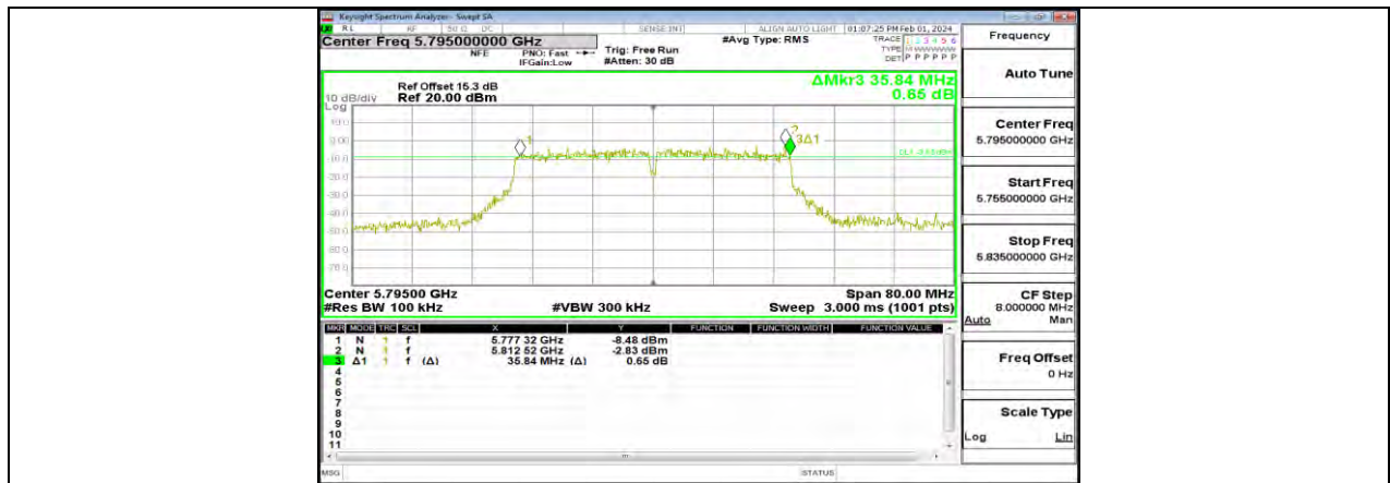
11N40SISO Ant1 5795
