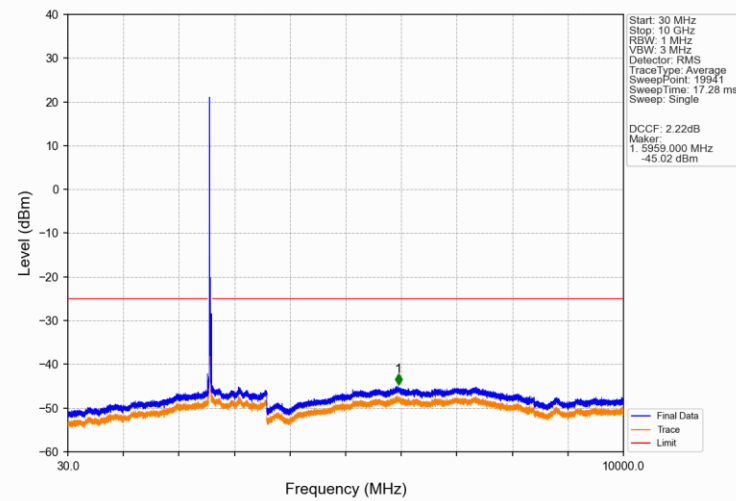
Band38 20MHz 16QAM LCH 2580MHz RB 1 0 NTV
