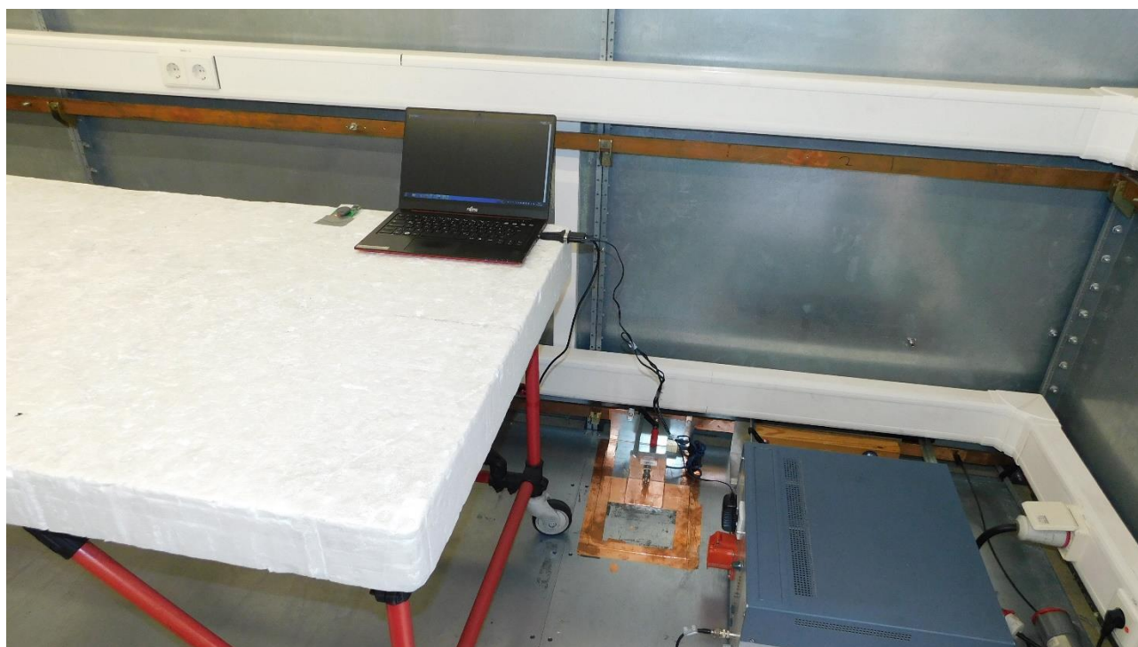
Picture 9: Test setup AC power line conducted emissions (front view), RS232
