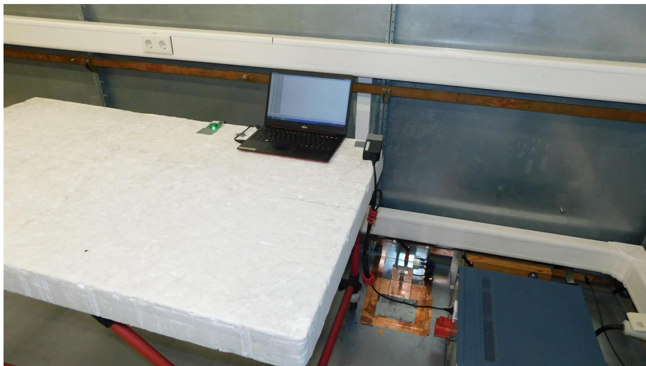
Picture 7: Test setup AC power line conducted emissions (front view), USB
