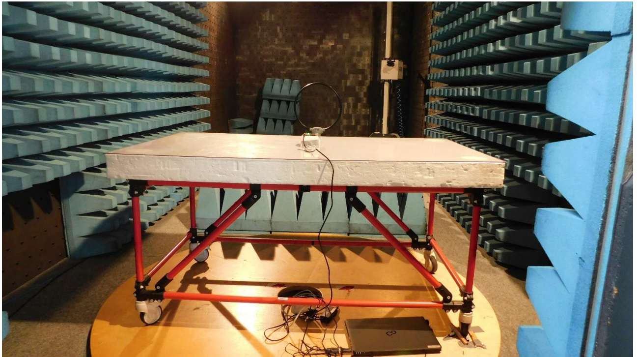
Picture 1: CDC, test setup radiated emission test 9 kHz -30 MHz and bandwidths measurement (front view)
