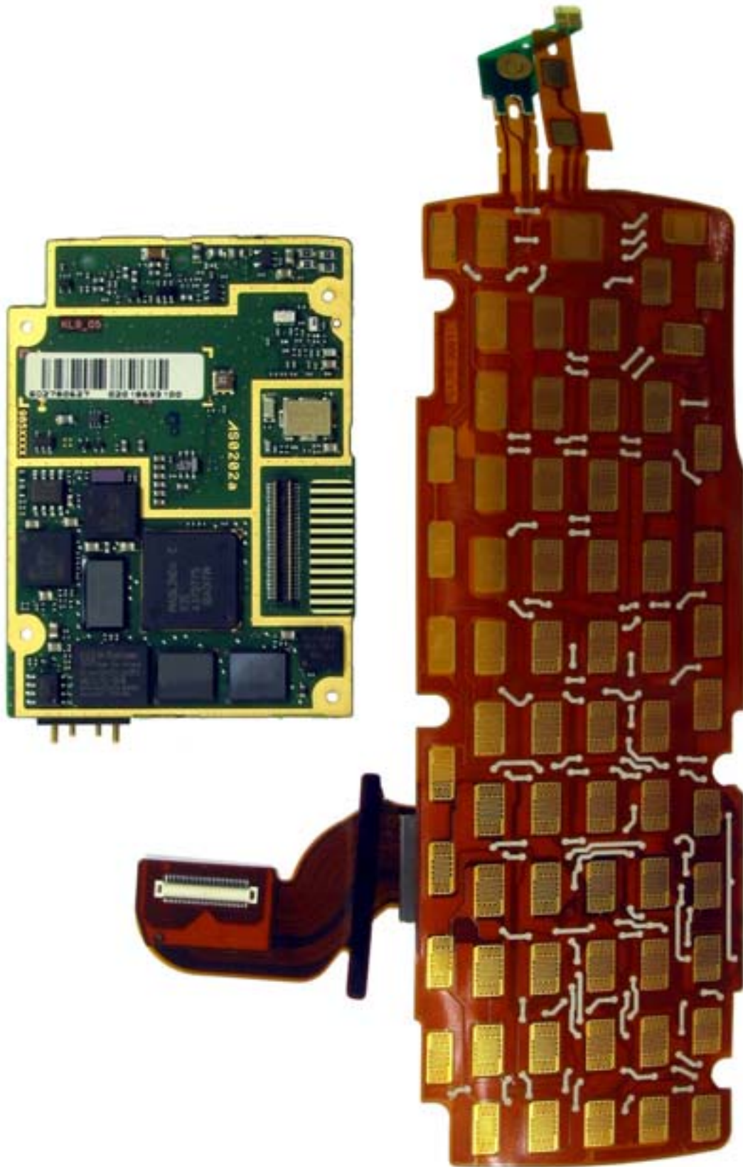
Exhibit 9: Internal Photographs
