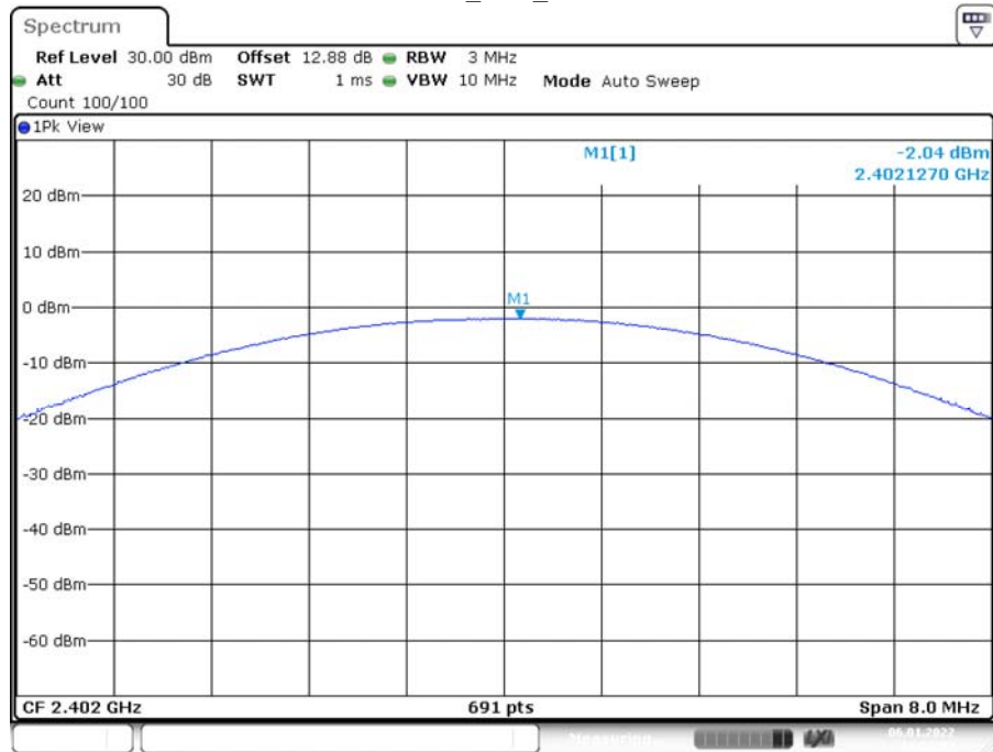
2DH1_Ant1_2402
