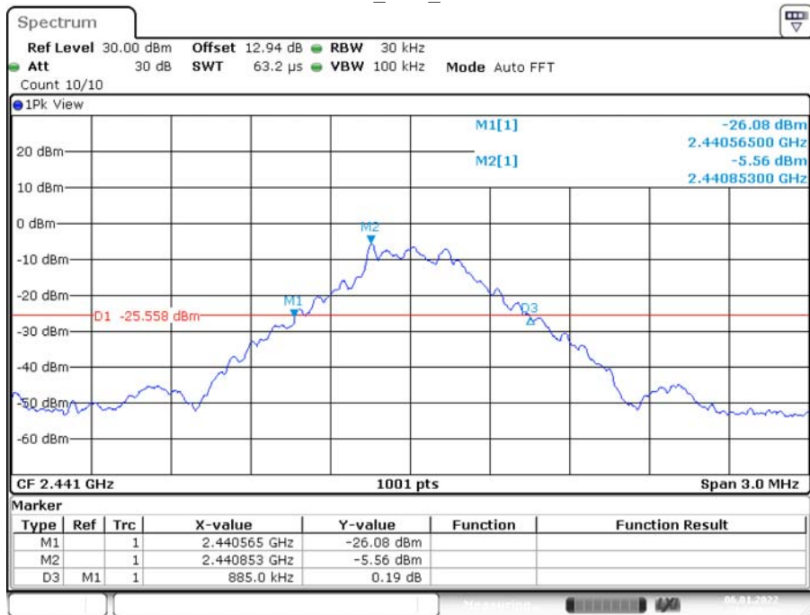
DH1_Ant1_2441
