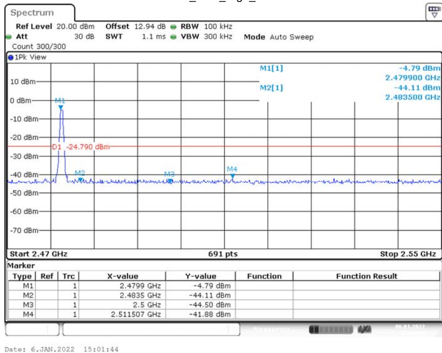
DH1_Ant1_High_2480
