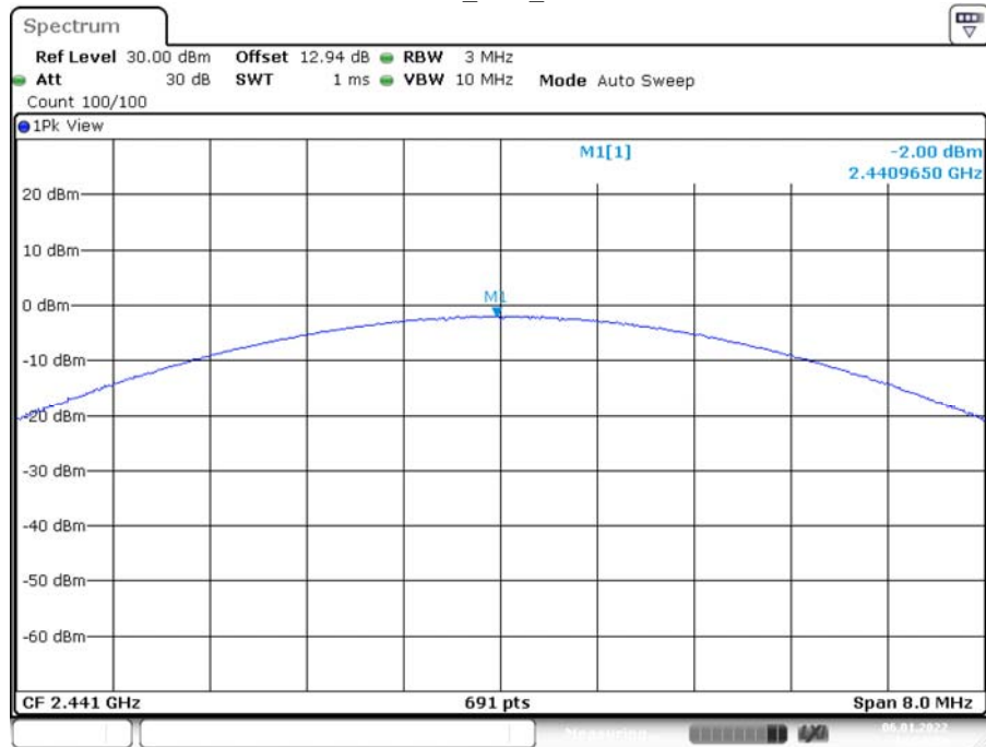
3DH1_Ant1_2441
