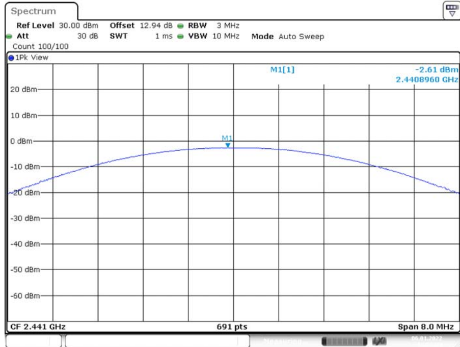
2DH1_Ant1_2441
