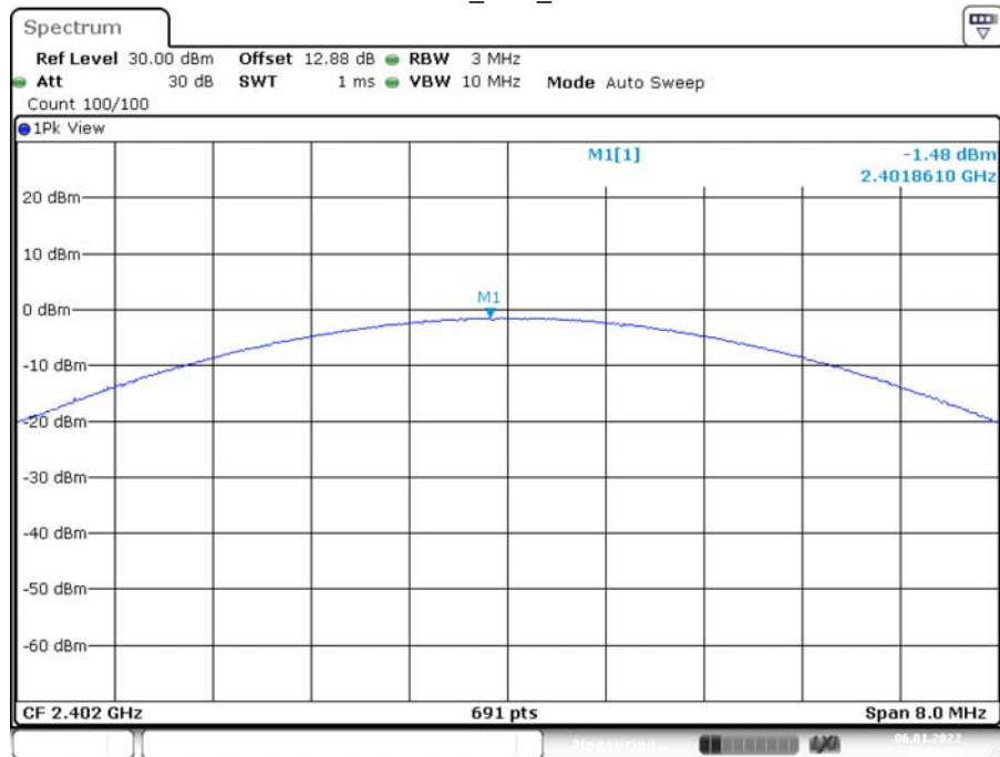
3DH1_Ant1_2402
