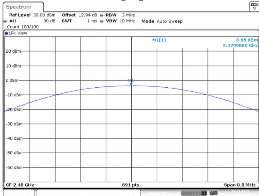
2DH1_Ant1_2480
