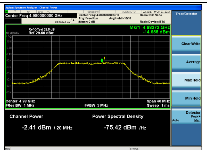
Chain 2 Peak Output Power (25dBi Antenna) - 4980MHz
