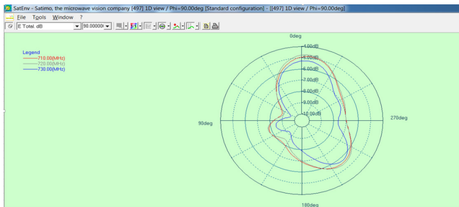
LTE B12/B17/B28Phi=90deg
